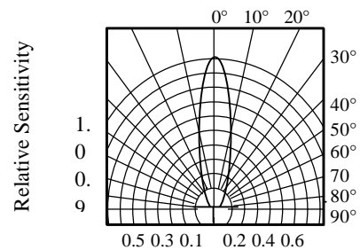
FIG.6 SENSITIVITY DIAGRAM
