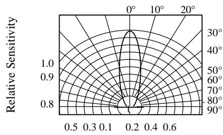
FIG.6 SENSITIVITY DIAGRAM
