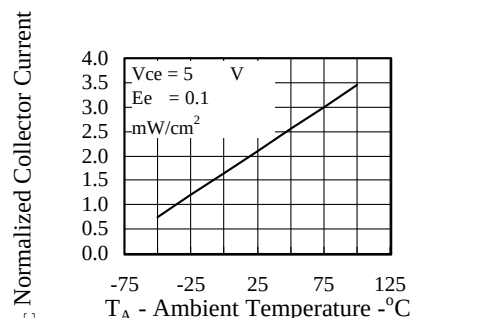
FIG.2 NORMALIZED COLLECTOR CURRENT VS AMBIENT TEMPERATURE
