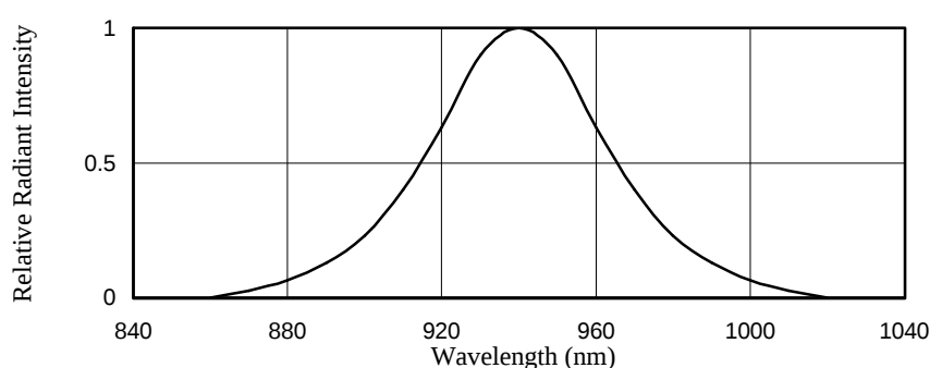
FIG.1 SPECTRAL DISTRIBUTION
