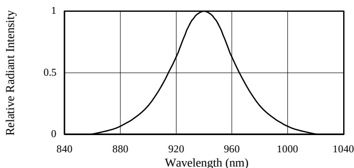
FIG.1 SPECTRAL DISTRIBUTION
