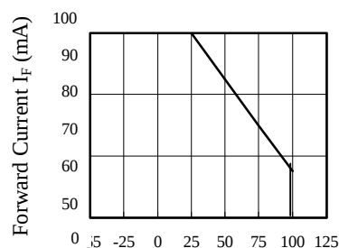
FIG.2 FORWARD CURRENT VS. AMBIENT TEMPERATURE
