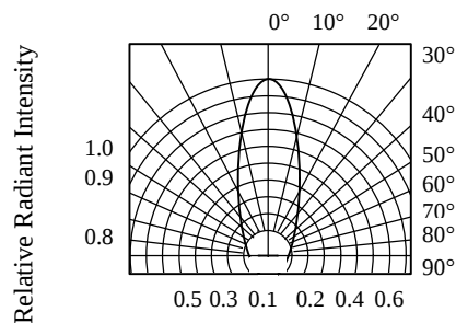
FIG.5 RADIATION DIAGRAM
