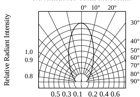
FIG.6 RADIATION DIAGRAM
