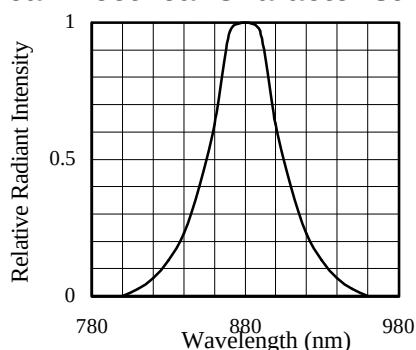
FIG.1 SPECTRAL DISTRIBUTION
