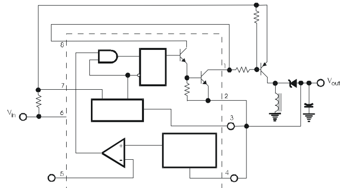
Figure 6b. External PNP Saturated Switch.
