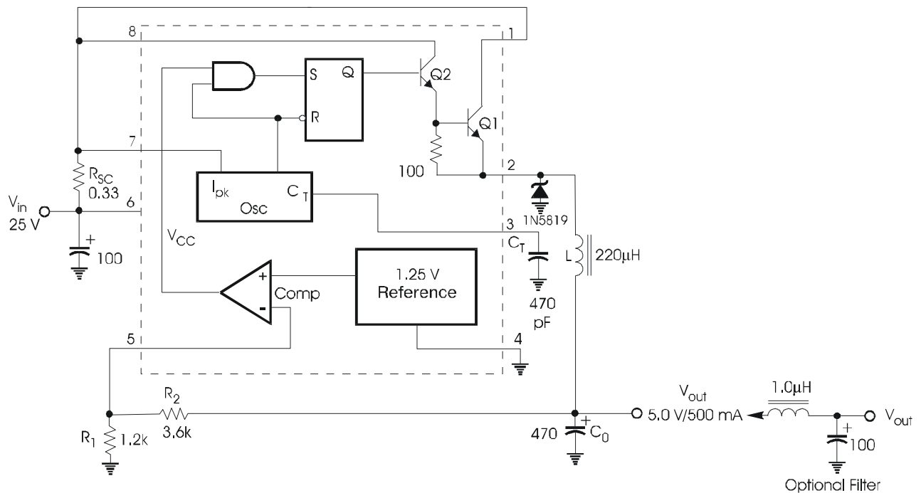
Figure 3. Step-Down Converter.
