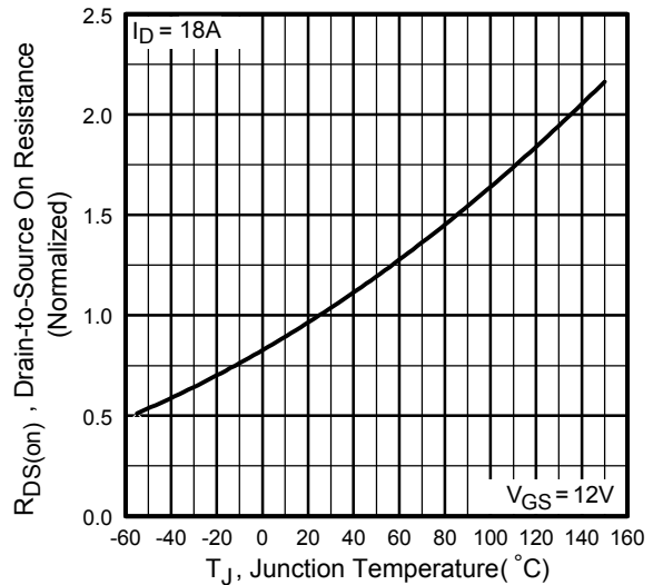
Fig 4. Normalized On-Resistance
