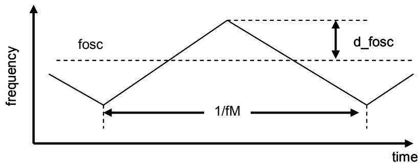
【Figure 7: d_{fosc} , f_M measurement】
