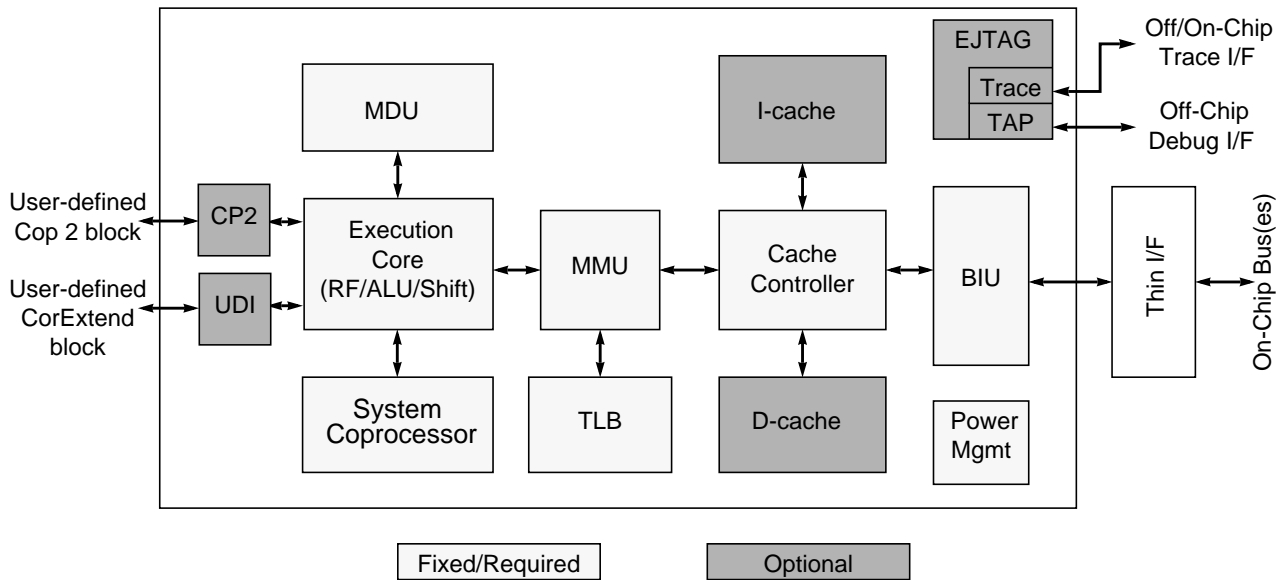
Figure 1 4KEc Core Block Diagram
