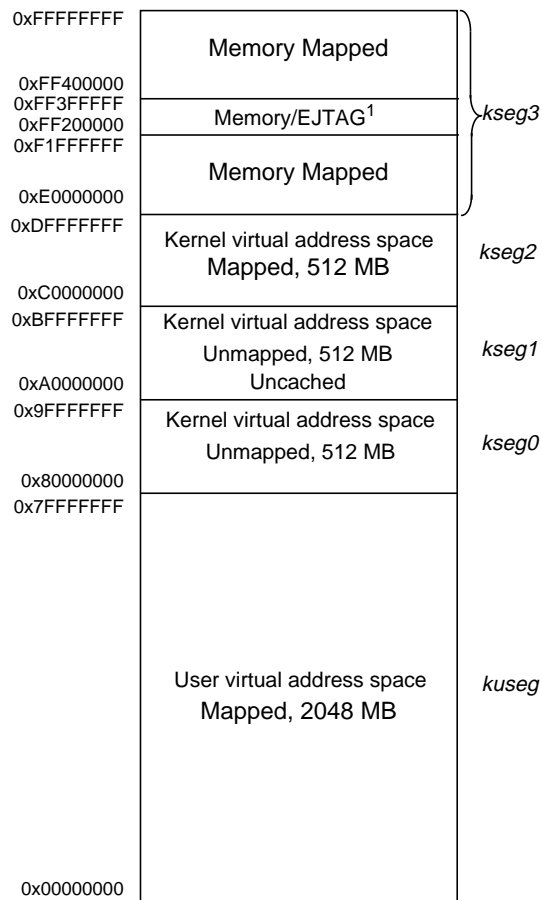
Figure 3 4KEc Core Virtual Address Map
