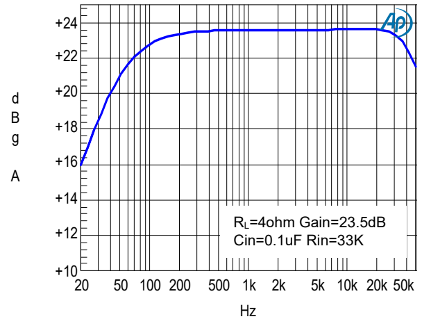
Frequency Response
