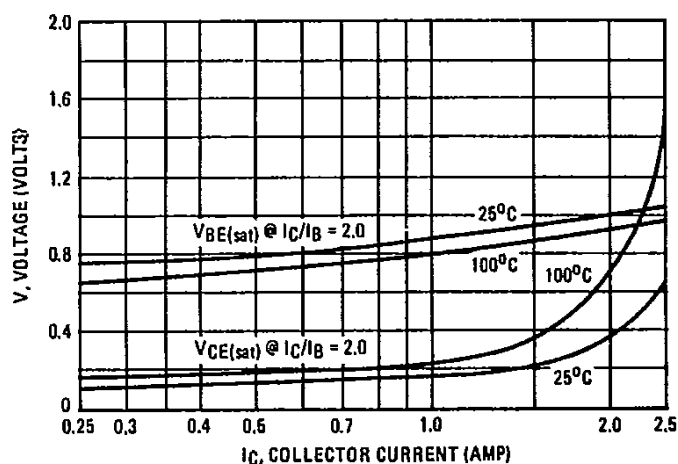
FIGURE 13 – "ON" VOLTAGES
