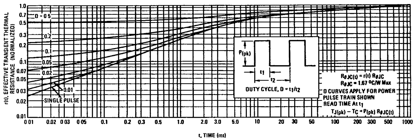
FIGURE 10 – THERMAL RESPONSE
