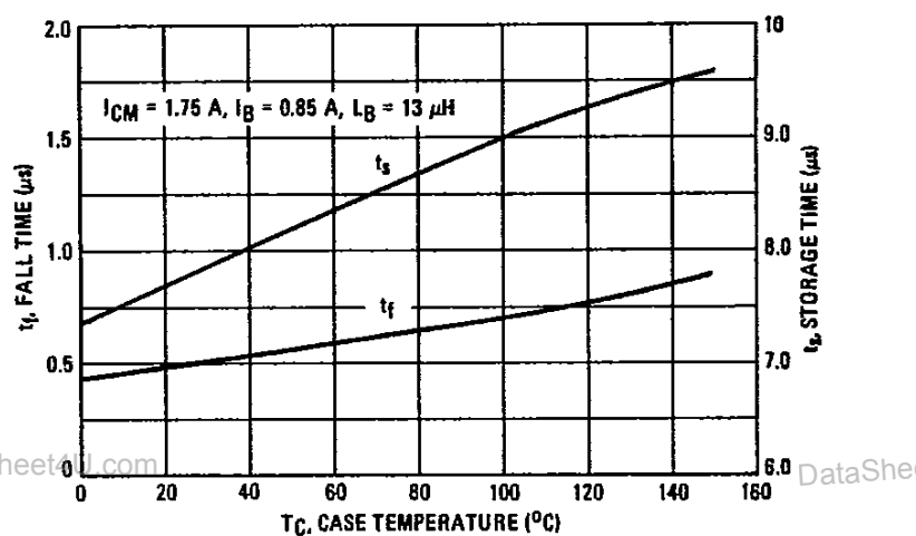
FIGURE 7 – SWITCHING BEHAVIOR versus TEMPERATURE
