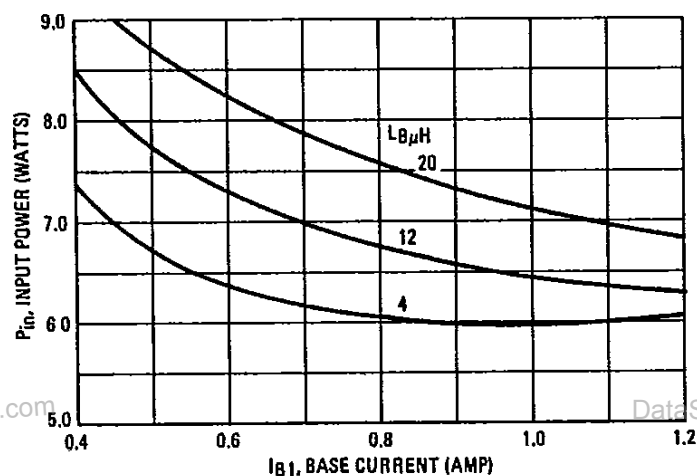
FIGURE 6 – OPTIMIZING DRIVE @ I_C = 2.0 A
