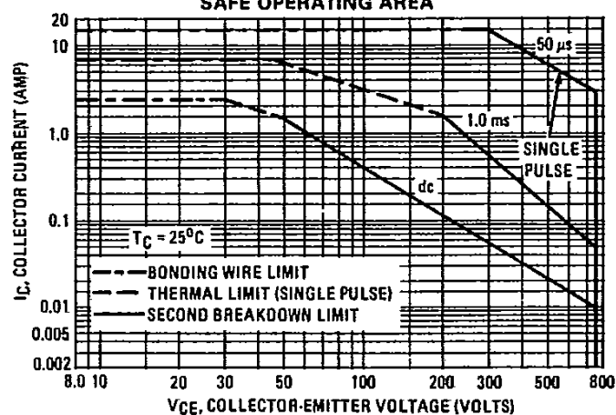
FIGURE 14-MAXIMUM FORWARD BIAS SAFE OPERATING AREA
