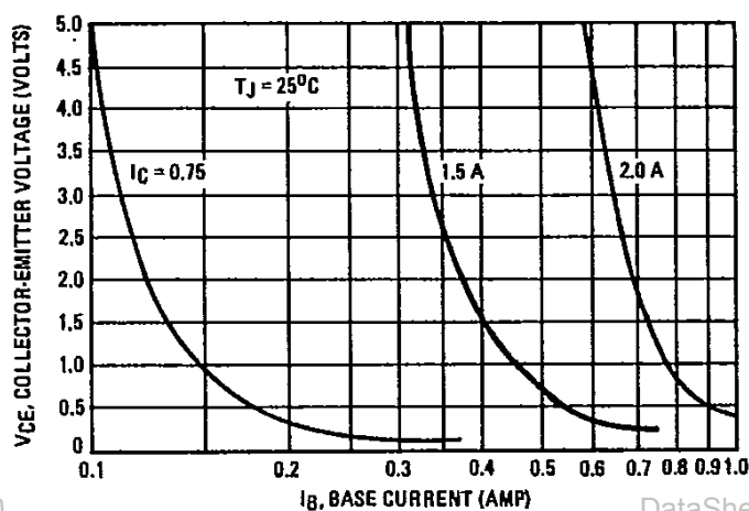
FIGURE 11 – COLLECTOR SATURATION REGION
