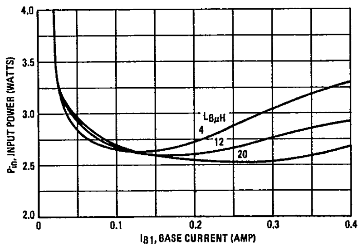
FIGURE 4 – OPTIMIZING DRIVE @ I_C = 0.75 A
