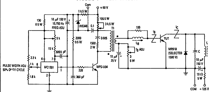
FIGURE 1 — TEST CIRCUIT
