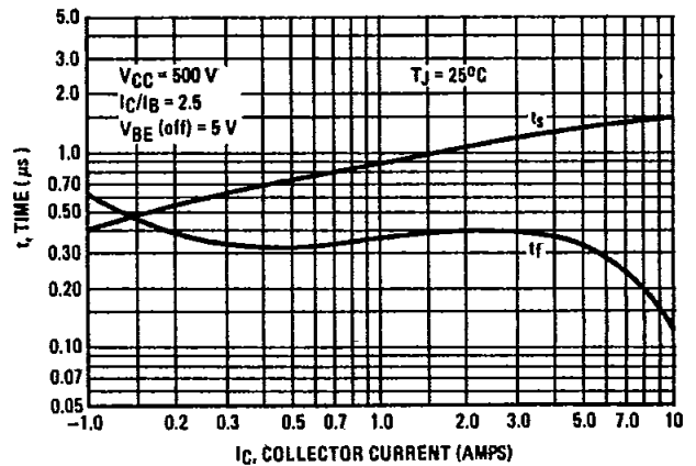
FIGURE 10 – TURN-OFF SWITCHING TIMES
