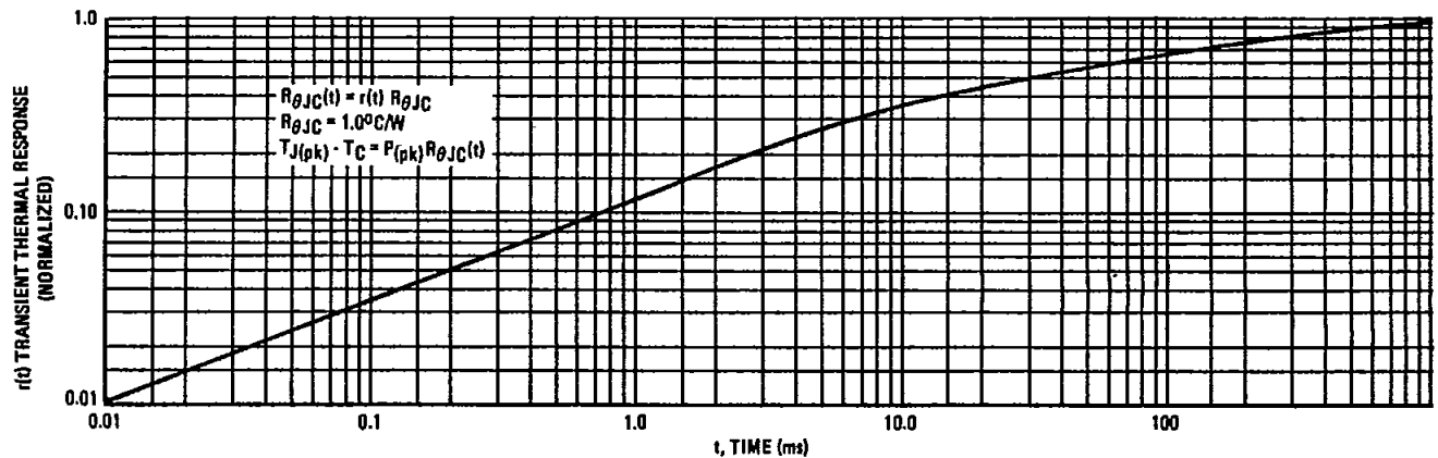
FIGURE 11 – THERMAL RESPONSE
