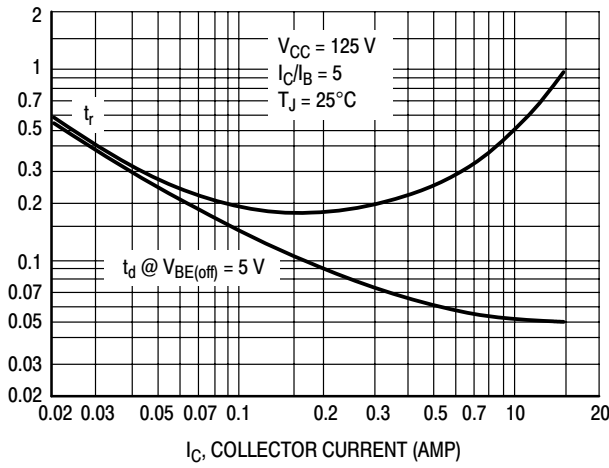
Figure 8. Turn-On Time
