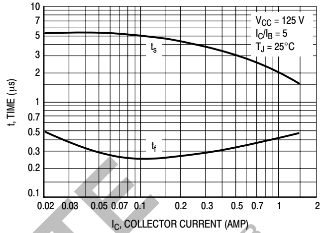
Figure 9. Turn-Off Time
