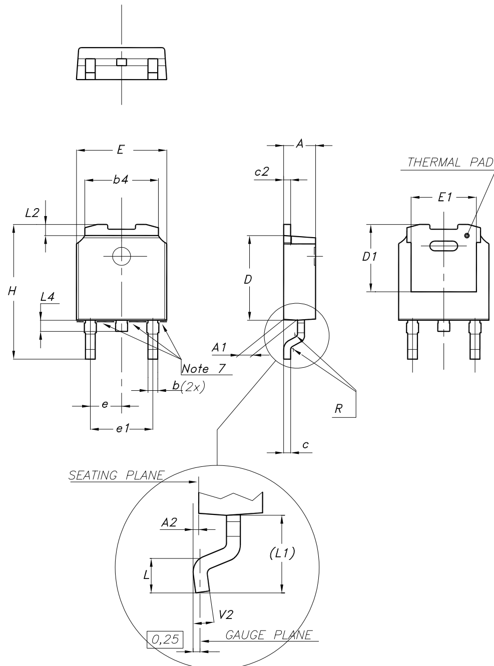
Figure 10. DPAK (TO-252) type A package outline
