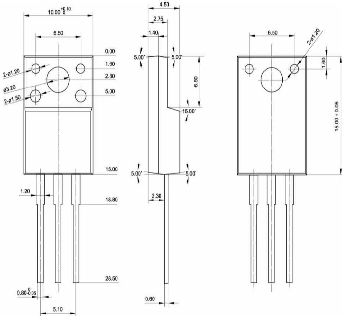
Fig.2 Outline dimensions
