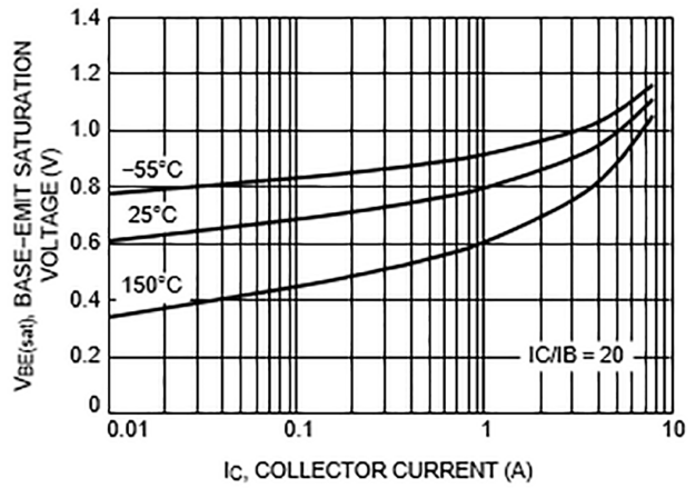
Figure 4. Saturation Voltage V_{BE(sat)}
