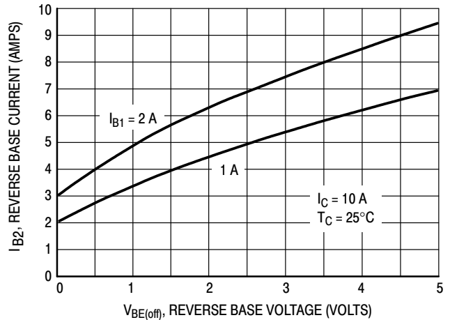
Figure 13. Peak Reverse Base Current
