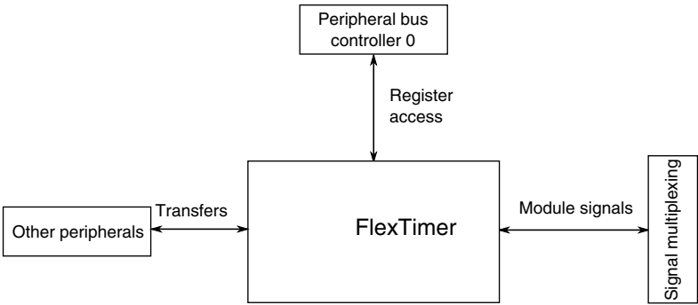
Figure 3-33. FlexTimer configuration
