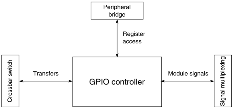
Figure 3-44. GPIO configuration
