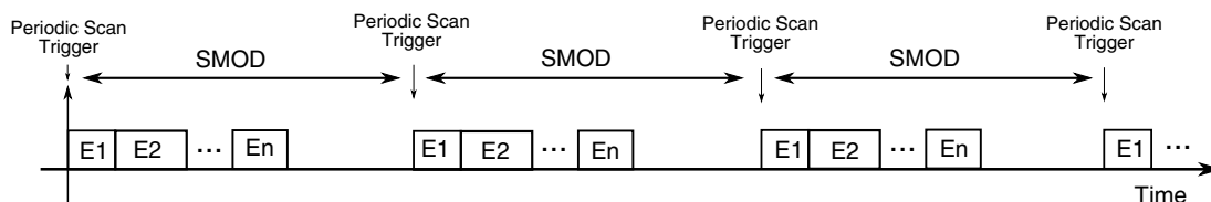
Figure 44-40. Periodical Scan Time Chart
