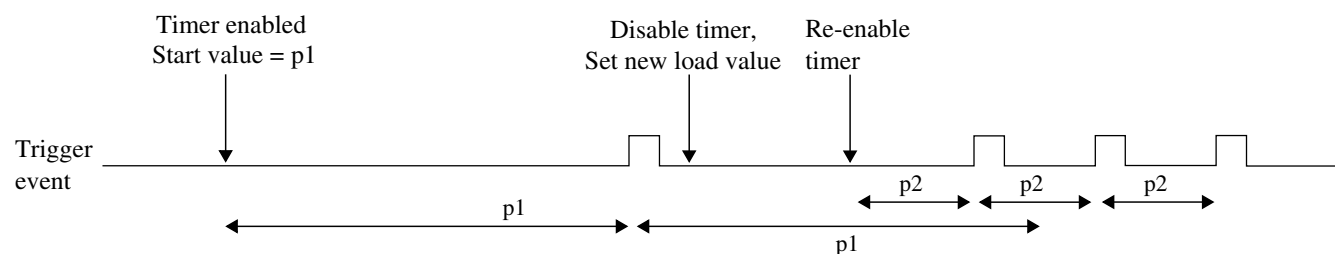
Figure 35-24. Modifying running timer period
