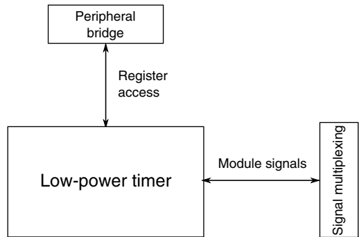
Figure 3-36. LPT configuration
