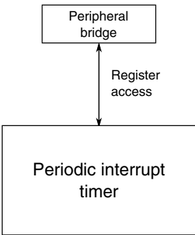
Figure 3-35. PIT configuration
