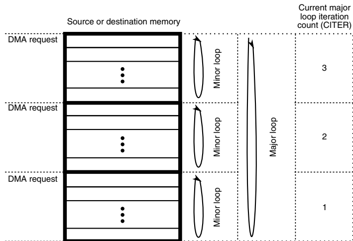
Figure 21-101. Example of multiple loop iterations
