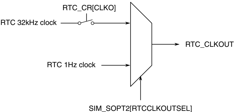
Figure 3-39. RTC_CLKOUT generation
