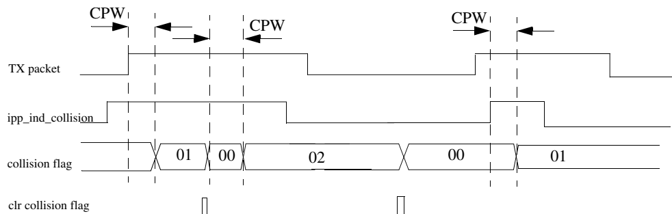
Figure 41-197. Collision pulse detection
