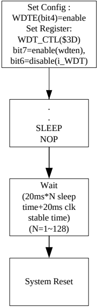
WDT-Wakeup : (Watch-dog timer wake-up)
