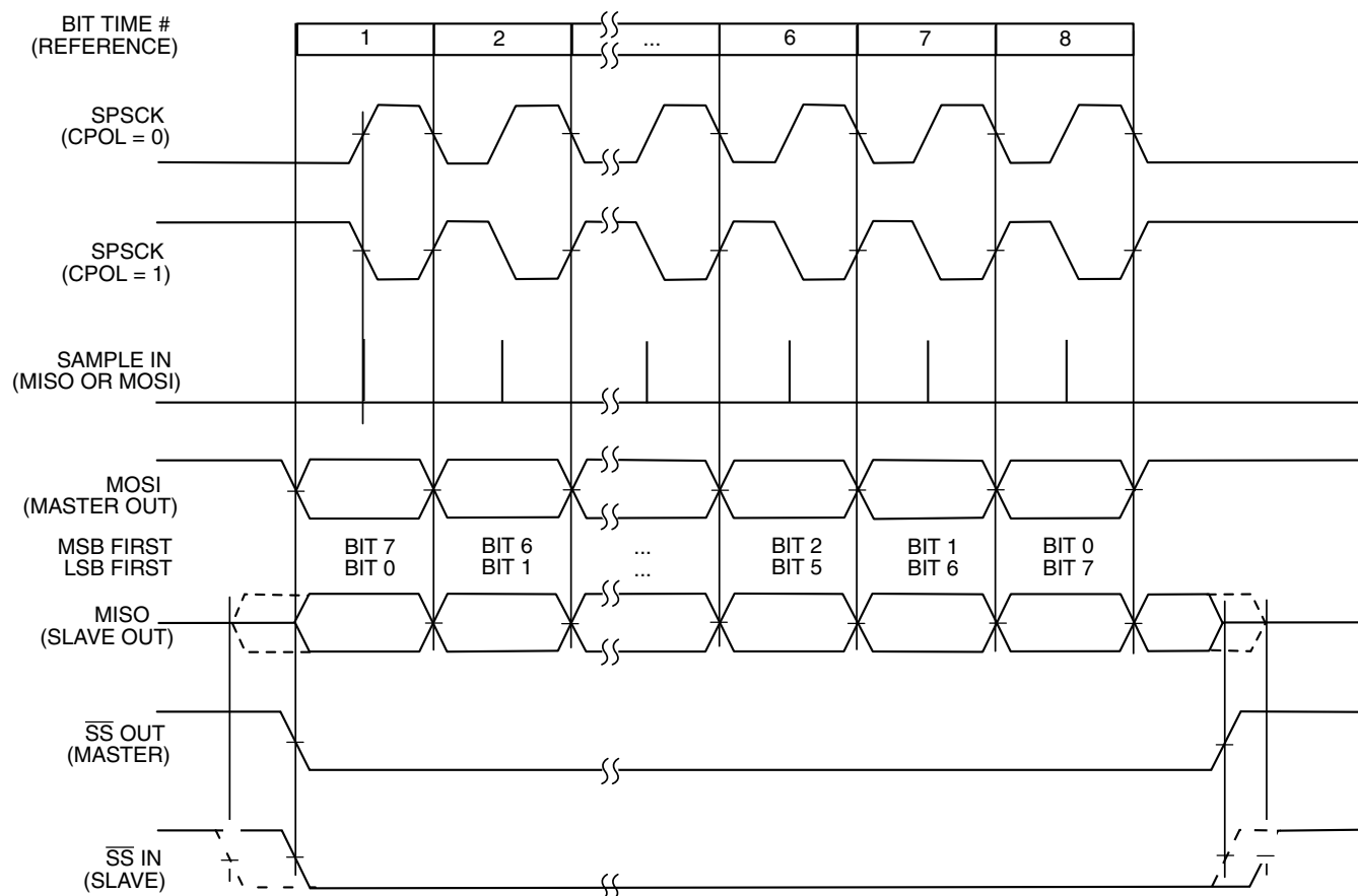
Figure 29-22. SPI clock formats (CPHA = 0)
