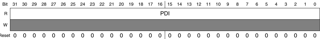
FGPIOx_PDIR field descriptions
