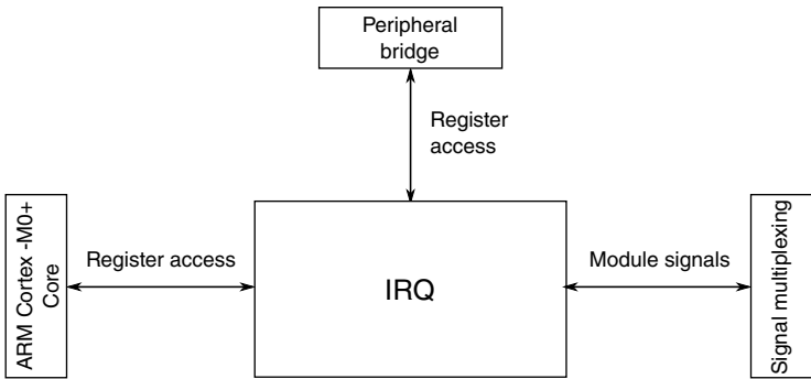
Figure 3-32. IRQ configuration
