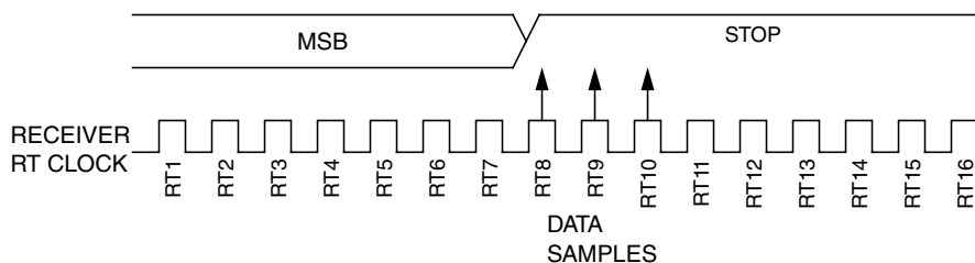
Figure 31-36. Slow data
