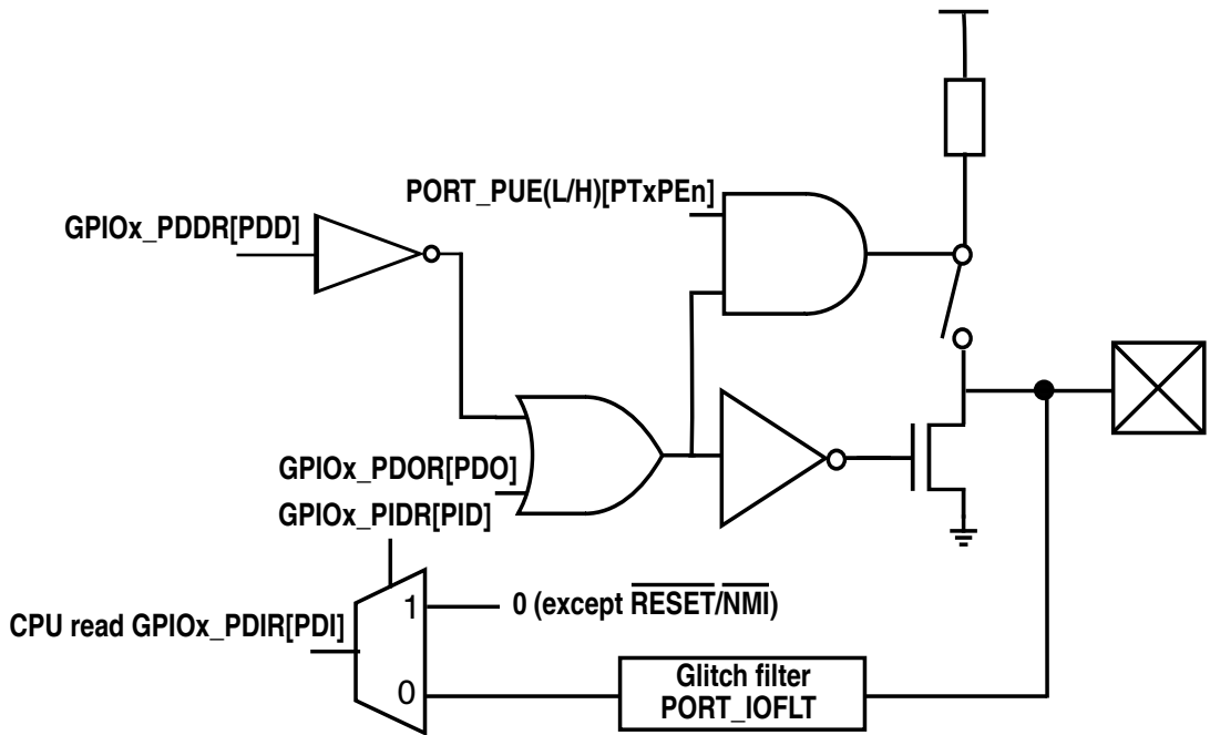
Figure 11-2. SDA(PTA2)/SCL(PTA3) structure
