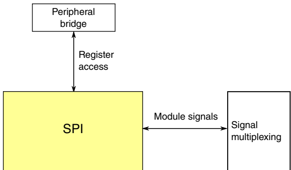
Figure 3-27. SPI configuration
