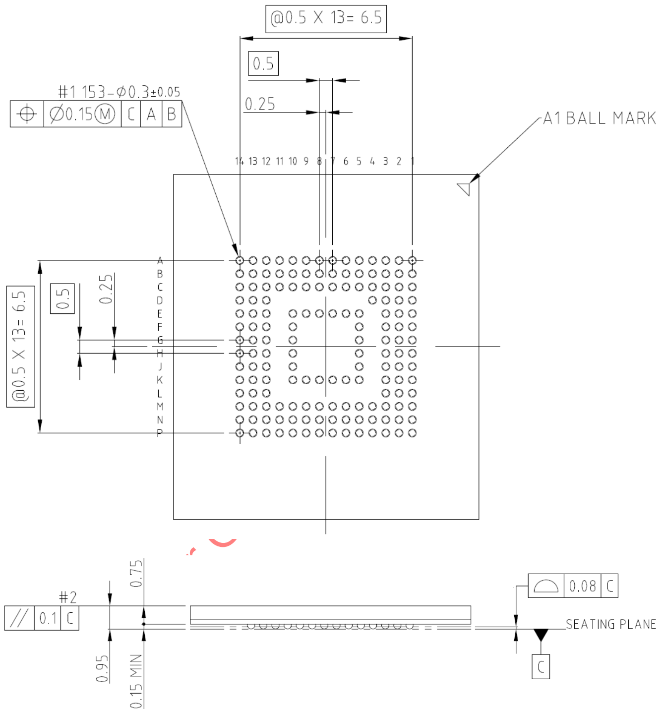
Figure 5 – 11.5 x 13.0 x 1.0mm Bottom &amp; side View
