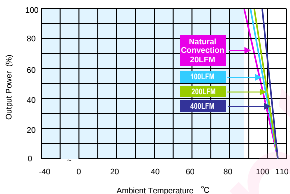
MKZI10-24S15, MKZI10-48S12, MKZI10-48S15 Derating Curve without Heatsink
