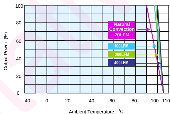
MKZI10-24S15, MKZI10-48S12, MKZI10-48S15 Derating Curve with Heatsink
