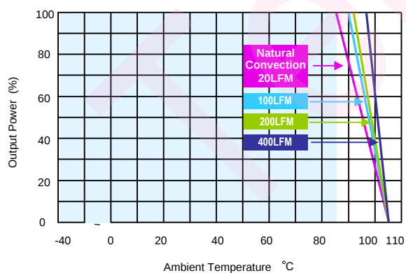
MKZI10-24S12, MKZI10-48S24 Derating Curve without Heatsink
