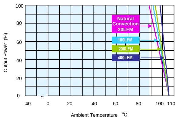
MKZI10-24S24 Derating Curve without Heatsink
