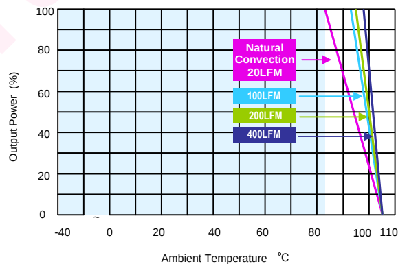
MKZI10-110S05 Derating Curve with Heatsink
