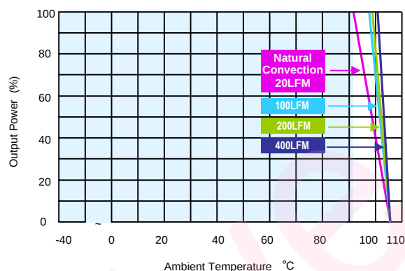
MKZI10-24S24 Derating Curve with Heatsink
