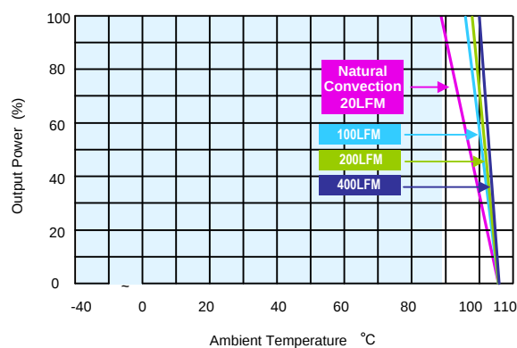
MKZI10-24S12, MKZI10-48S24 Derating Curve with Heatsink
