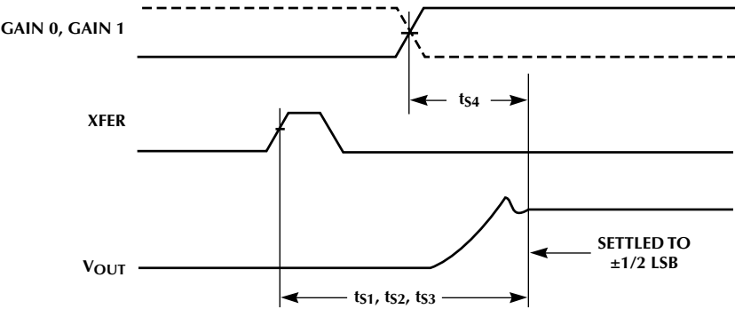
Figure 2. Settling Time
