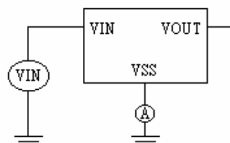
Test Circuit 2
