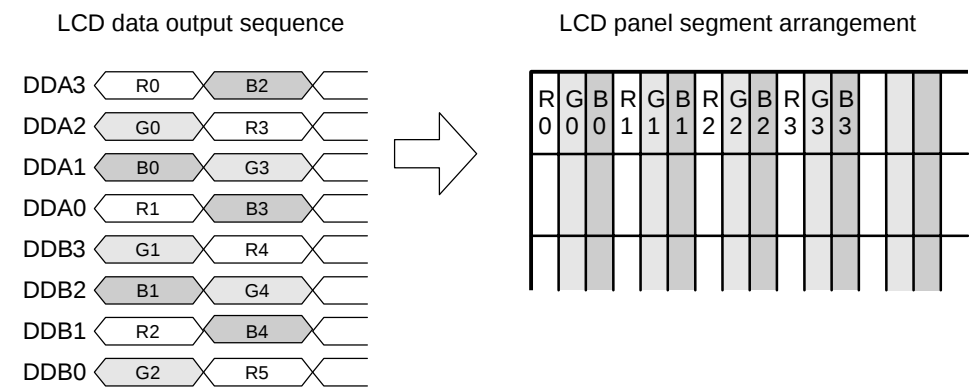
Fig. F3.2.2 Color STN, 8-bit mode
