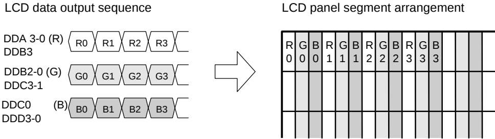
Fig. F3.2.8 Color TFT, 16-bit mode
