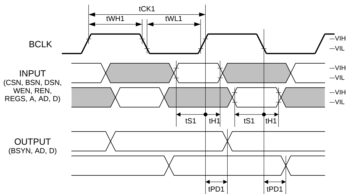
(a) Host interface
