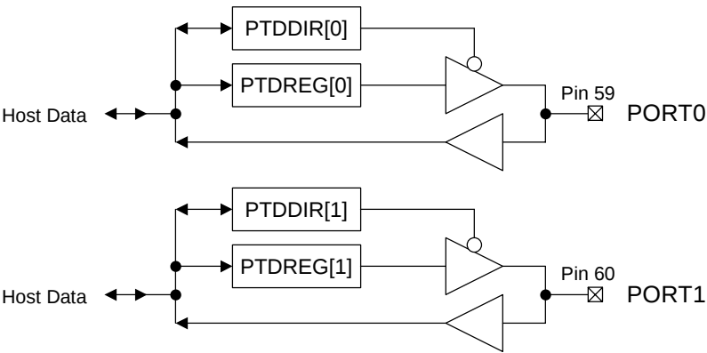
Fig. F4.1 General purpose ports
