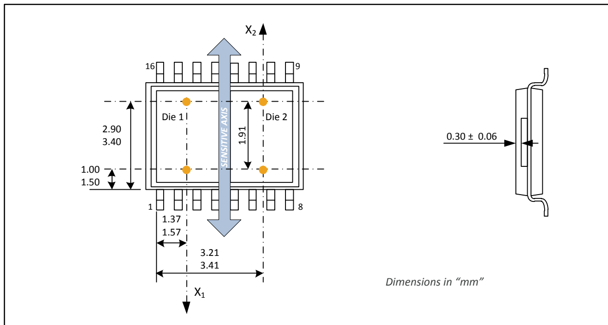
fig. 35 - TSSOP-16 - Sensitive Spot Location for Linear Stray-field Immune
