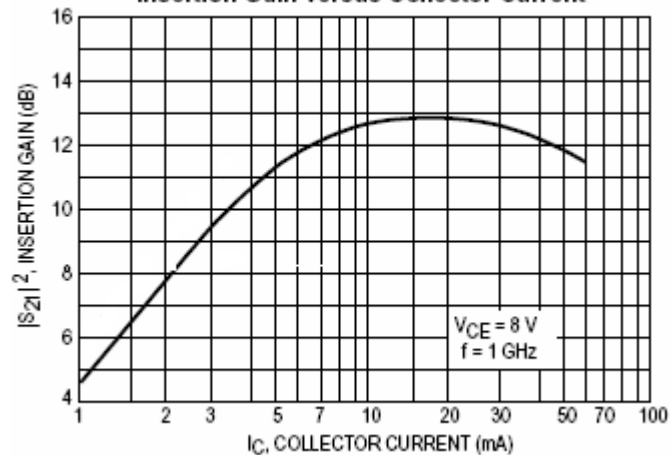
Insertion Gain versus Collector Current
