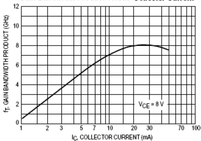
Gain Bandwidth Product versus Collector Current
