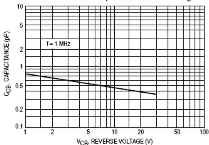
Collector-Base Capacitance versus Voltage
