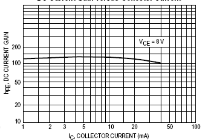
DC Current Gain versus Collector Current
