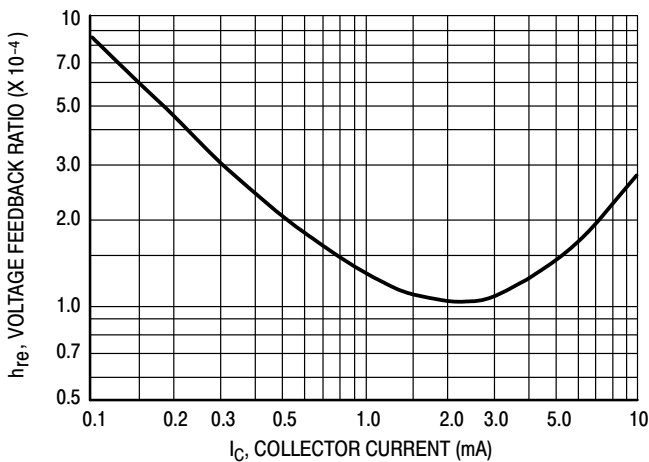
Figure 15. Voltage Feedback Ratio
