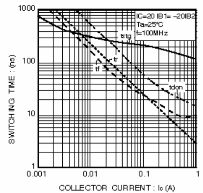
Fig.6 Switching time
