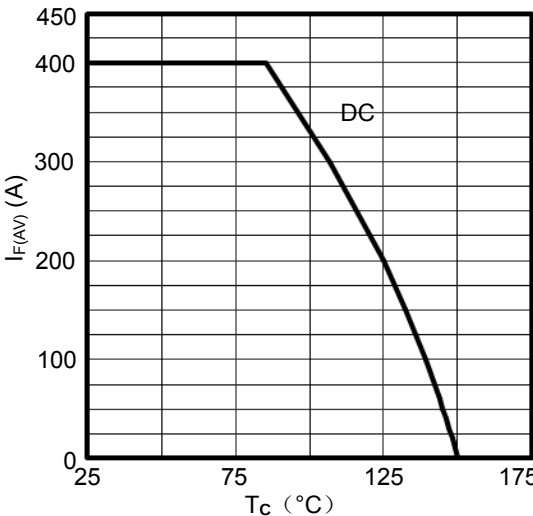
Figure4. Forward current vs.Case temperature
