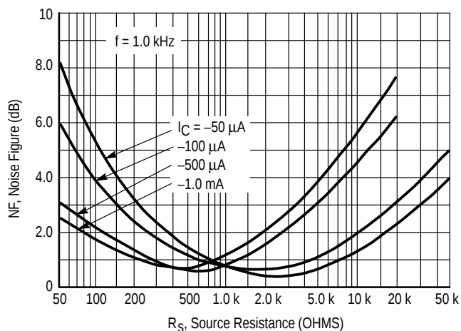
Figure 18. Source Resistance Effects
