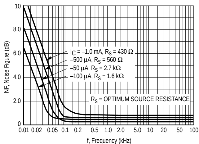
Figure 17. Frequency Effects
