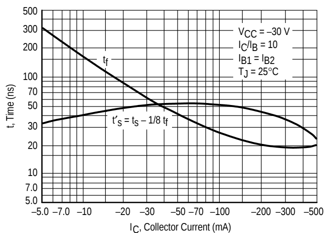
Figure 16. Turn-Off Time
