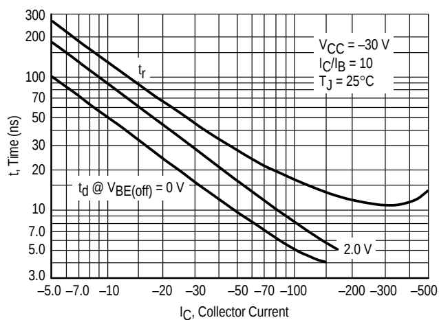
Figure 15. Turn-On Time
