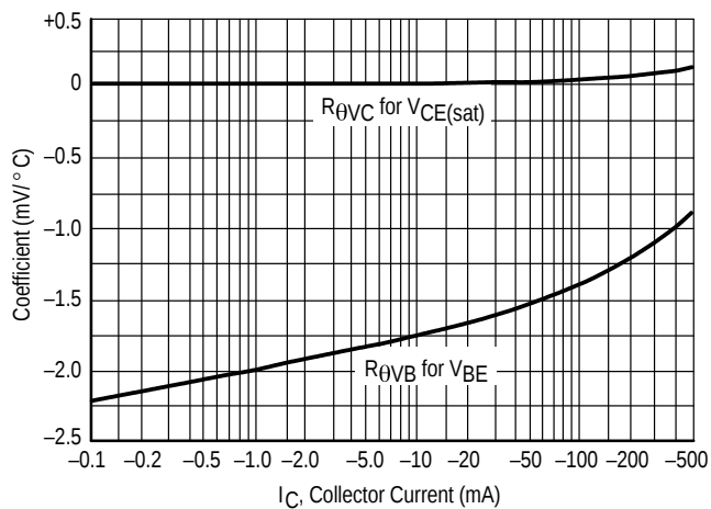
Figure 22. Temperature Coefficients
