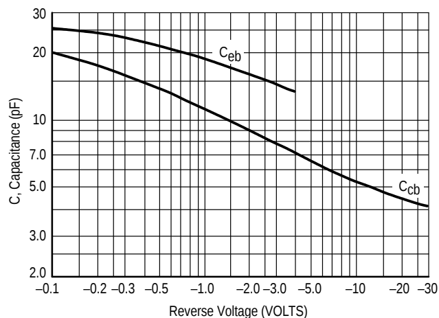
Figure 19. Capacitances
