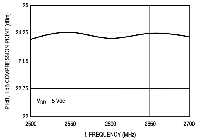
Figure 26. P1dB versus Frequency
