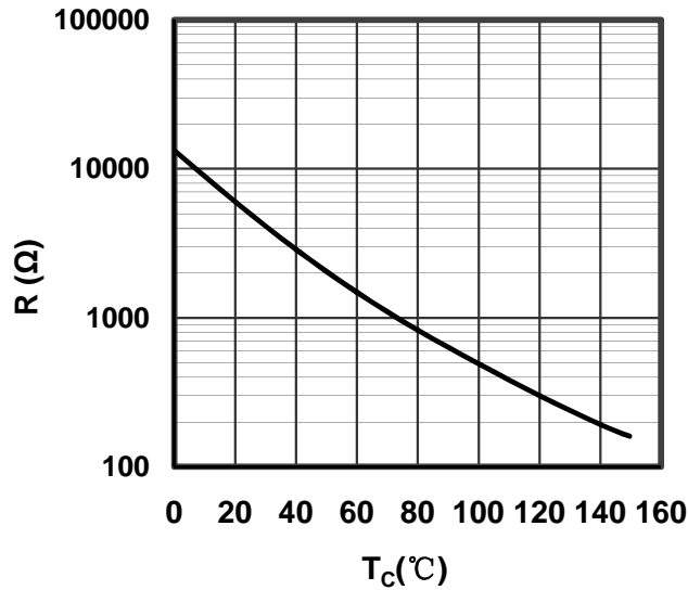
Figure 13. NTC Characteristics
