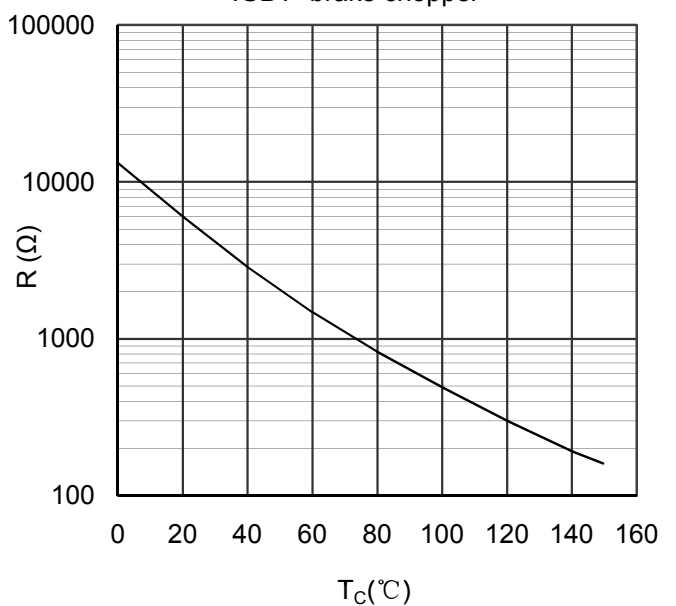
Figure 14. NTC Characteristics
