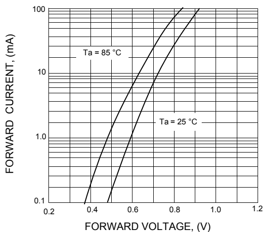
FIG.3 - FORWARD CHARACTERISTICS
