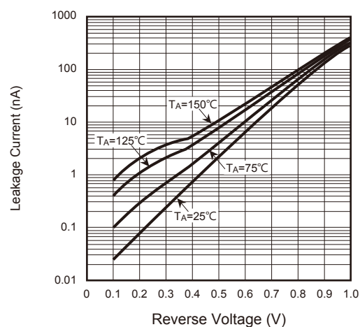
Fig.4 - V_R - I_R Characteristics
