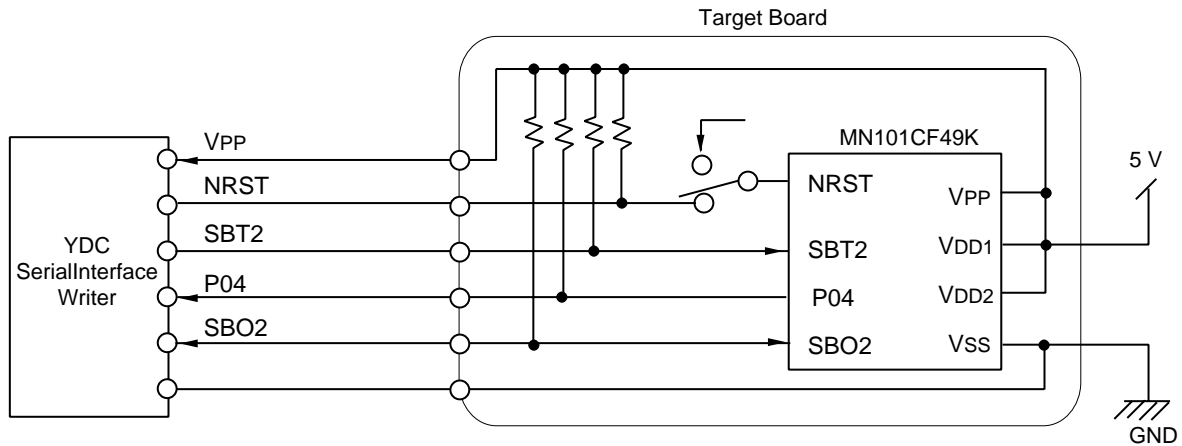
Figure 20-6-2 Target Board for programming with the clock synchronous communication using Serial writer
