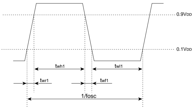
Figure 20-3-3 OSC1 Timing Chart
