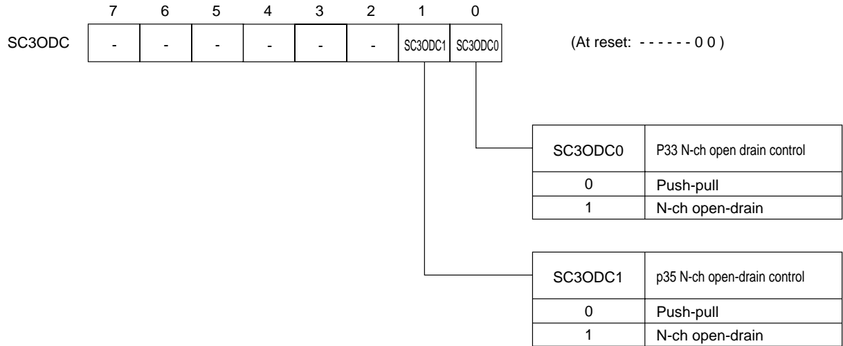
Figure 14-2-5 Serial Interface 3 Port Control Register (SC3ODC : x'03FAE', R/W)
