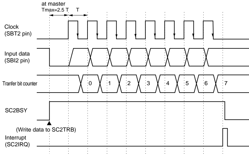
Figure 13-3-8 Reception Timing (Falling edge, Start condition is enabled)
