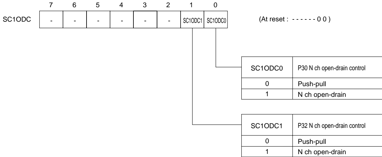
Figure 12-2-7 Serial Interface 1 Port Control Register (SC1ODC : x'03F9E', R/W)
