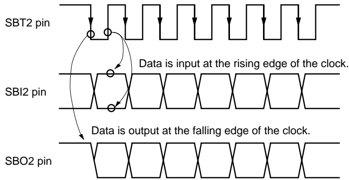
Figure 13-3-10 Transmission / Reception Timing (Reception : Rising edge, Transmission : Falling edge)
