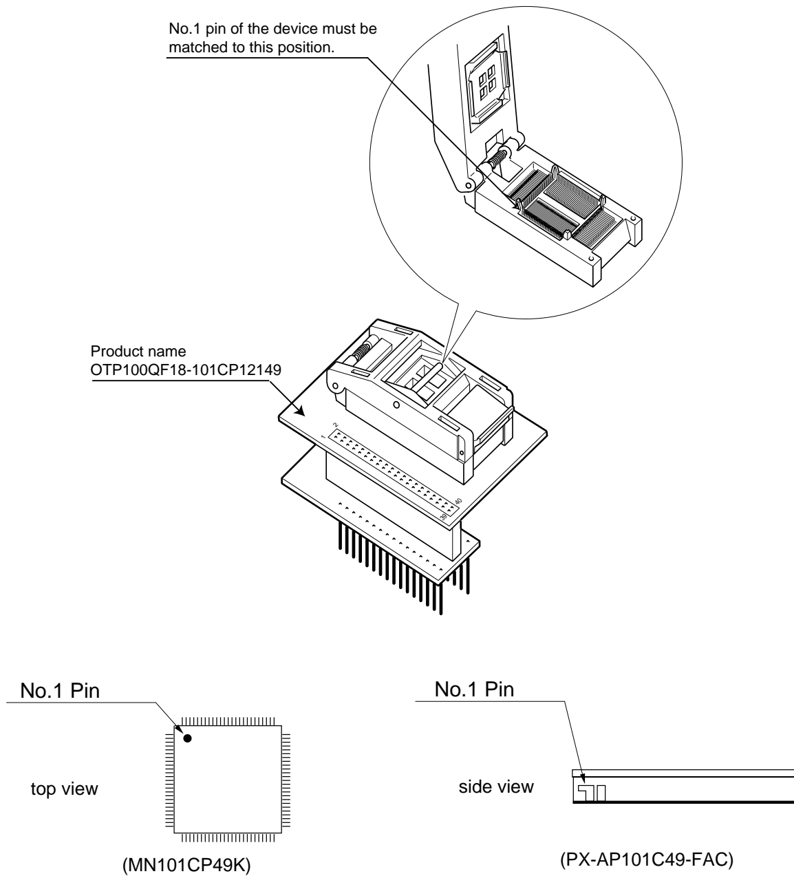
Figure 19-1-1 Mounting a Device in Programming Adapter and the Position of No.1 Pin
