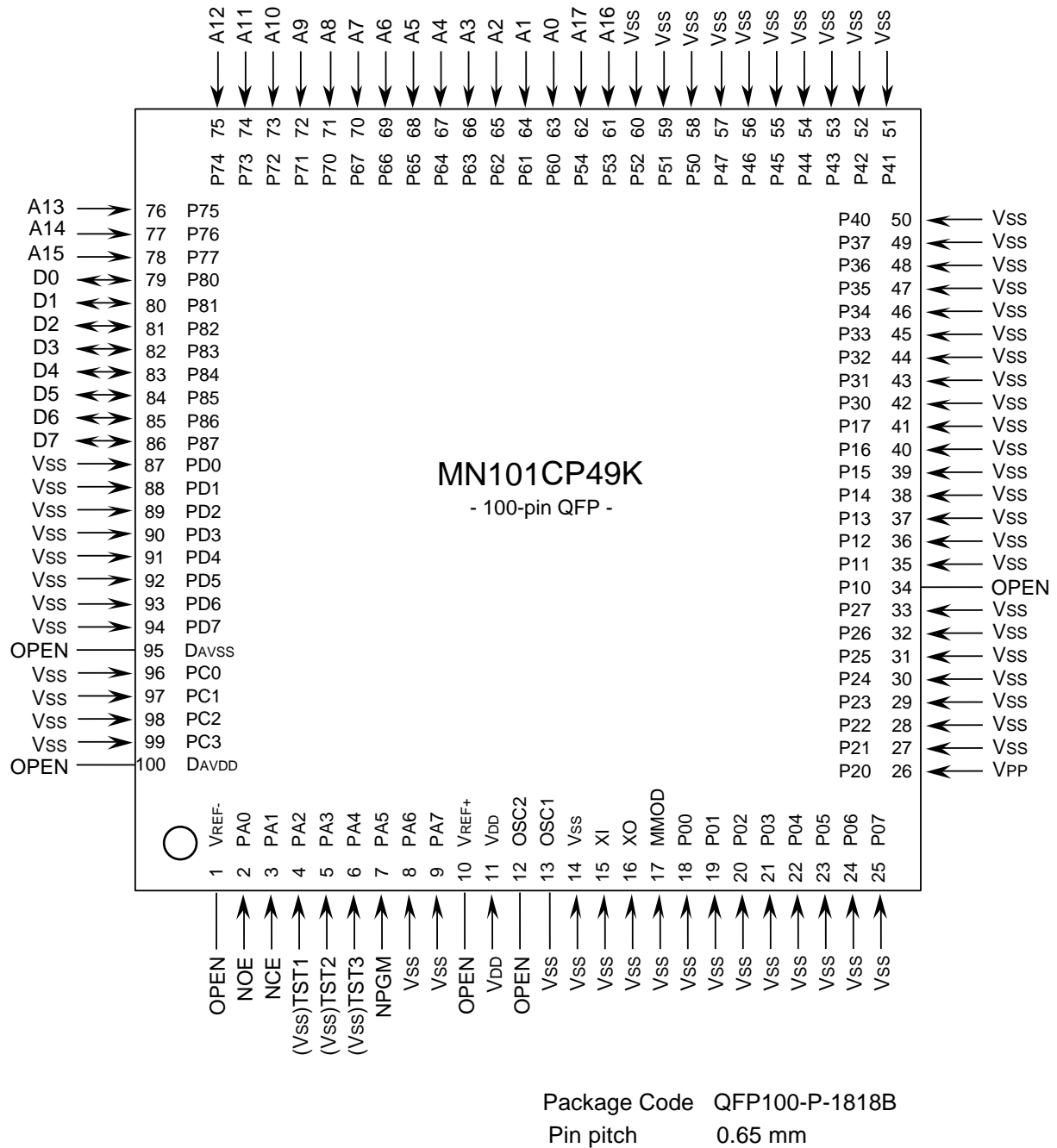
Figure 19-1-2 MN101CP49KAF EPROM Programming Adapter Connection
