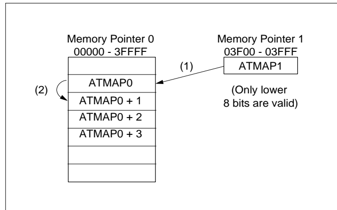
Figure 15-3-5 Transfer Mode 3
