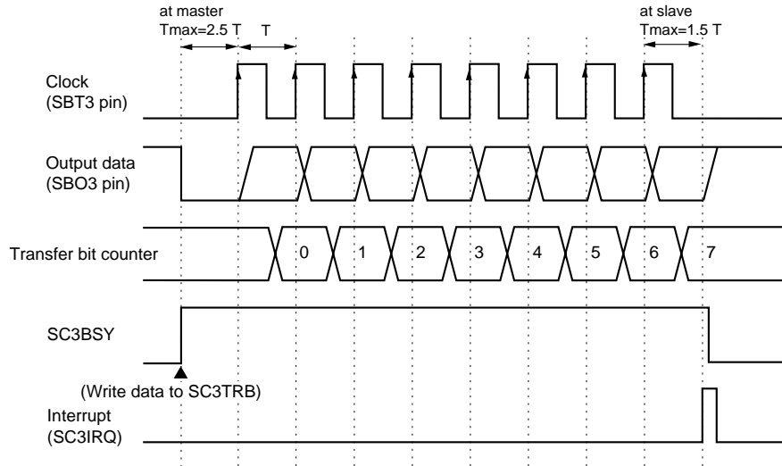
Figure 14-3-4 Transmission Timing (Rising edge, Enable Start Condition)
