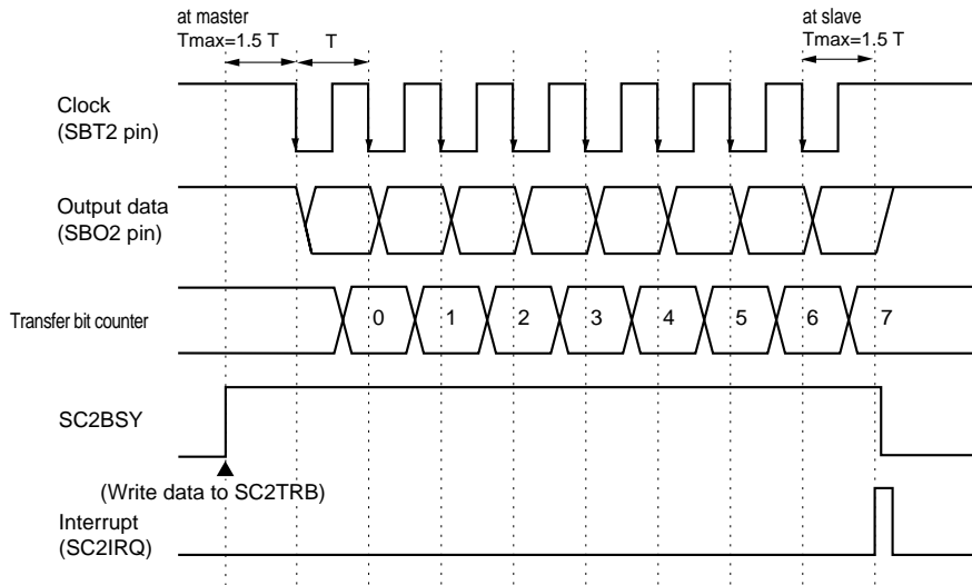
Figure 13-3-3 Transmission Timing (Falling edge, Start condition is disabled)
