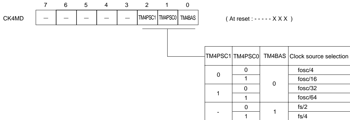
Figure 5-2-6 Timer 4 Prescaler Selection Register (CK4MD : x'03F66', R/W)
