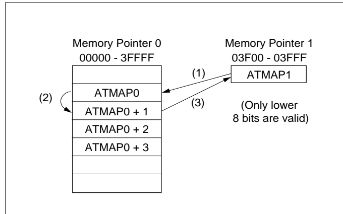
Figure 15-3-9 Transfer Mode 7
