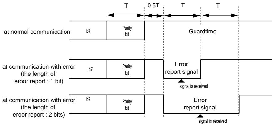
Figure 12-3-20 Report Timing of Communication Error Signal
