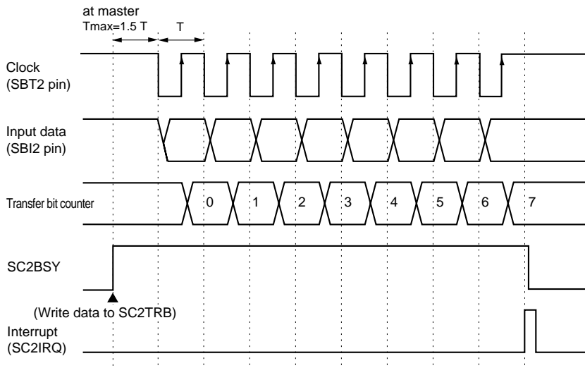
Figure 13-3-7 Reception Timing (Rising edge, Start condition is disabled)
