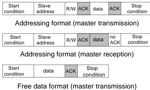
Figure 14-3-15 Communication Sequence on Each Transfer Format
