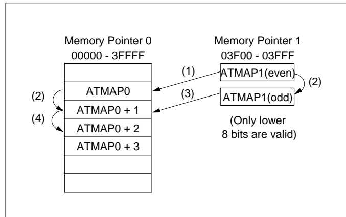
Figure 15-3-7 Transfer Mode 5
