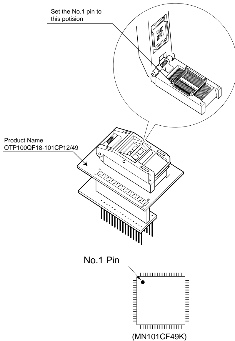
Figure 20-5-1 Fixing a Device on the Adapter Socket and the Position of No.1 Pin
