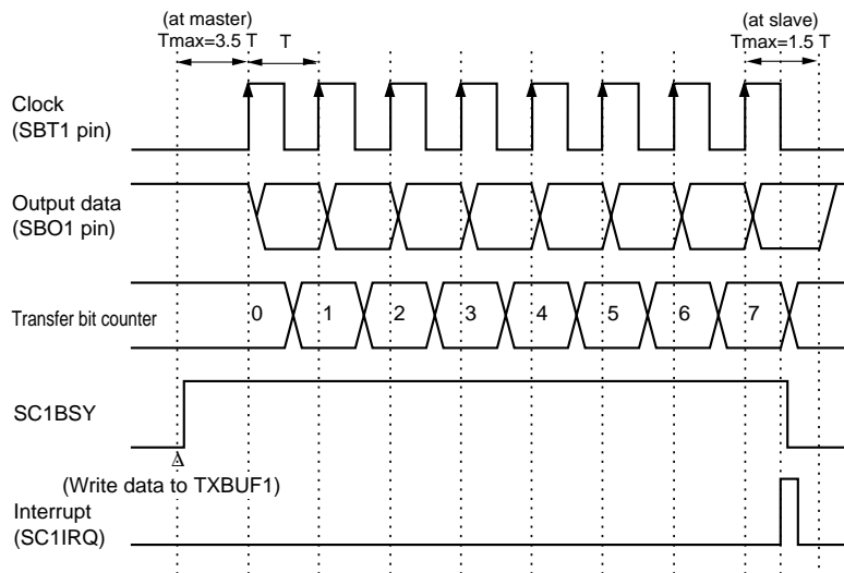
Figure 12-3-7 Transmission Timing (rising edge, start condition is disabled)
