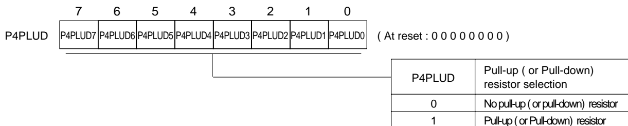
Port 4 pull-up / pull-down resistor control register (P4PLUD : x'03F44', R/W)
