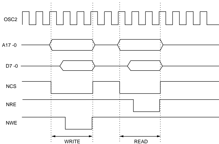
Figure 2-3-5 ROM and RAM Access Timing with 1 Wait Cycle
