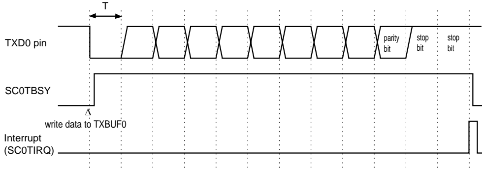
Figure 11-3-20 Transmission Timing (parity bit is enabled)
