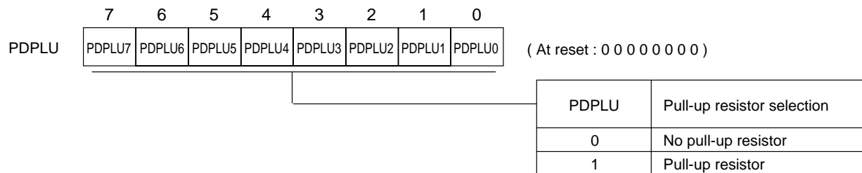
Port D pull-up resistor control register (PDPLU : x'03F4D', R/W)
