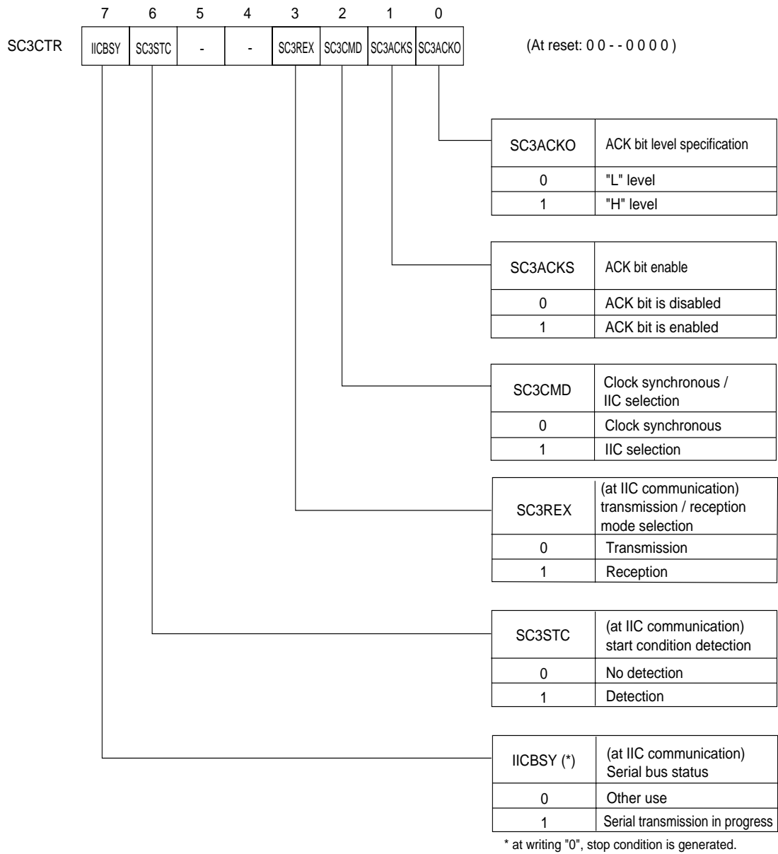
Figure 14-2-4 Serial Interface 3 Control Register (SC3CTR : x'03FAA', R/W)
