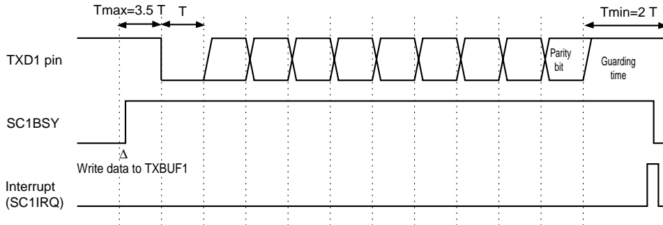
Figure 12-3-22 Transmission Timing (ATR Data, T=0, 1 Data Communication)
