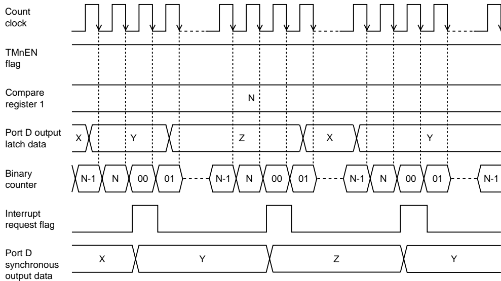
Figure 6-7-1 Count Timing of Synchronous Output (Timer 1, Timer2)
