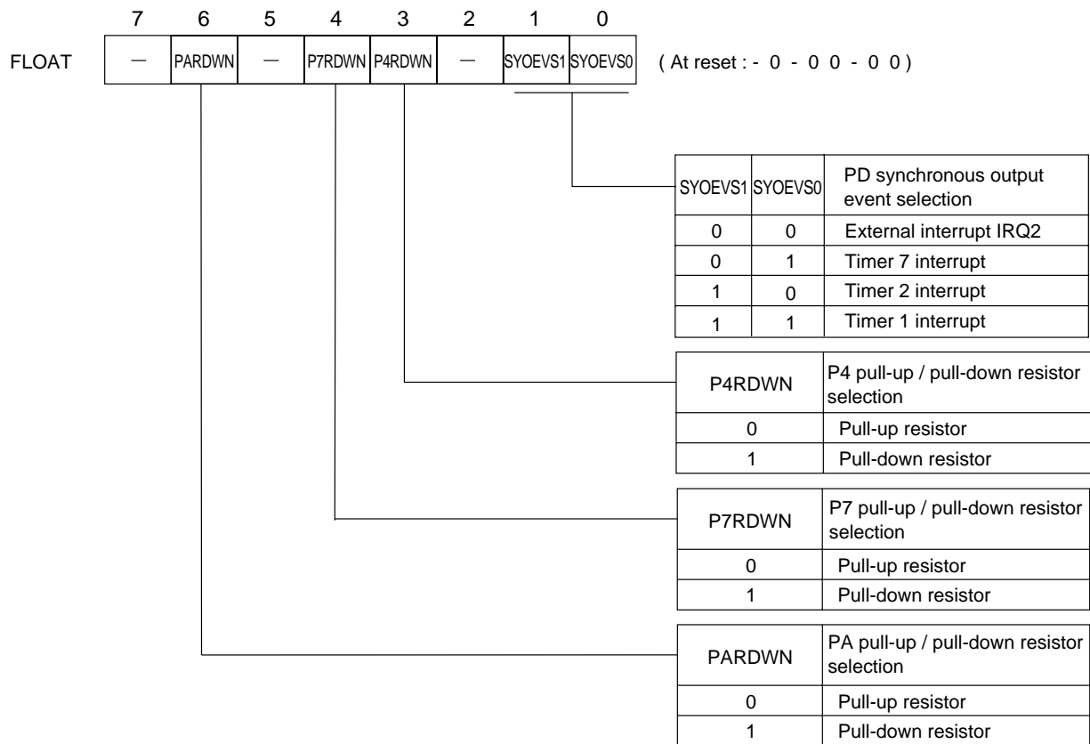
Pull-up / Pull-down resistor selection, pin control register (FLOAT : x'03F2E', R/W)
