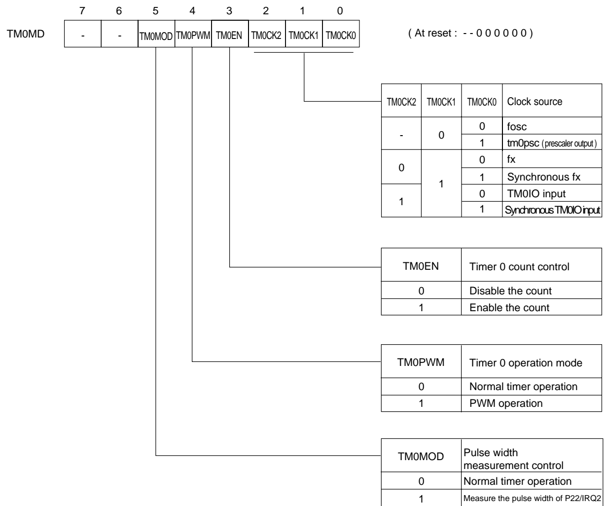
Figure 6-2-11 Timer 0 Mode Register (TM0MD : x'03F54', R/W)
