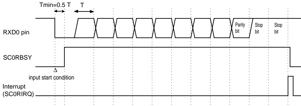
Figure 11-3-22 Reception Timing (parity bit is enabled)
