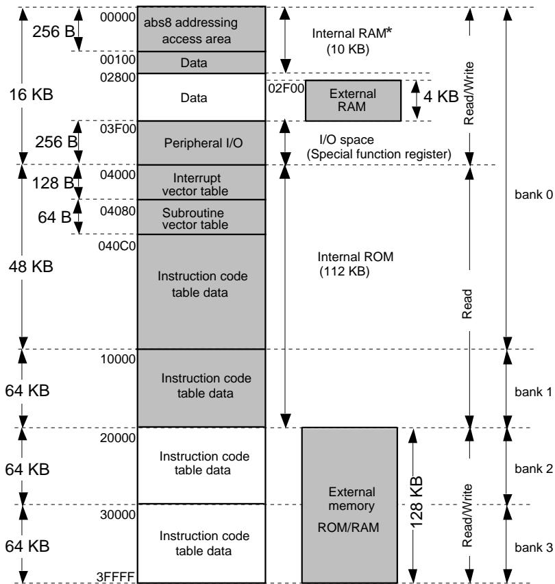
Figure 2-6-4 Memory Expansion Mode
