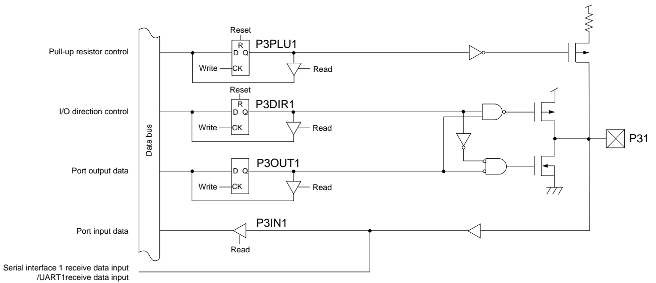
Figure 4-5-3 Block Diagram (P31)
