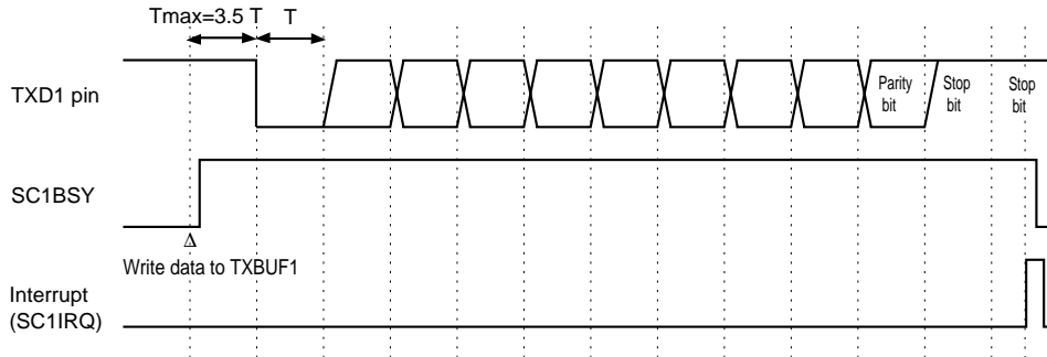
Figure 12-3-15 Transmission Timing (parity bit is enabled)
