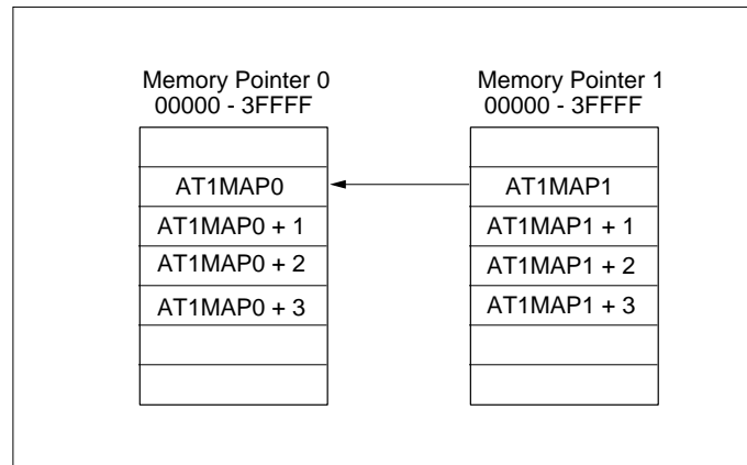
Figure 15-3-13 Transfer Mode B
