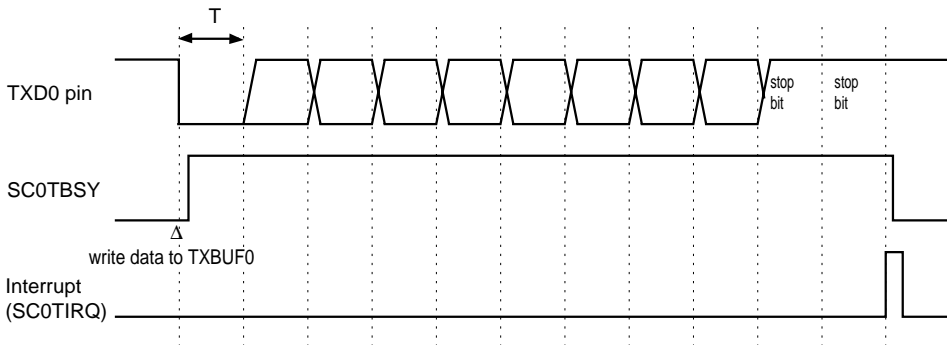
Figure 11-3-21 Transmission Timing (parity bit is disabled)
