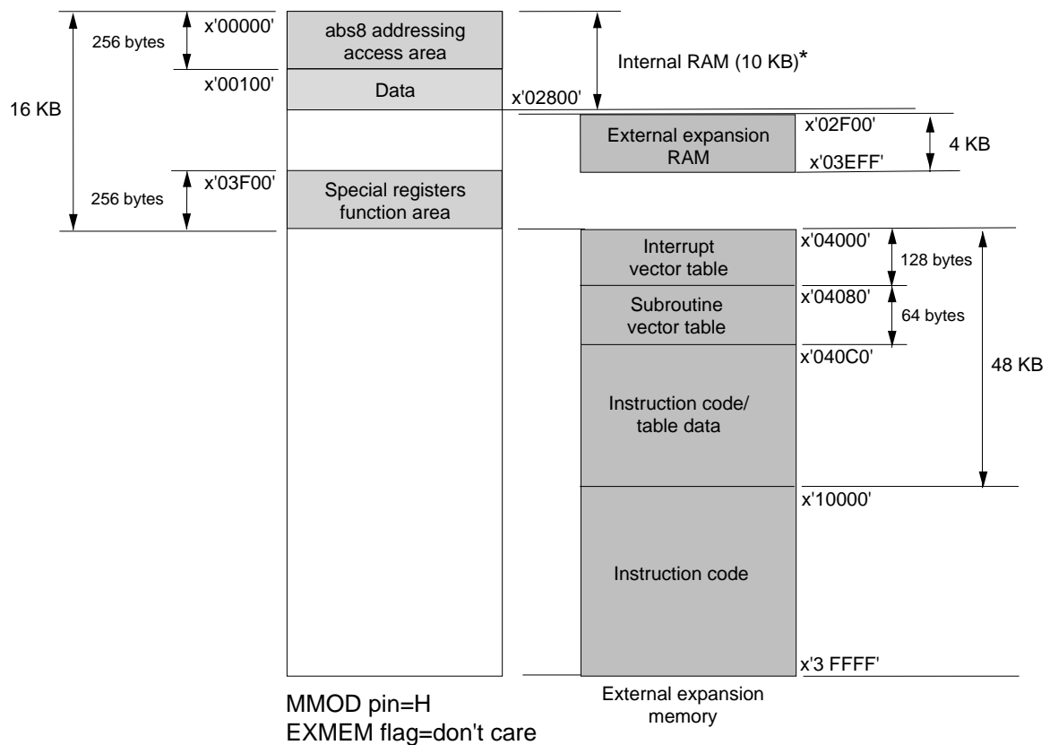
Figure 2-2-3 Processor Mode
