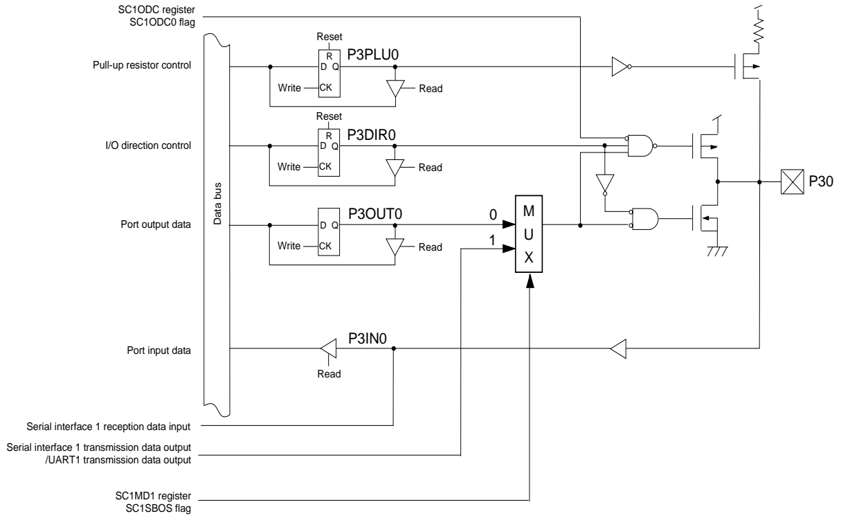
Figure 4-5-2 Block Diagram (P30)
