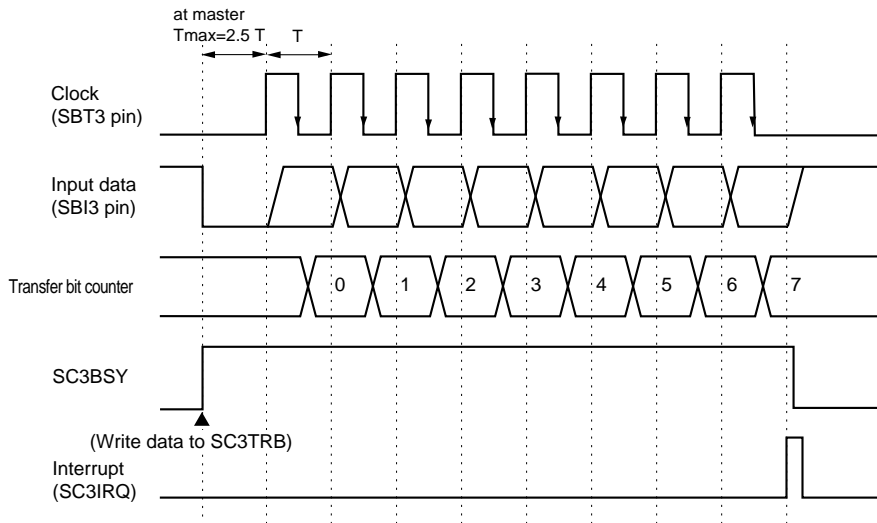
Figure 14-3-8 Reception Timing (Falling edge, Enable Start Condition)
