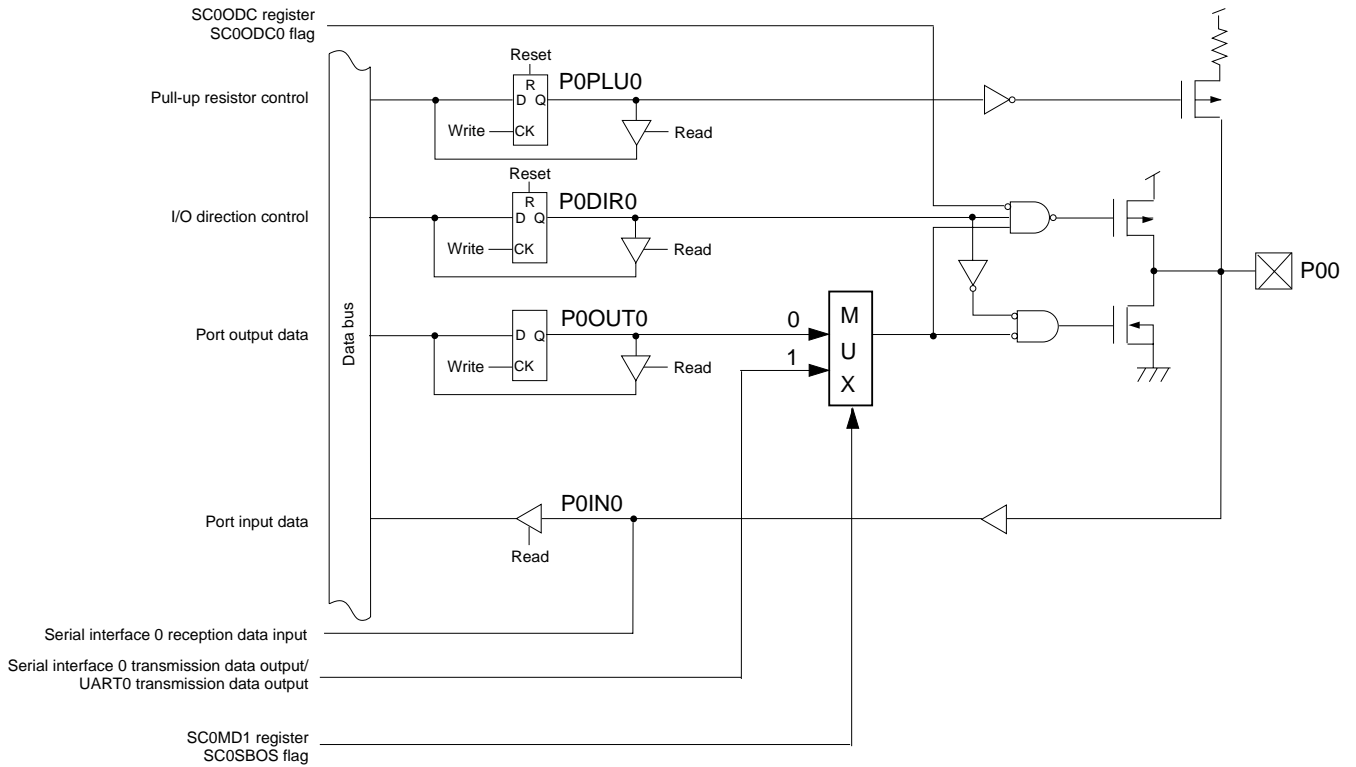
Figure 4-2-2 Block diagram (P00)
