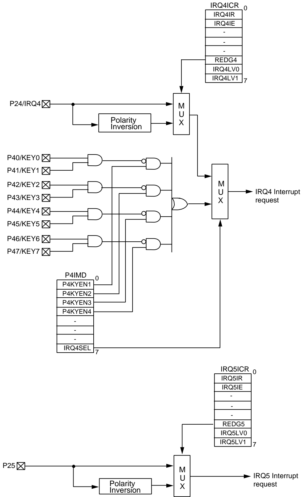
Figure 3-3-3 External Interrupt 4 Interface, External Interrupt 5 Interface, Block Diagram
