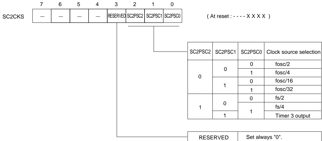
Figure 5-2-9 Serial Interface 2 Transfer Clock Selection Register (SC2CKS : x'03FA7', R/W)
