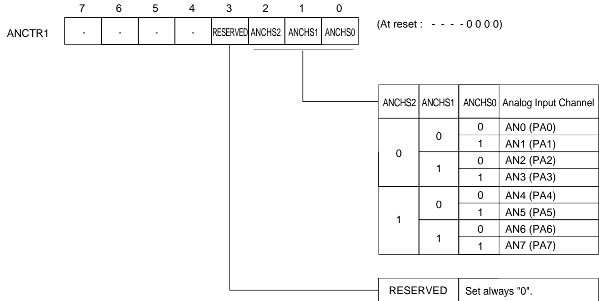
Figure 16-2-2 A/D Converter Control Register 1 (ANCTR1 : x'03FB1', R/W)
