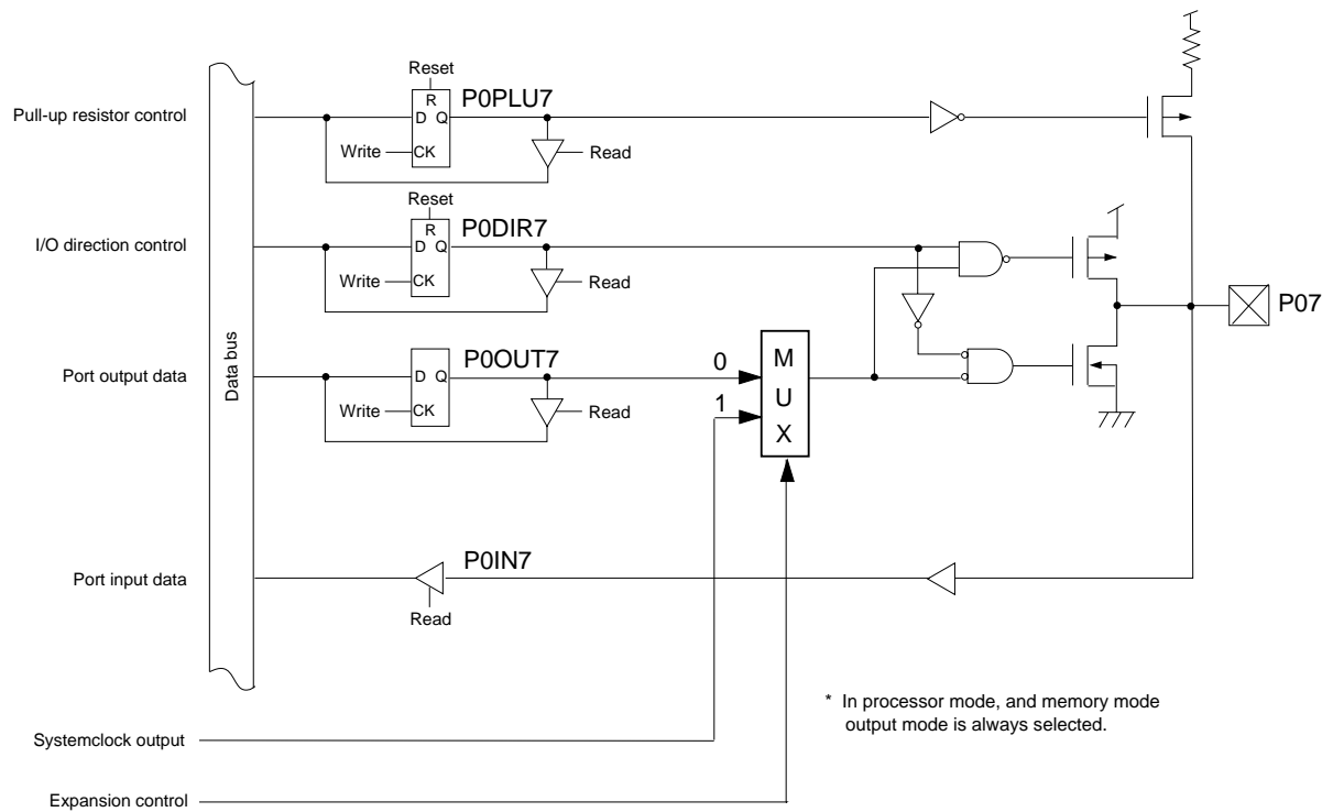
Figure 4-2-9 Block Diagram (P07)
