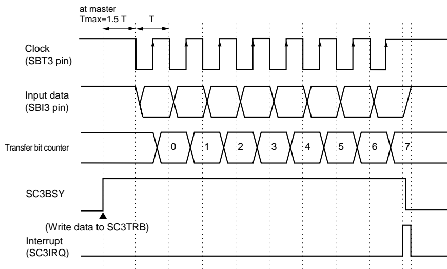
Figure 14-3-7 Reception Timing (Rising edge, Disable Start Condition)
