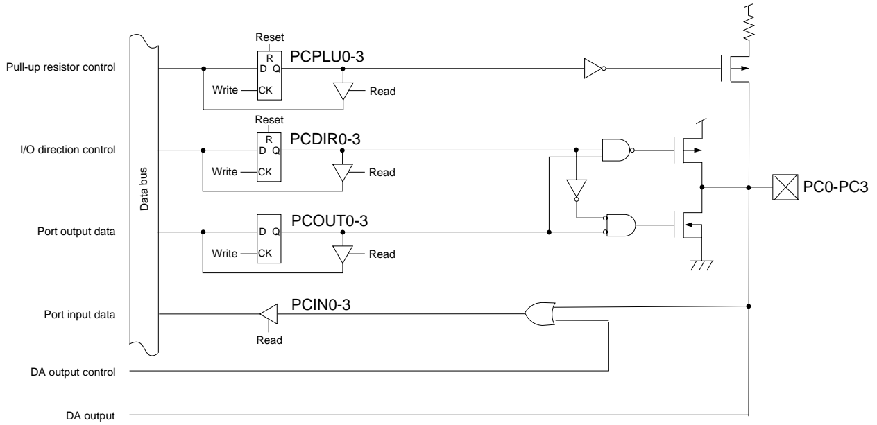
Figure 4-12-2 Block Diagram (PC0 to PC3)
