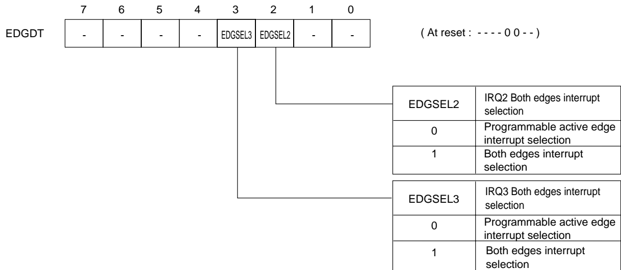
Figure 3-3-5 Both Edges Interrupt Control Register (EDGDT : x'03F8F', R/W)
