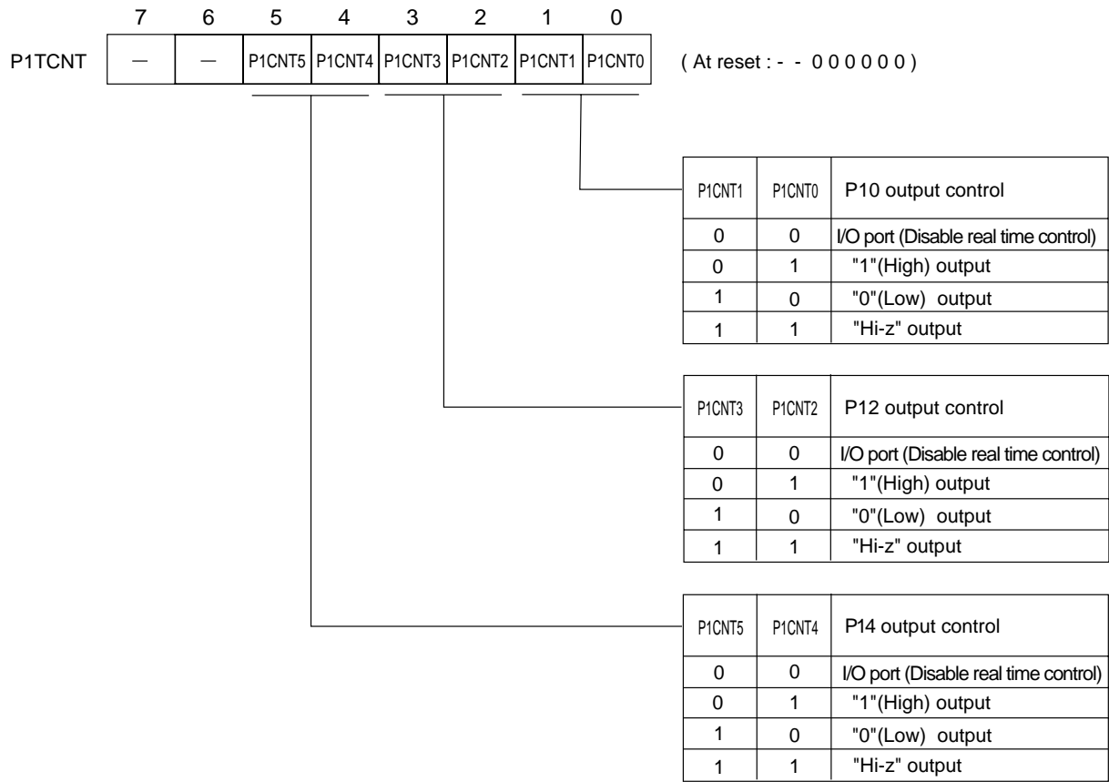
Port 1 output control register (P1TCNT : x'03F7E', R/W)
