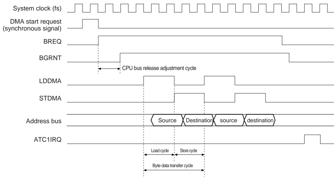
Figure 15-3-1 ATC1 Timing Chart
