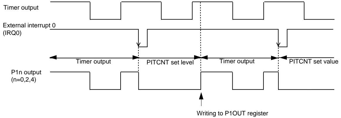
Figure 4-14-1 Real Time Output Control Timing
