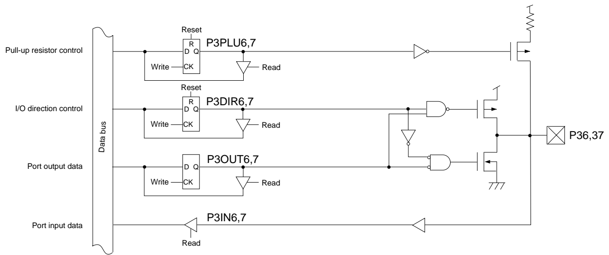
Figure 4-5-8 Block Diagram (P36,37)
