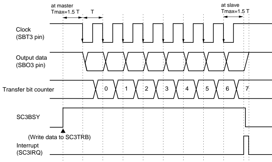
Figure 14-3-3 Transmission Timing (Falling edge, Disable Start Condition)
