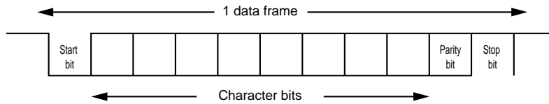
Figure 12-3-14 UART Serial Interface Transmission / Reception Data Format
