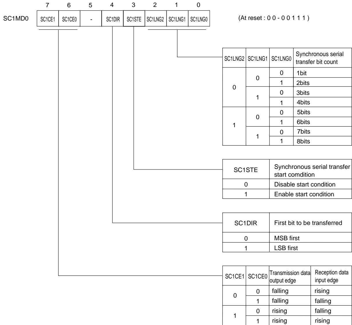
Figure 12-2-3 Serial Interface 1 Mode Register 0 (SC1MD0 : x'03F9A', R/W)
