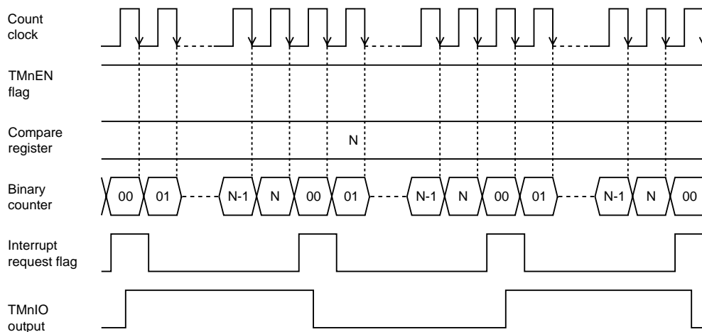
Figure 6-5-1 Count Timing of Timer Pulse Output (Timers 0 to 4)
