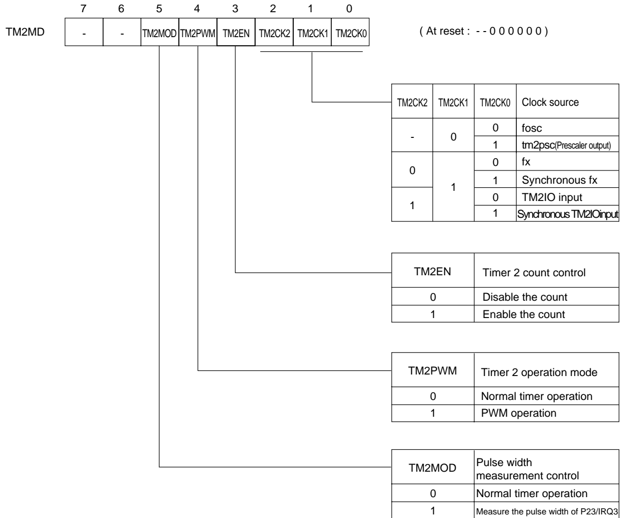
Figure 6-2-13 Timer 2 Mode Register (TM2MD : x'03F5C', R/W)
