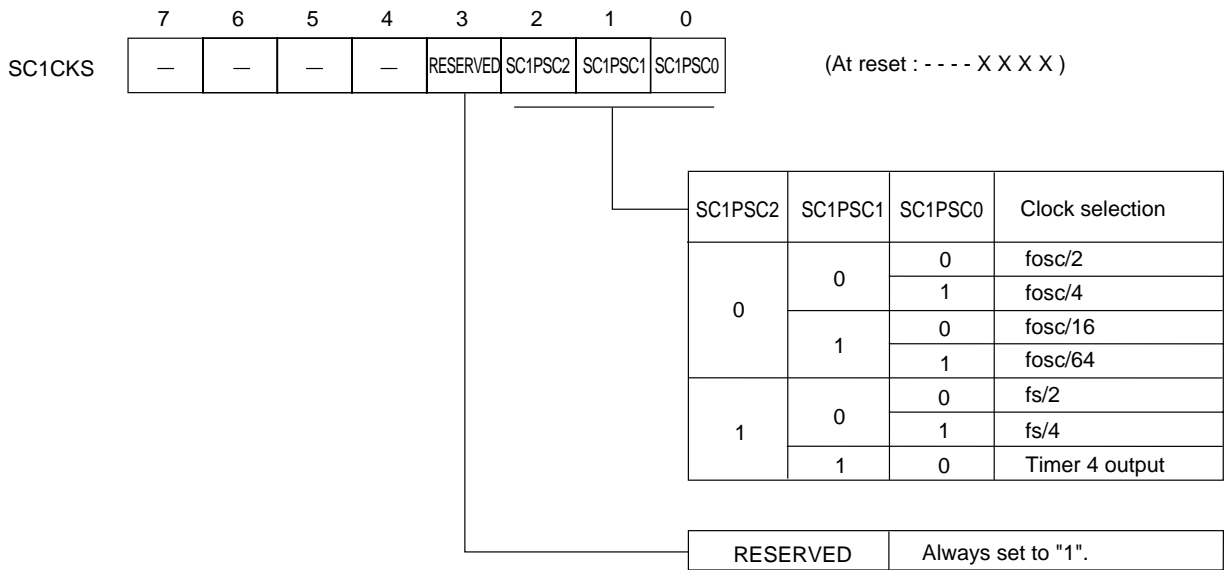
Figure 12-2-8 Serial Interface 1 Transfer Clock Selection Register (SC1CKS : x'03F9F', R/W)
