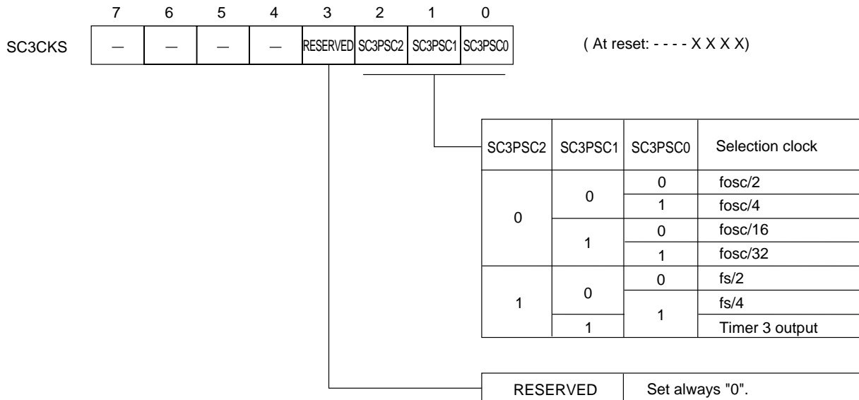
Figure 14-2-6 Serial Interface 3 Transfer Clock Selection Register (SC3CKS : x'03FAF', R/W)
