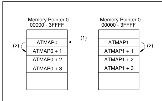
Figure 15-3-15 Transfer Mode D
