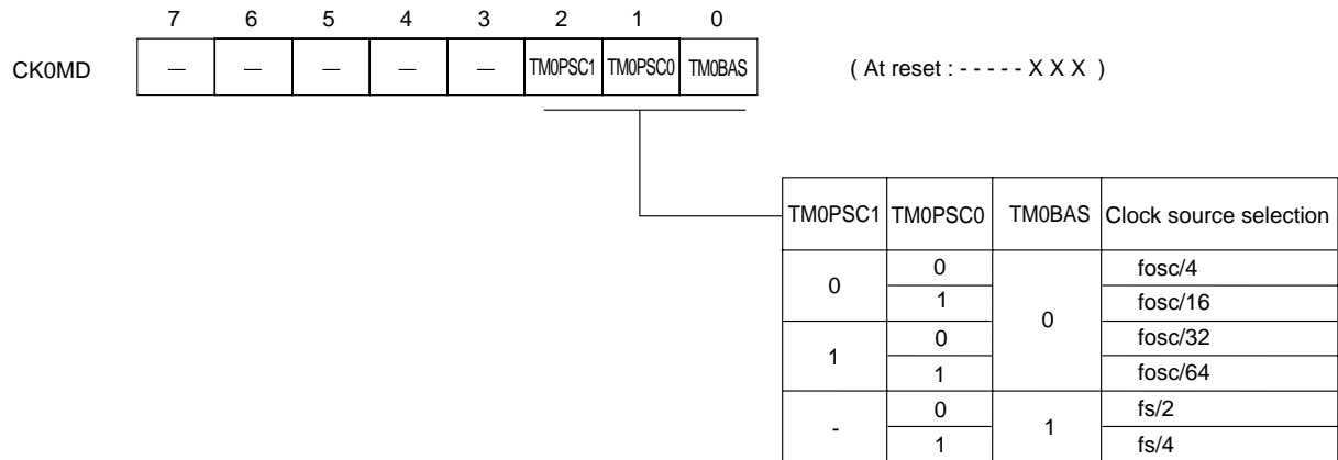
Figure 5-2-2 Timer 0 Prescaler Selection Register (CK0MD : x'03F56', R/W)
