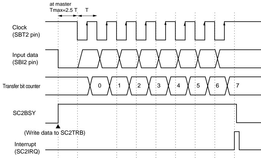
Figure 13-3-6 Reception Timing (Rising edge, Start condition is enabled)
