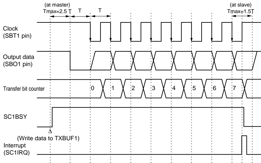
Figure 12-3-4 Transmission Timing (falling edge, start condition is enabled)
