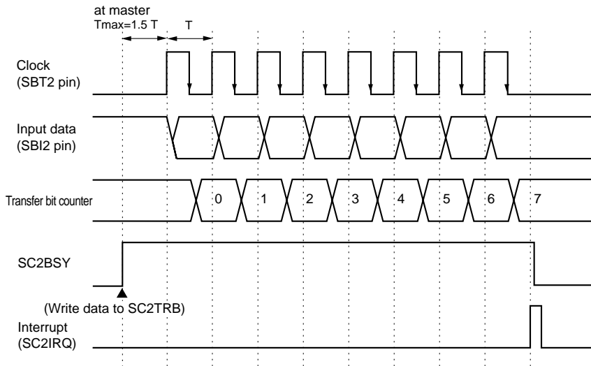
Figure 13-3-9 Reception Timing (Falling edge, Start condition is disabled)
