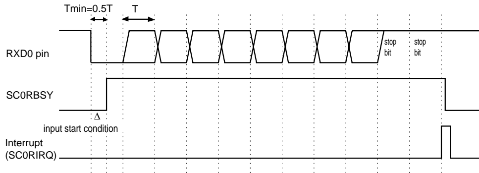
Figure 11-3-23 Reception Timing (parity bit is disabled)
