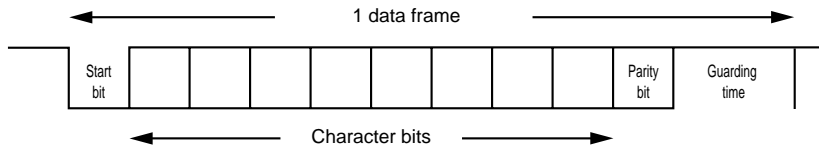
Figure 12-3-19 ATR Communication Data Format
