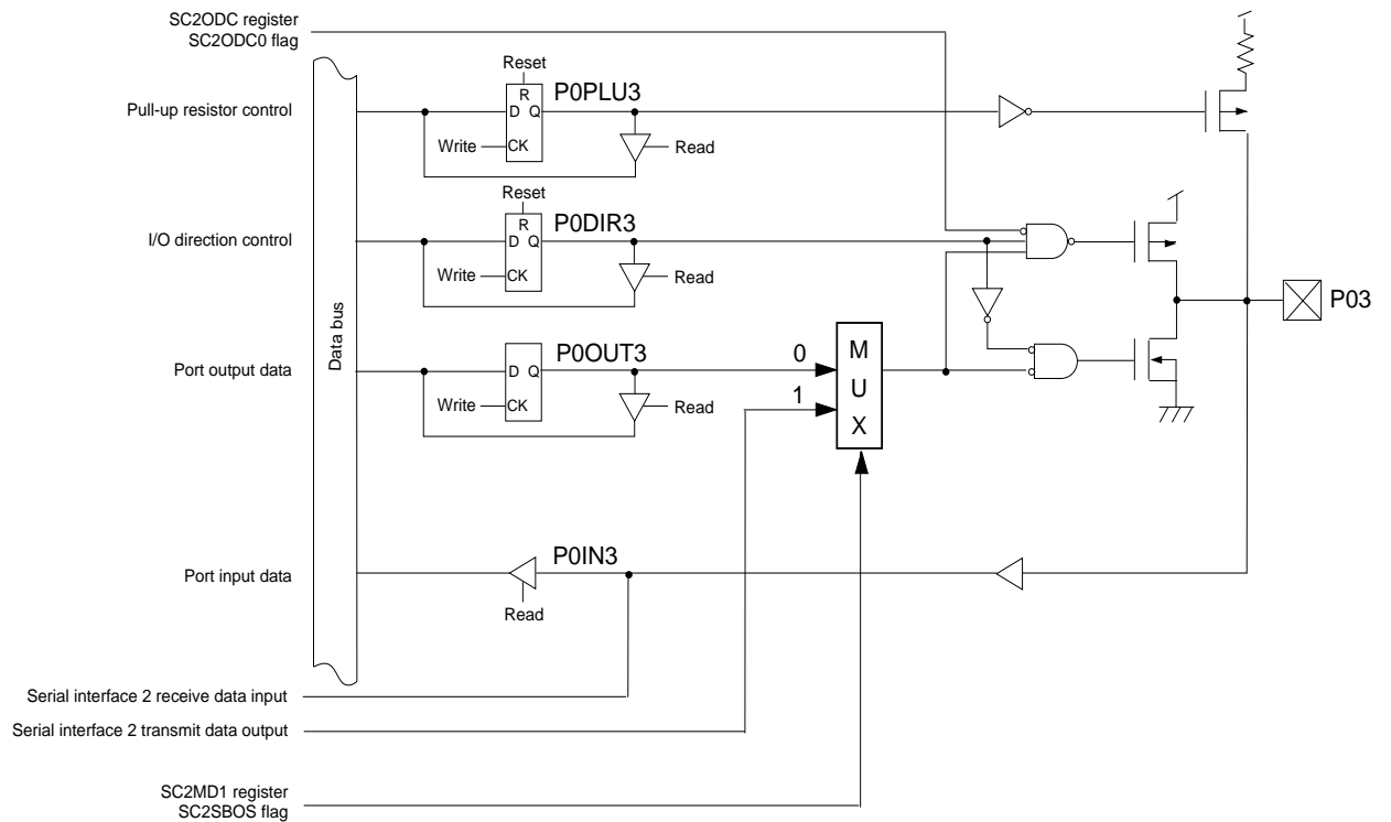
Figure 4-2-5 Block diagram (P03)
