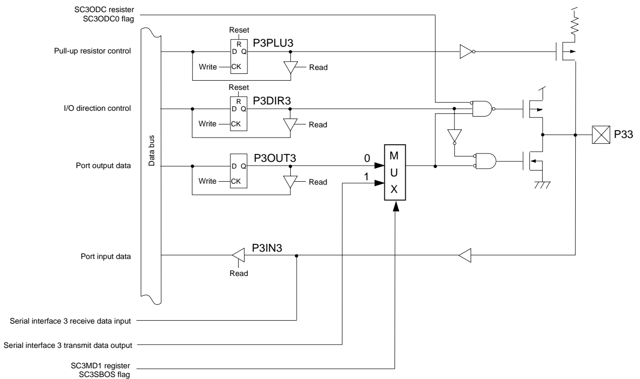
Figure 4-5-5 Block Diagram (P33)
