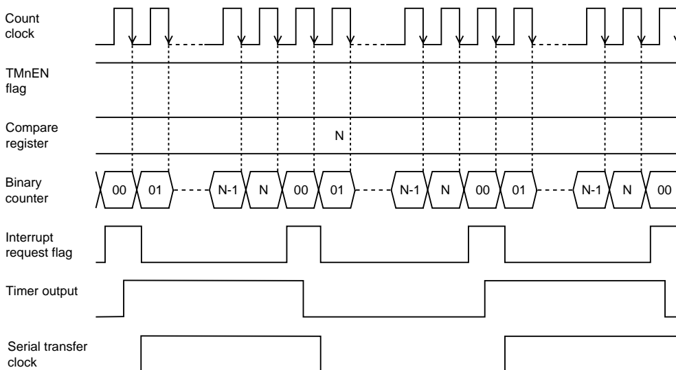
Figure 6-8-1 Timing of Serial Interface Transfer Clock (Timers 2, 3 and 4)
