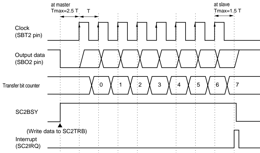
Figure 13-3-4 Transmission Timing (Rising edge, Start condition is enabled)
