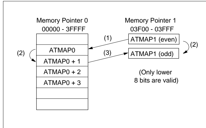
Figure 15-3-11 Transfer Mode 9
