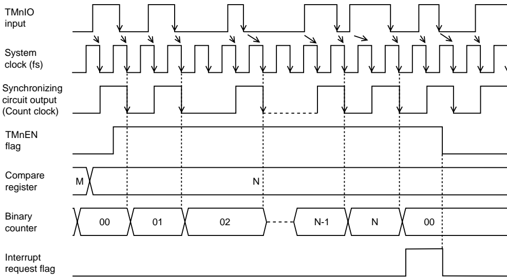
Figure 6-4-2 Count Timing of Synchronous TMnIO Input (Timers 0 to 4)
