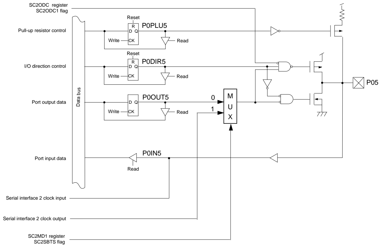
Figure 4-2-7 Block Diagram (P05)
