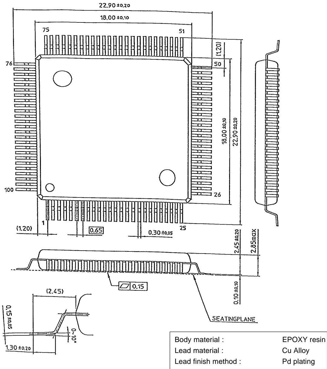
Figure 1-6-1 100-Pin QFP
