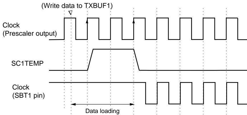
Figure 12-3-1 Data Loading Period and Transmission Buffer Empty Flag
