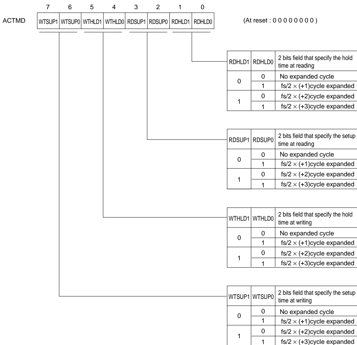
Figure 18-1-1 AC Timing Control Register (ACTMD : x'03F06', R/W)
