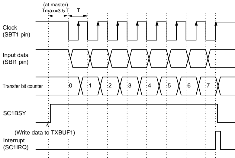
Figure 12-3-9 Reception Timing (rising edge, start condition is disabled)
