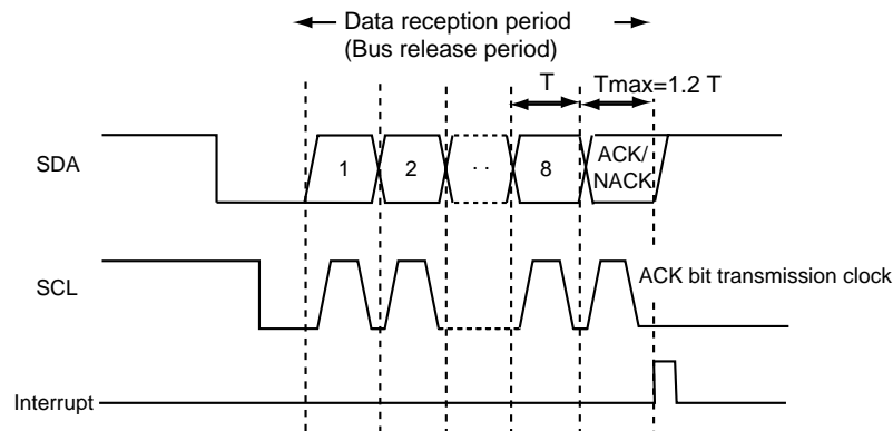
Figure 14-3-14 ACK Bit Transmission Timing after Reception of 8-bit Data
