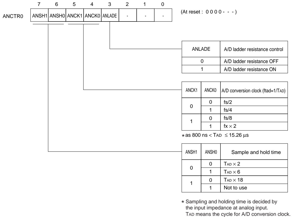
Figure 16-2-1 A/D Converter Control Register 0 (ANCTR0 : x'03FB0', R/W)
