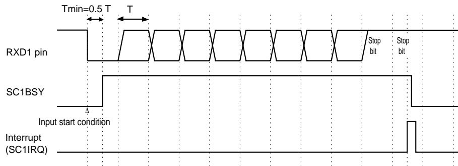
Figure 12-3-18 Reception Timing (parity bit is disabled)
