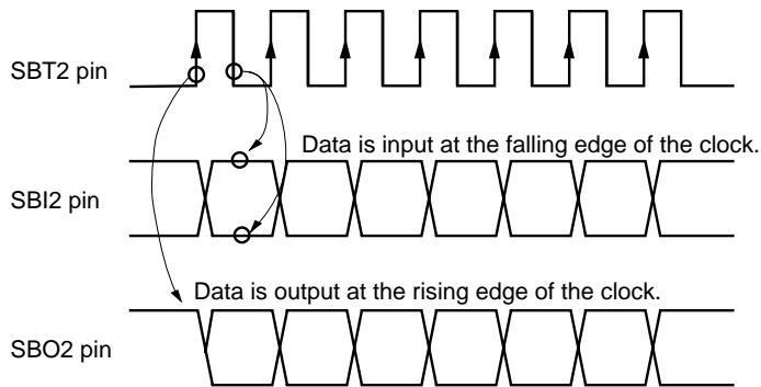
Figure 13-3-11 Transmission / Reception Timing (Reception : Falling edge, Transmission : Rising edge)
