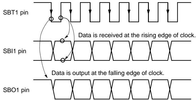
Figure 12-3-12 Transmission / Reception Timing (Reception : rising edge, Transmission : falling edge)
