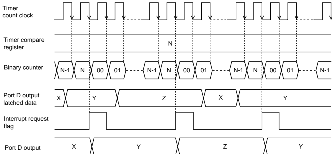
Figure 4-15-3 Synchronous Output Timing by Event Generation (Timers 1, 2 and 7)
