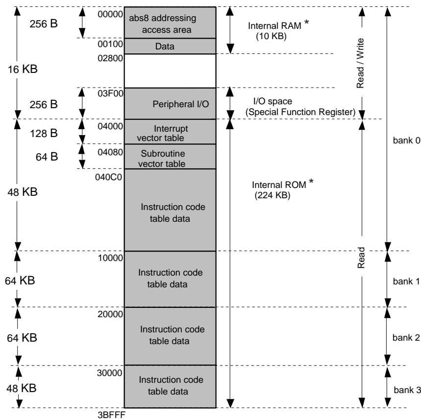
Figure 2-6-3 Single Chip Mode
