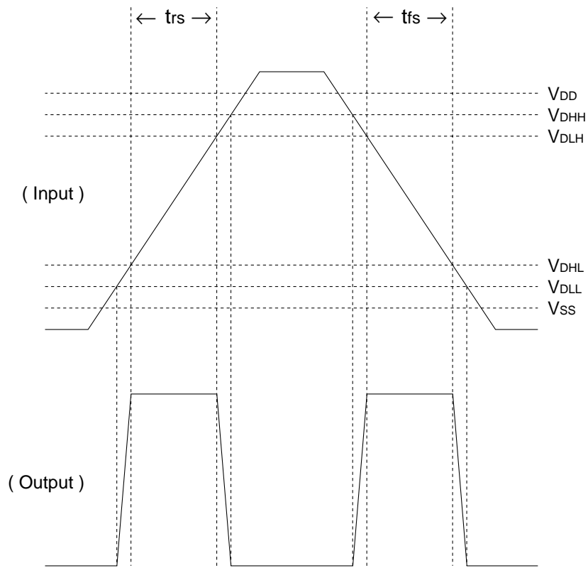
Figure 20-3-5 AC Zero-Cross Detector
