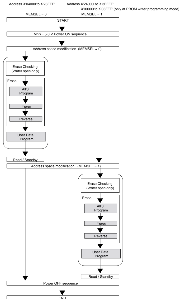
Figure 20-4-1 Reprogramming Flow of Internal Flash EEPROM
