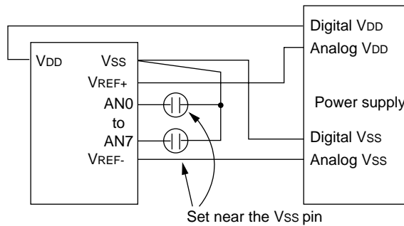
Figure 16-3-2 A/D Converter Recommended Example 1
