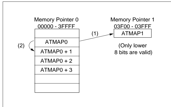
Figure 15-3-4 Transfer Mode 2
