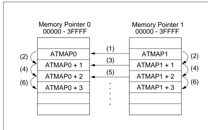
Figure 15-3-17 Transfer Mode F
