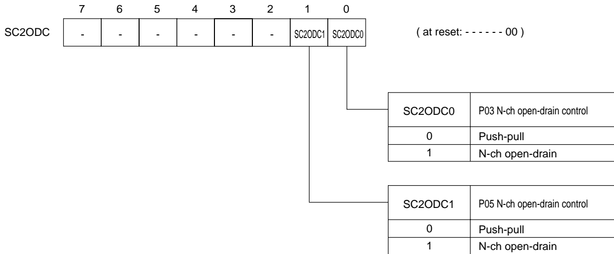
Figure 13-2-4 Serial Interface 2 Port Control Register (SC2ODC : x'03FA6', R/W)
