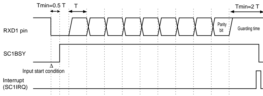
Figure 12-3-23 Reception Timing (T=0, 1 Data Communication)
