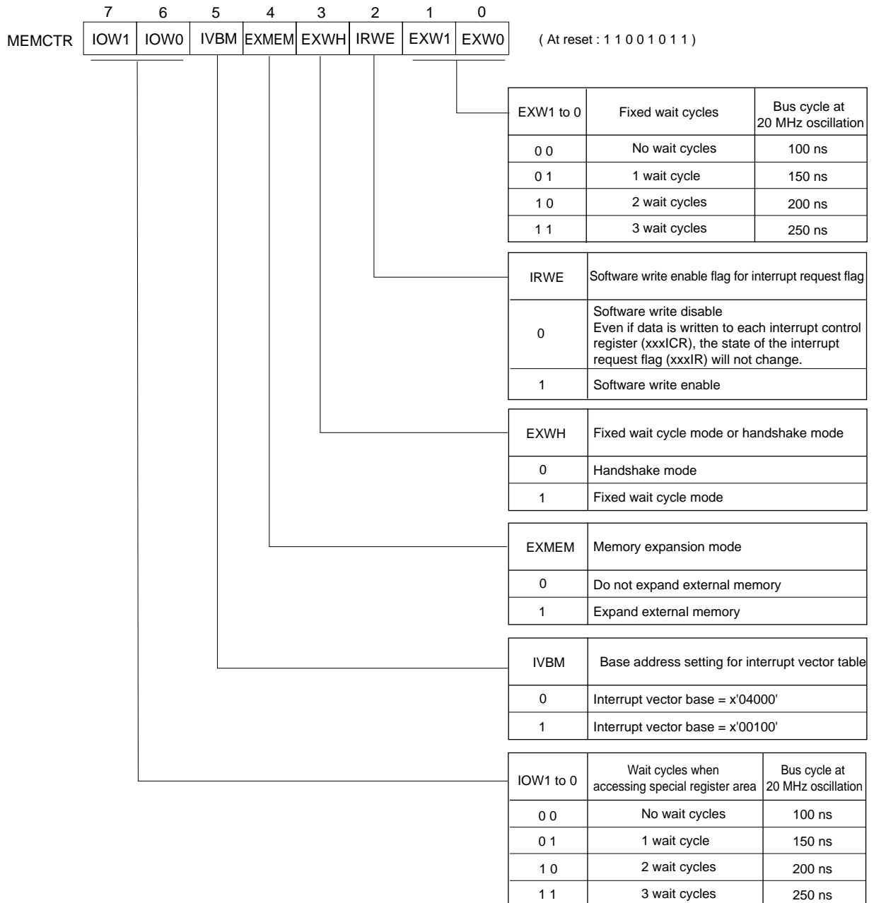
Figure 2-3-2 Memory Control Register (MEMCTR: x'03F01' R/W)
