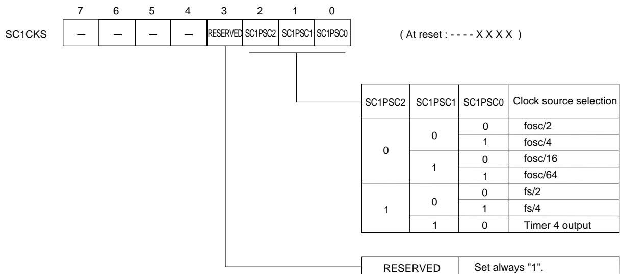
Figure 5-2-8 Serial Interface 1 Transfer Clock Selection Register (SC1CKS : x'03F9F', R/W)
