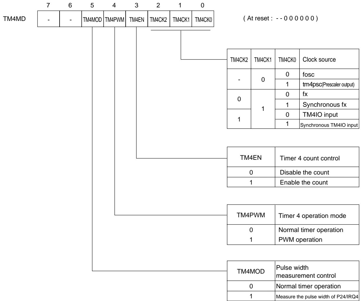
Figure 6-2-15 Timer 4 Mode Register (TM4MD : x'03F64', R/W)
