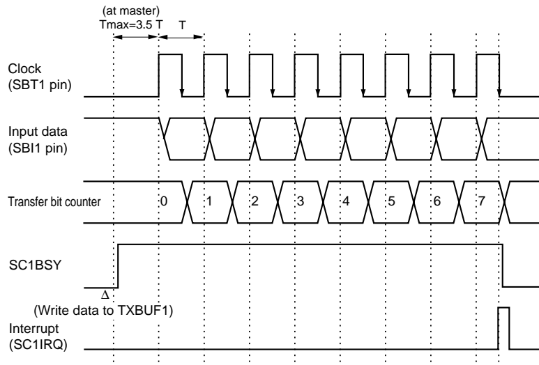
Figure 12-3-11 Reception Timing (falling edge, start condition is disabled)
