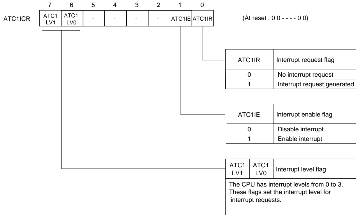
Figure 3-2-23 ATC1 Interrupt Control Register (ATC1ICR : x'03FFC', R/W)
