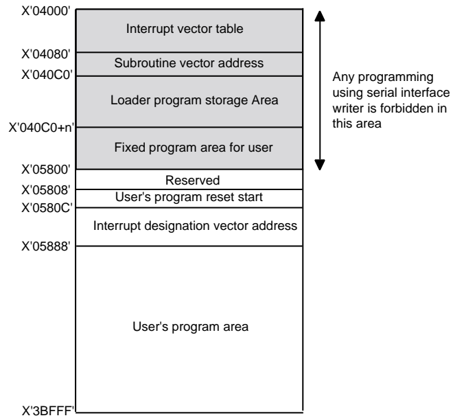
Figure 20-6-3 Internal Flash EEPROM Memory map
