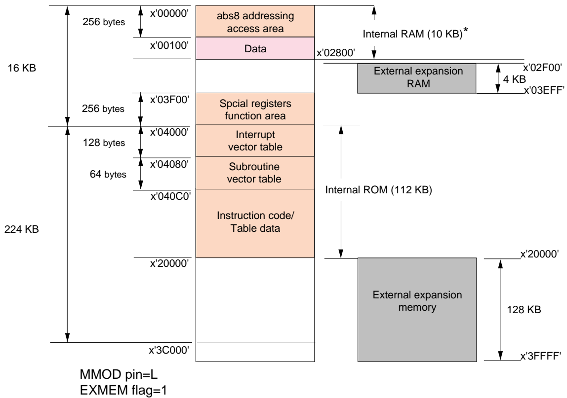
Figure 2-2-2 Memory Expansion Mode
