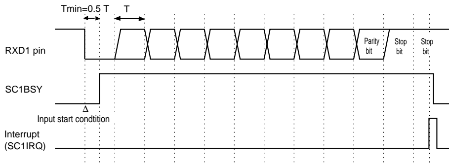
Figure 12-3-17 Reception Timing (parity bit is enabled)
