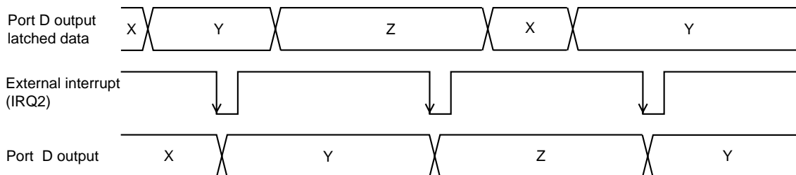
Figure 4-15-2 Synchronous Output Timing by Event Generation (IRQ2)
