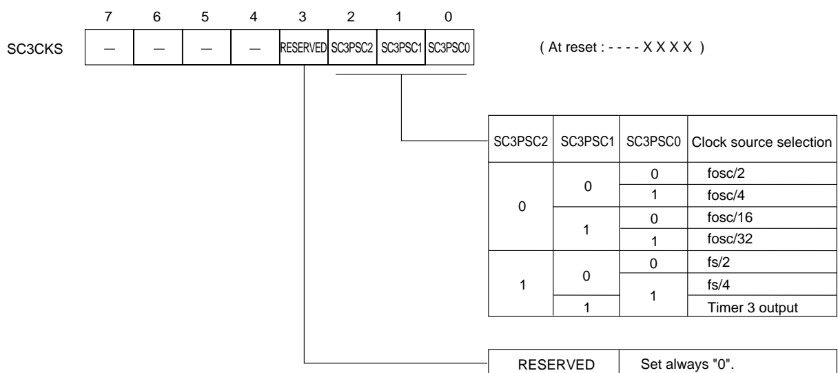
Figure 5-2-10 Serial Interface 3 Transfer Clock Selection Register (SC3CKS : x'03FAF', R/W)
