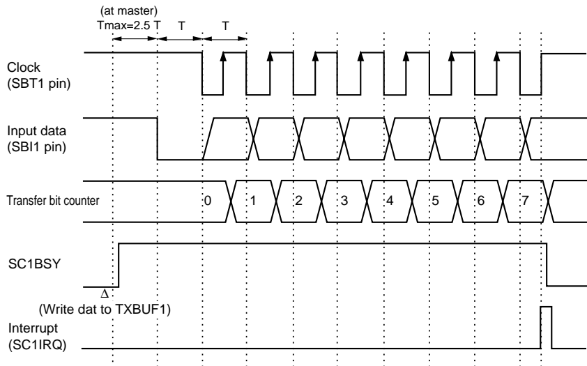
Figure 12-3-8 Reception Timing (rising edge, start condition is enabled)
