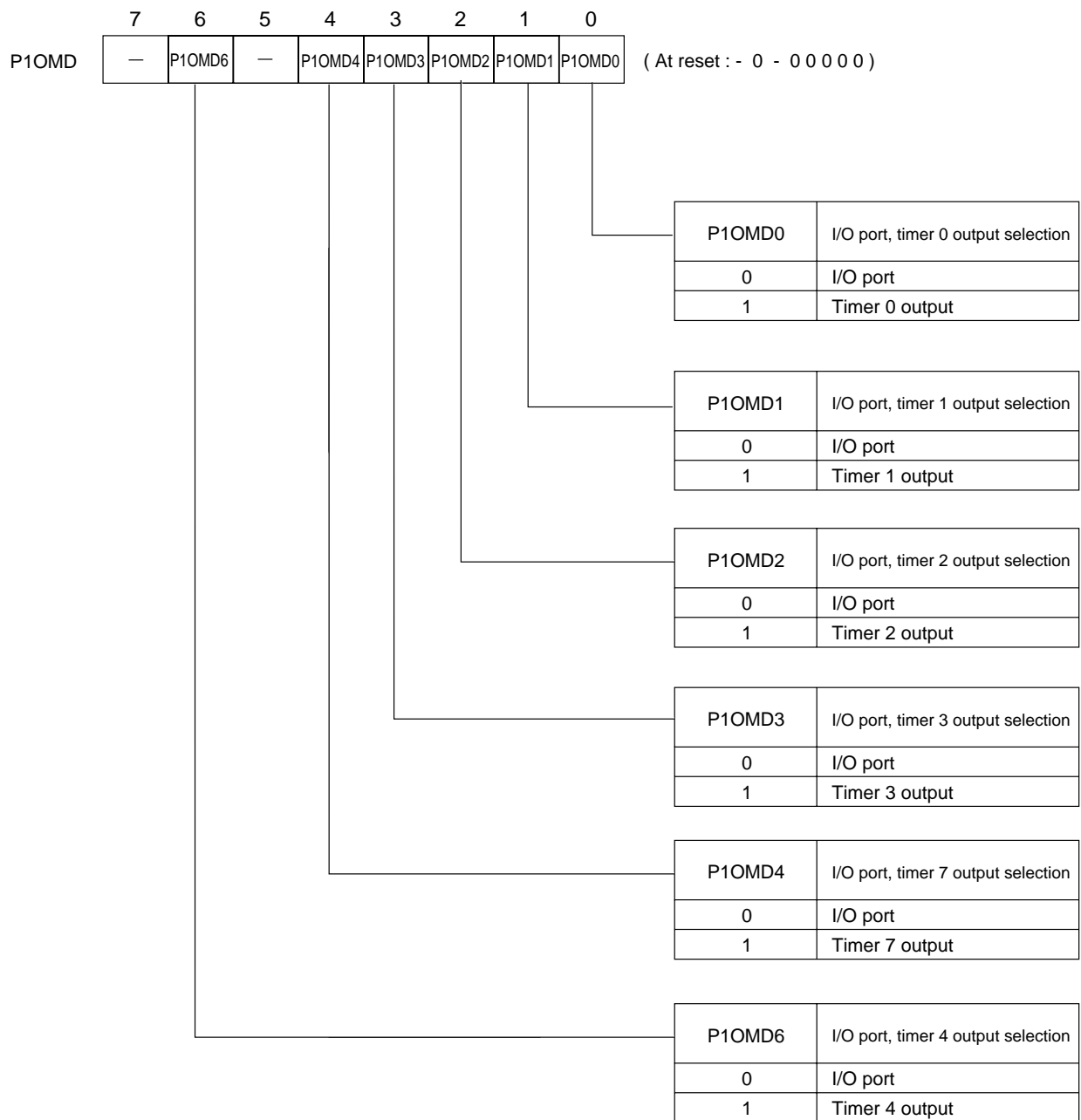
Port 1 output mode register (P1OMD : x'03F2F', R/W)
