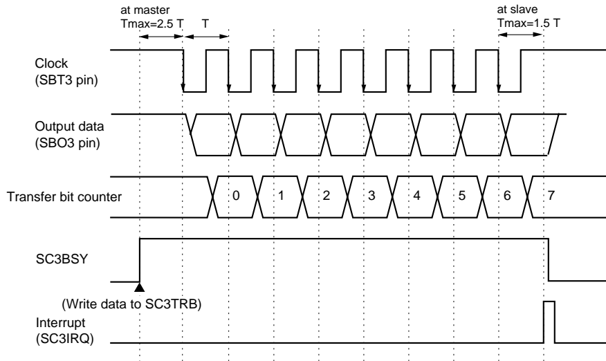
Figure 14-3-2 Transmission Timing (Falling edge, Enable Start Condition)
