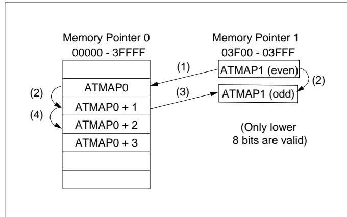
Figure 15-3-10 Transfer Mode 8
