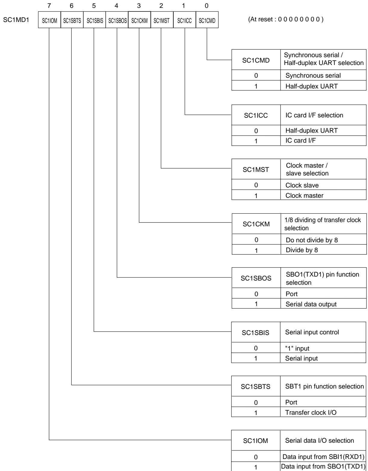
Figure 12-2-4 Serial Interface 1 Mode Register 1 (SC1MD1 : x'03F9B', R/W)
