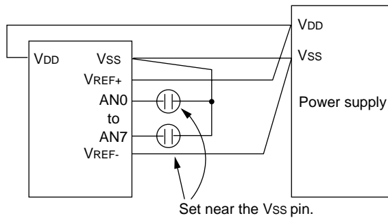
Figure 16-3-3 A/D Converter Recommended Example 2
