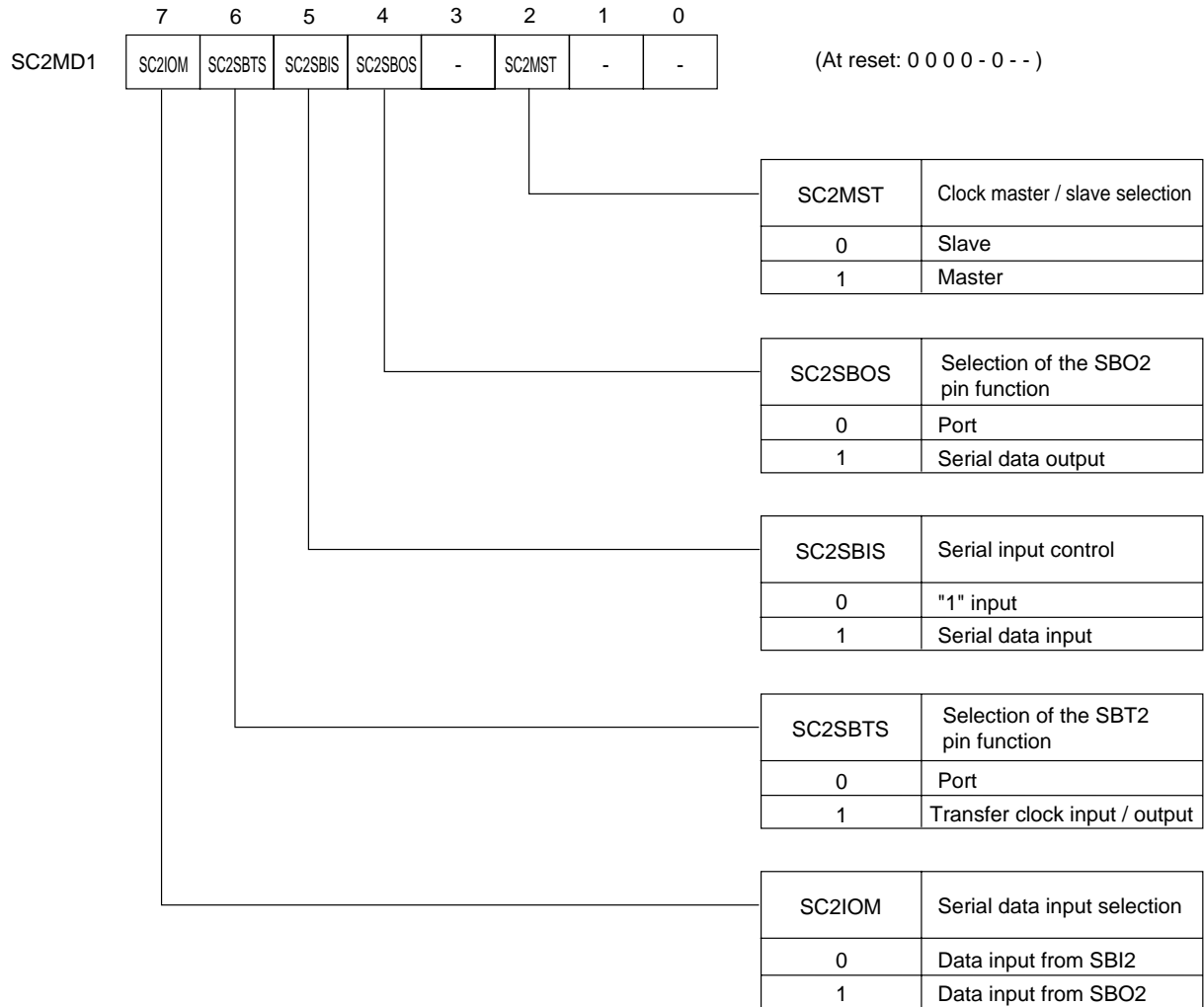
Figure 13-2-3 Serial Interface 2 Mode Register 1 (SC2MD1 : x'03FA1', R/W)
