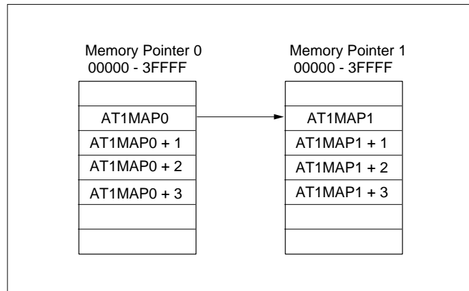
Figure 15-3-12 Transfer Mode A
