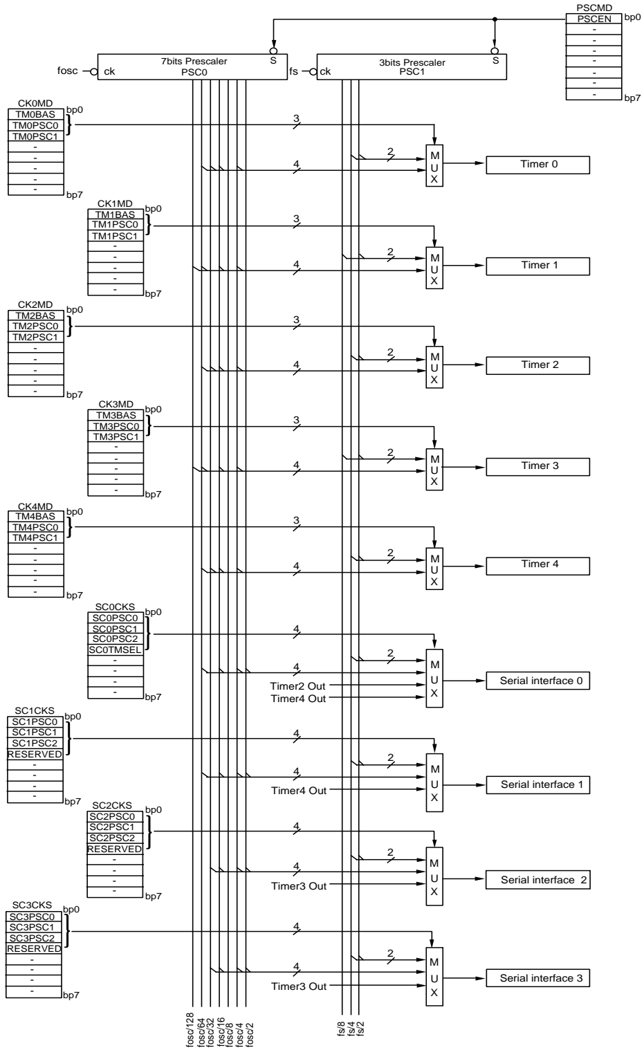
Figure 5-1-1 Prescaler Block Diagram
