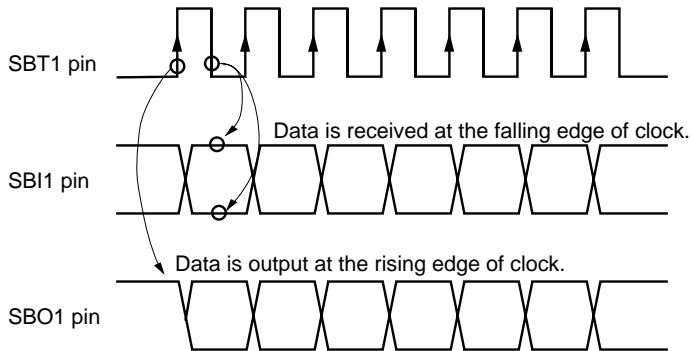
Figure 12-3-13 Transmission / Reception Timing (Reception : falling edge, Transmission : rising edge)
