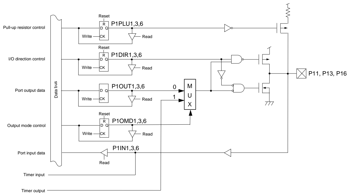
Figure 4-3-5 Block Diagram (P11, P13, P16)
