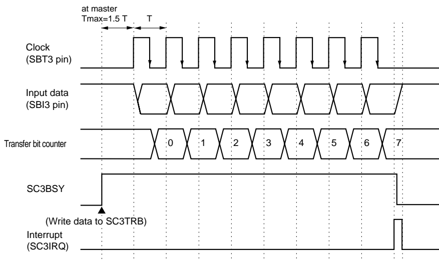
Figure 14-3-9 Reception Timing (Falling edge, Disable Start Condition)
