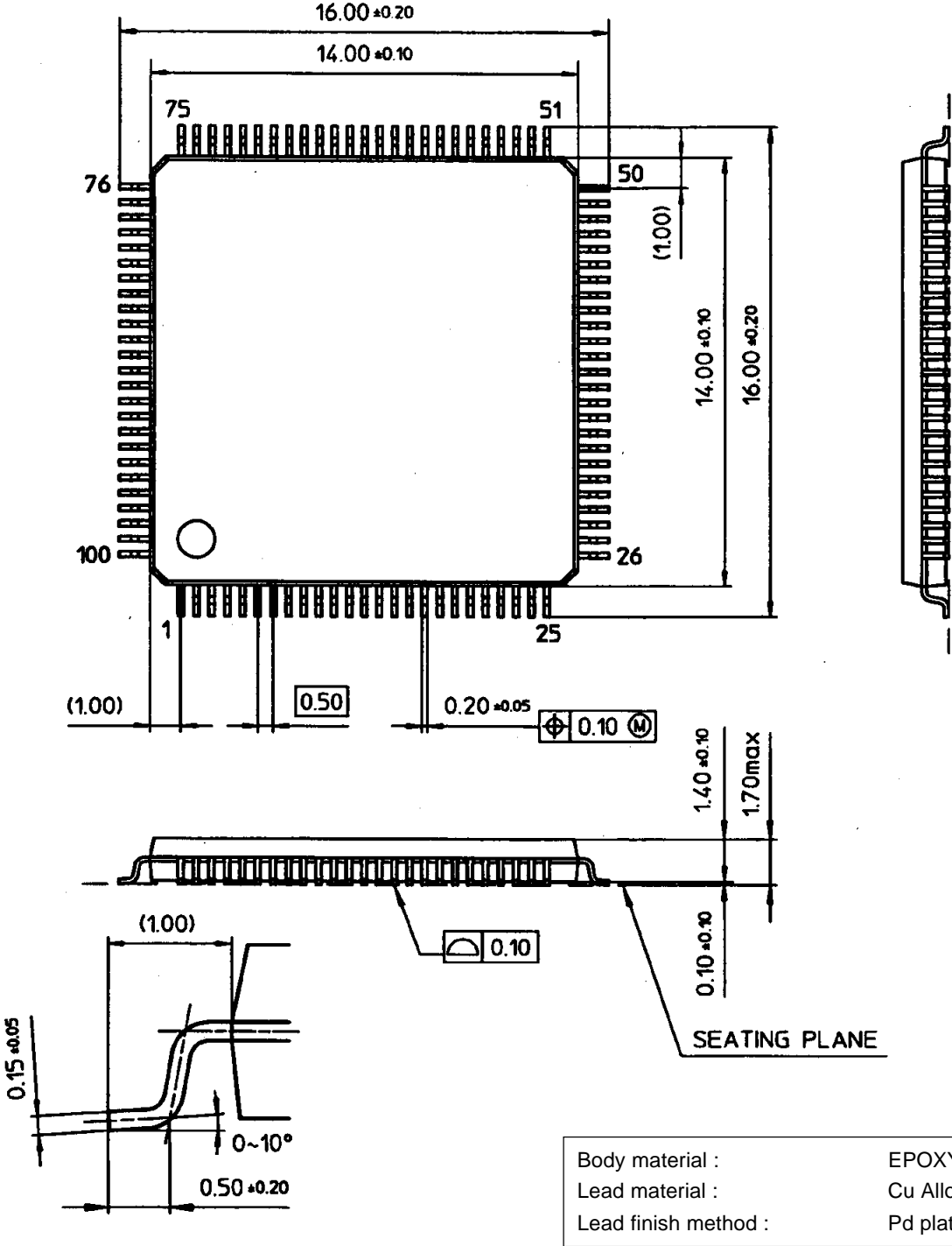
Figure 1-6-2 100-Pin LQFP
