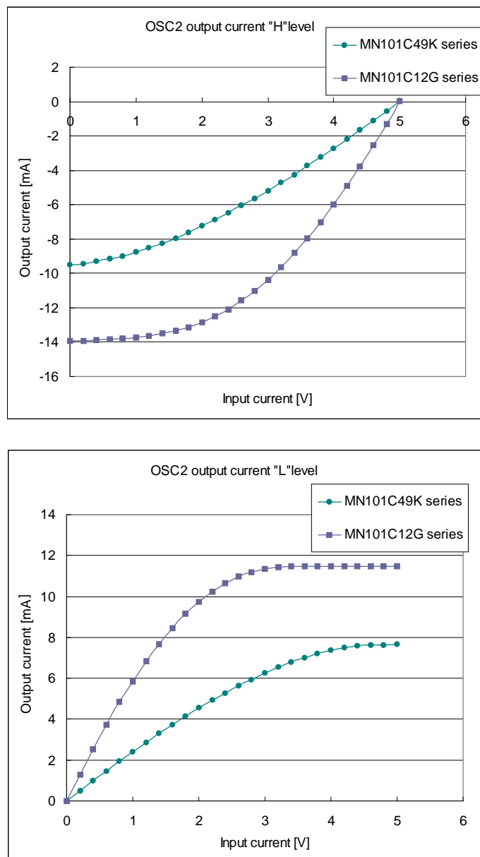
Figure 19-2-1 MN101C49K OSC2 pin's output current
