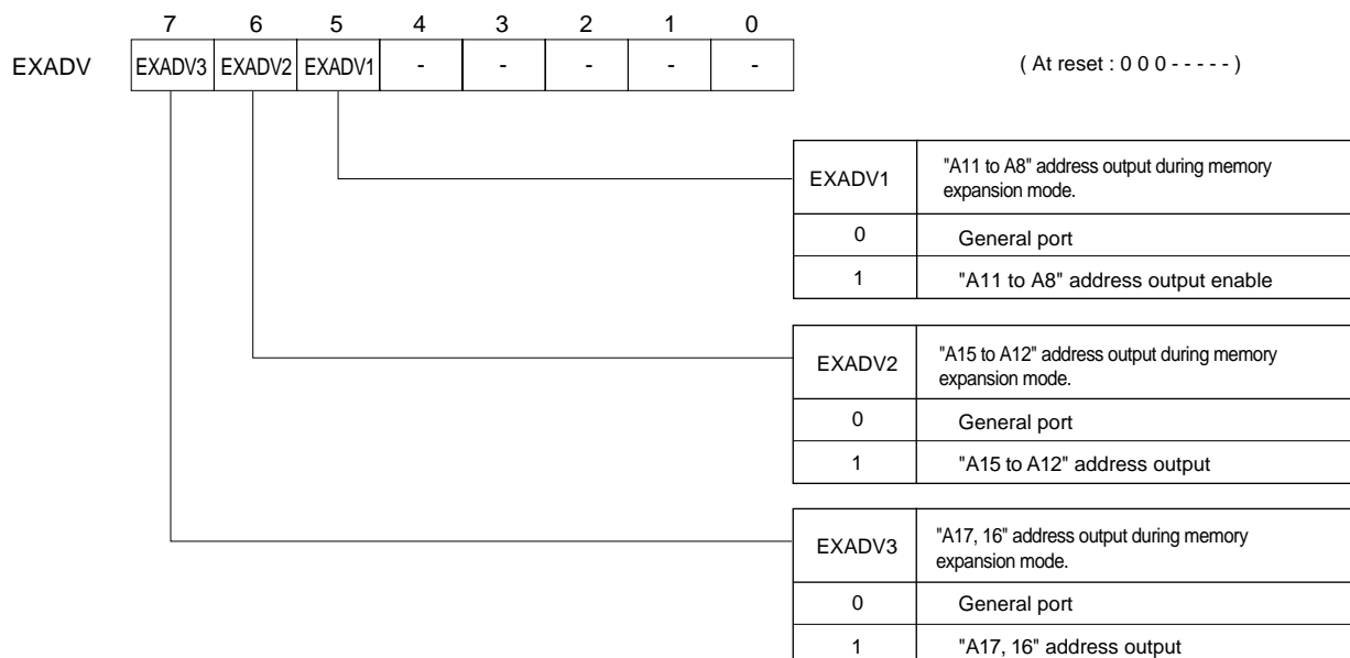
Figure 2-3-3 Expansion Address Control Register (EXADV : x'03F0E', R/W)
