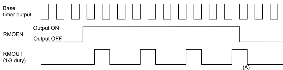
Figure 6-11-2 Count Timing of Remote Control Carrier Output Function (Timer 0, Timer 3)
