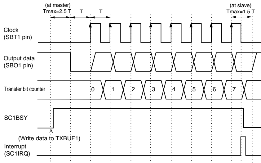
Figure 12-3-6 Transmission Timing (rising edge, start condition is enabled)
