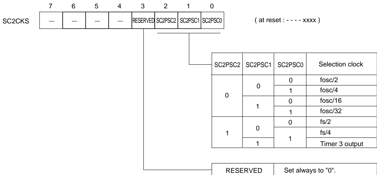
Figure 13-2-5 Serial Interface 2 Transfer Clock Selection Register (SC2CKS : x'03FA7', R/W)
