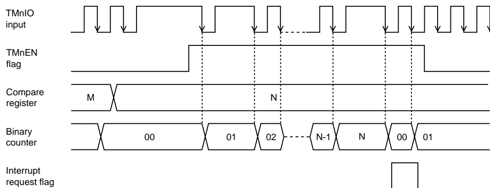
Figure 6-4-1 Count Timing of TMnIO Input (Timers 0 to 4)
