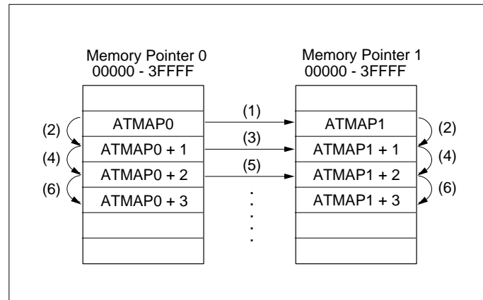
Figure 15-3-16 Transfer Mode E
