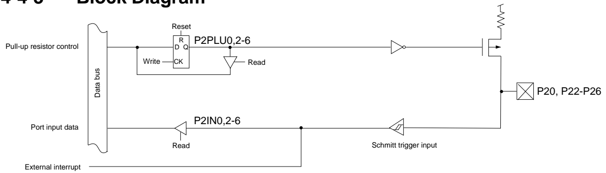
Figure 4-4-2 Block Diagram (P20, P22 to P26)
