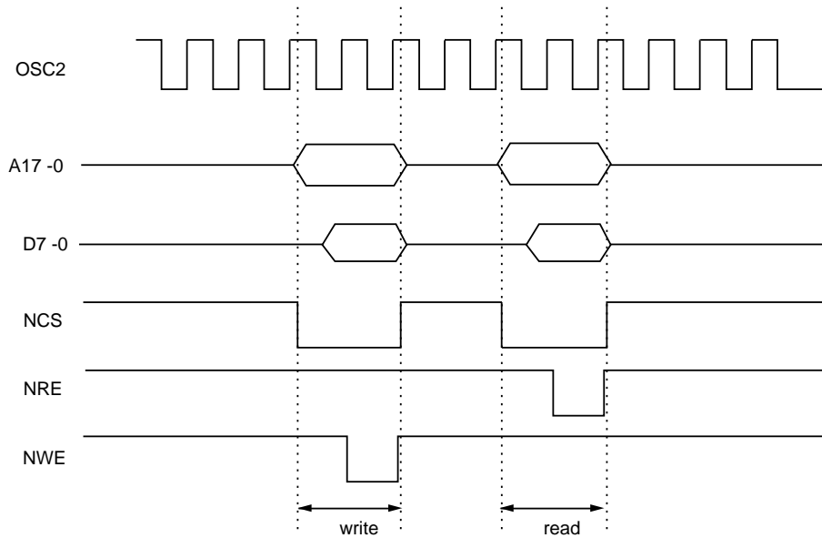
Figure 2-3-4 ROM and RAM Access Timing with No Wait Cycles
