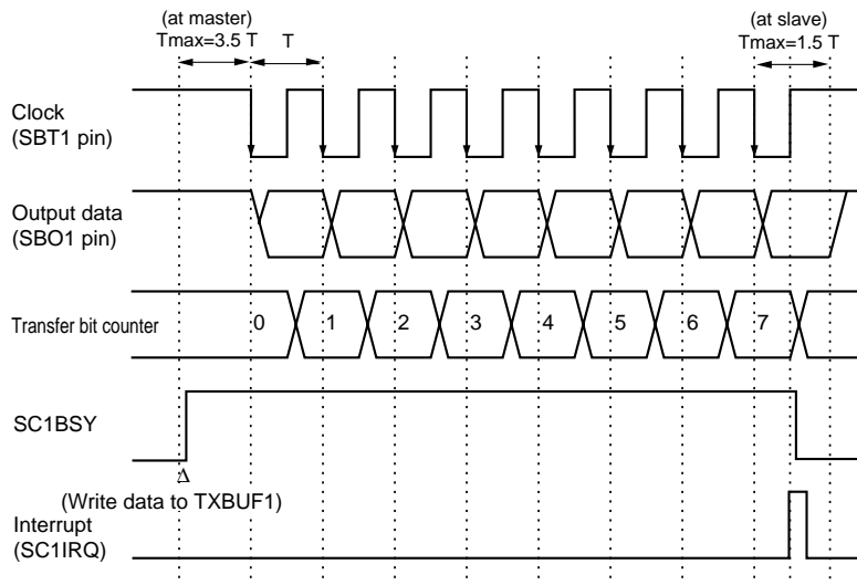
Figure 12-3-5 Transmission Timing (falling edge, start condition is disabled)
