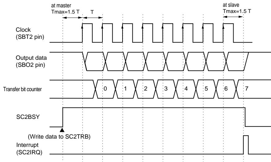
Figure 13-3-5 Transmission Timing (Rising edge, Start condition is disabled)
