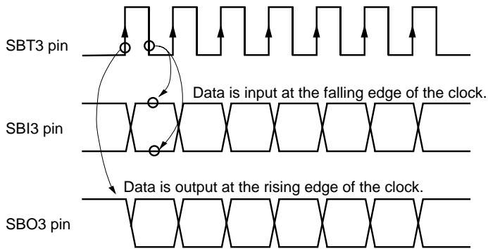
Figure 14-3-11 Transmission/Reception Timing (Reception : Falling edge, Transmission : Rising edge)
