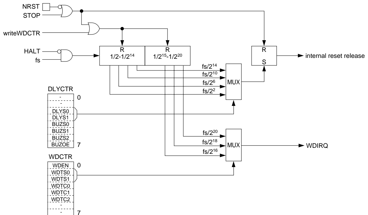
Figure 2-8-3 Block Diagram of Oscillation Stabilization Wait Time (watchdog timer)
