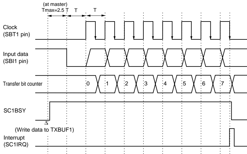
Figure 12-3-10 Reception Timing (falling edge, start condition is enabled)
