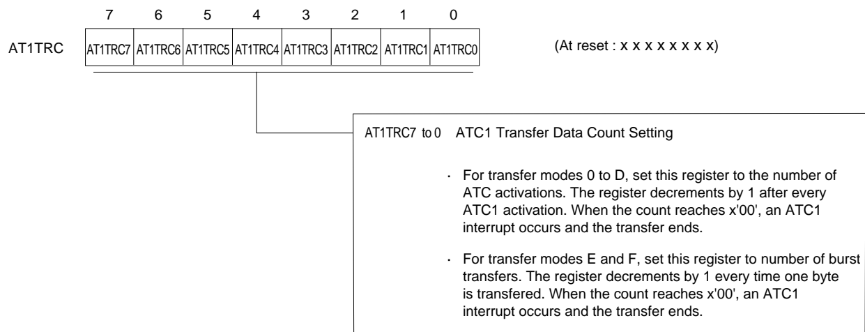
Figure 15-2-3 ATC1 Transfer Data Counter (AT1TRC : x'03FD2', R/W)
