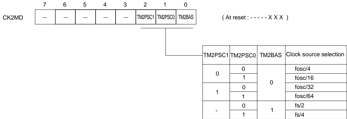
Figure 5-2-4 Timer 2 Prescaler Selection Register (CK2MD : x'03F5E', R/W)
