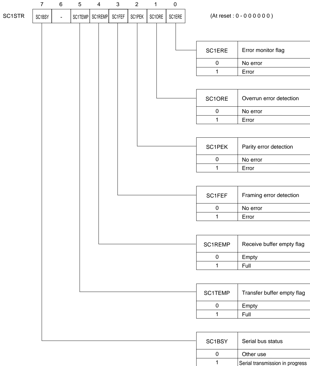
Figure 12-2-6 Serial Interface 1 State Register (SC1STR : x'03F9D', R)
