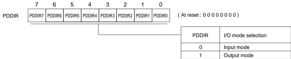
Port D direction control register (PDDIR : x'03F3D', R/W)
