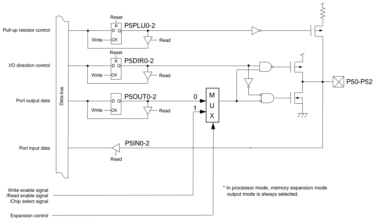
Figure 4-7-3 Block Diagram (P50 to P52)
