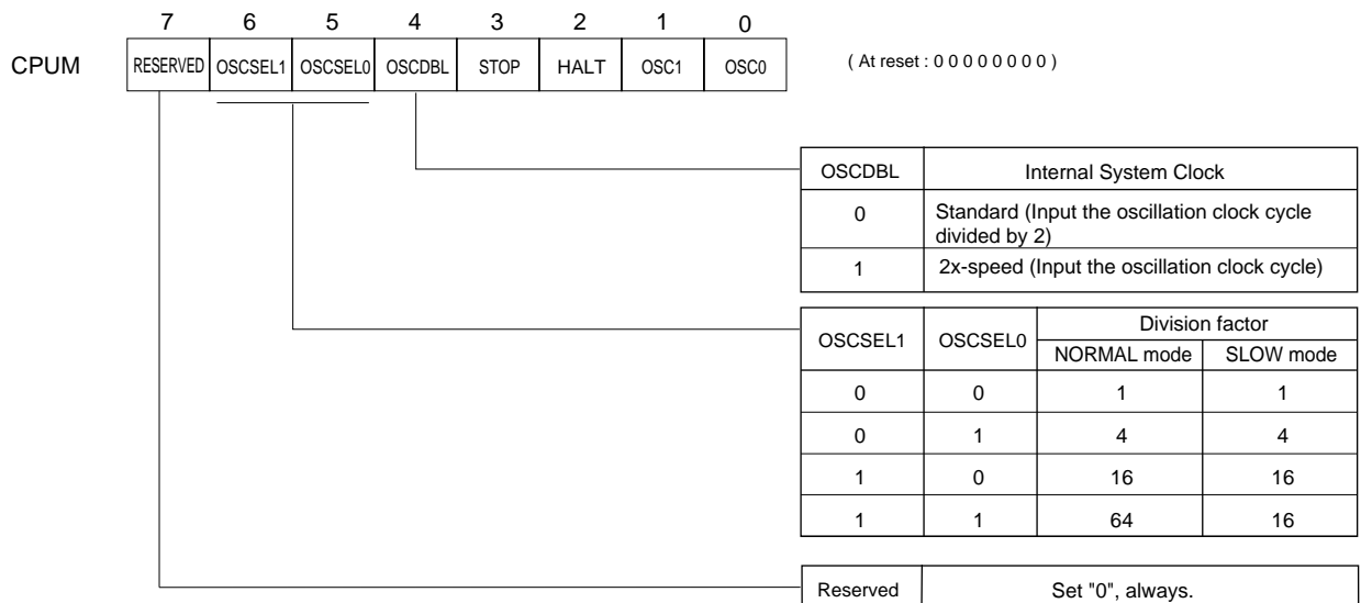
Figure 2-5-2 CPU Mode Control Register (CPUM : x'03F00', R/W)
