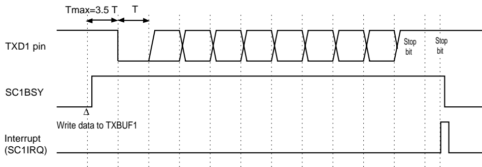
Figure 12-3-16 Transmission Timing (parity bit is disabled)
