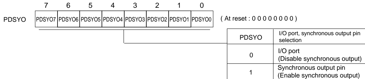
Port D synchronous output control register (PDSYO : x'03F1F', R/W)
