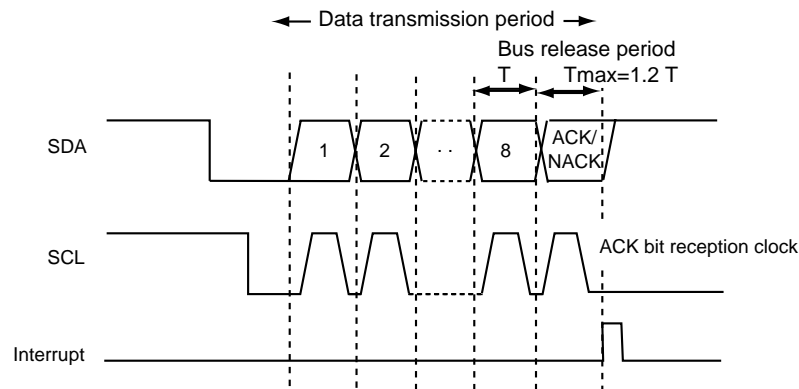
Figure 14-3-13 ACK Bit Reception Timing after Transmission of 8-bit Data
