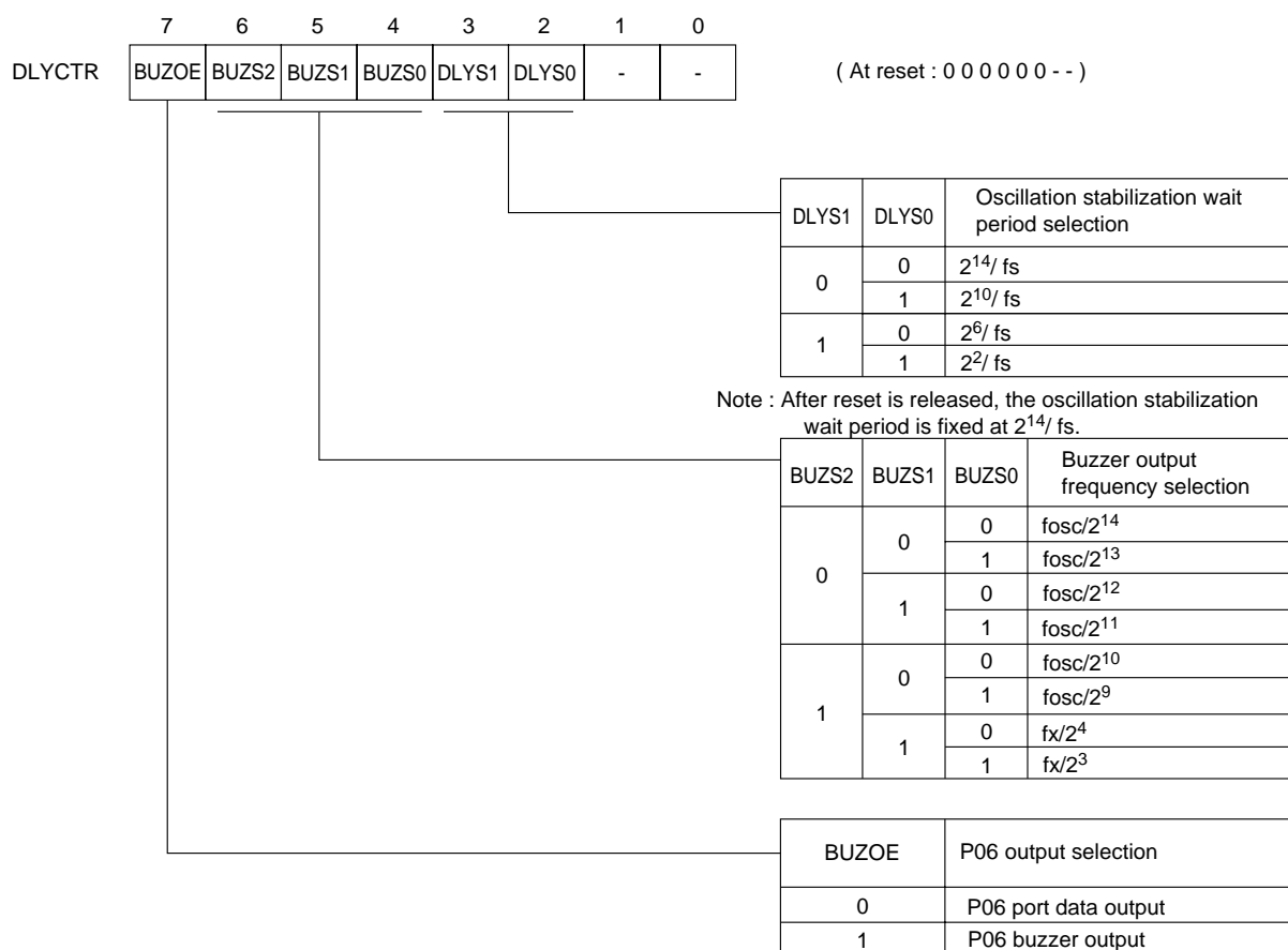
Figure 2-8-4 Oscillation Stabilization Wait Time Control Register (DLYCTR : x'03F03', R/W)
