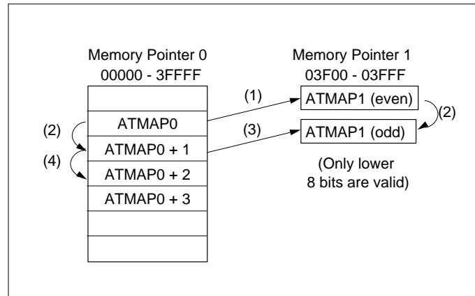
Figure 15-3-6 Transfer Mode 4
