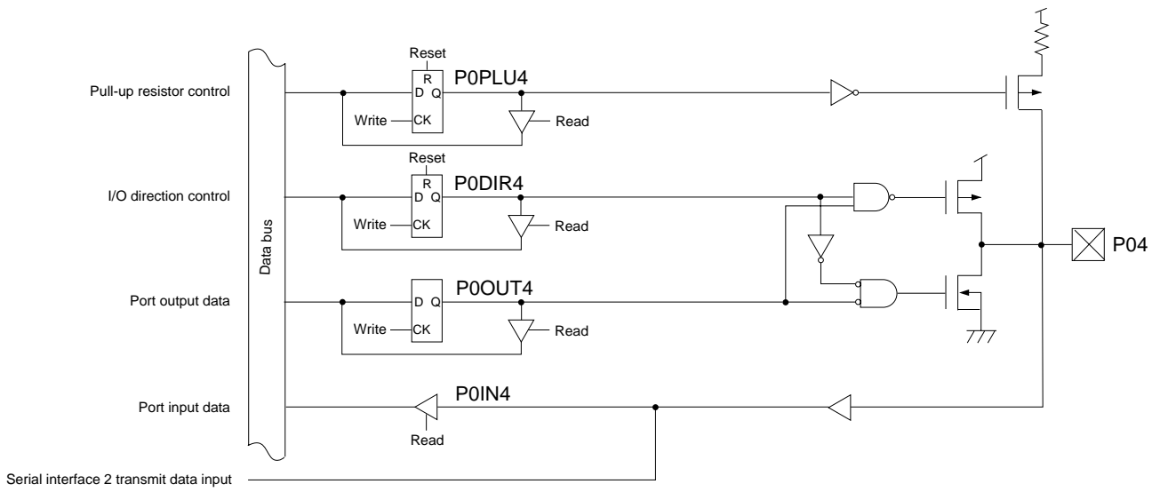
Figure 4-2-6 Block Diagram (P04)
