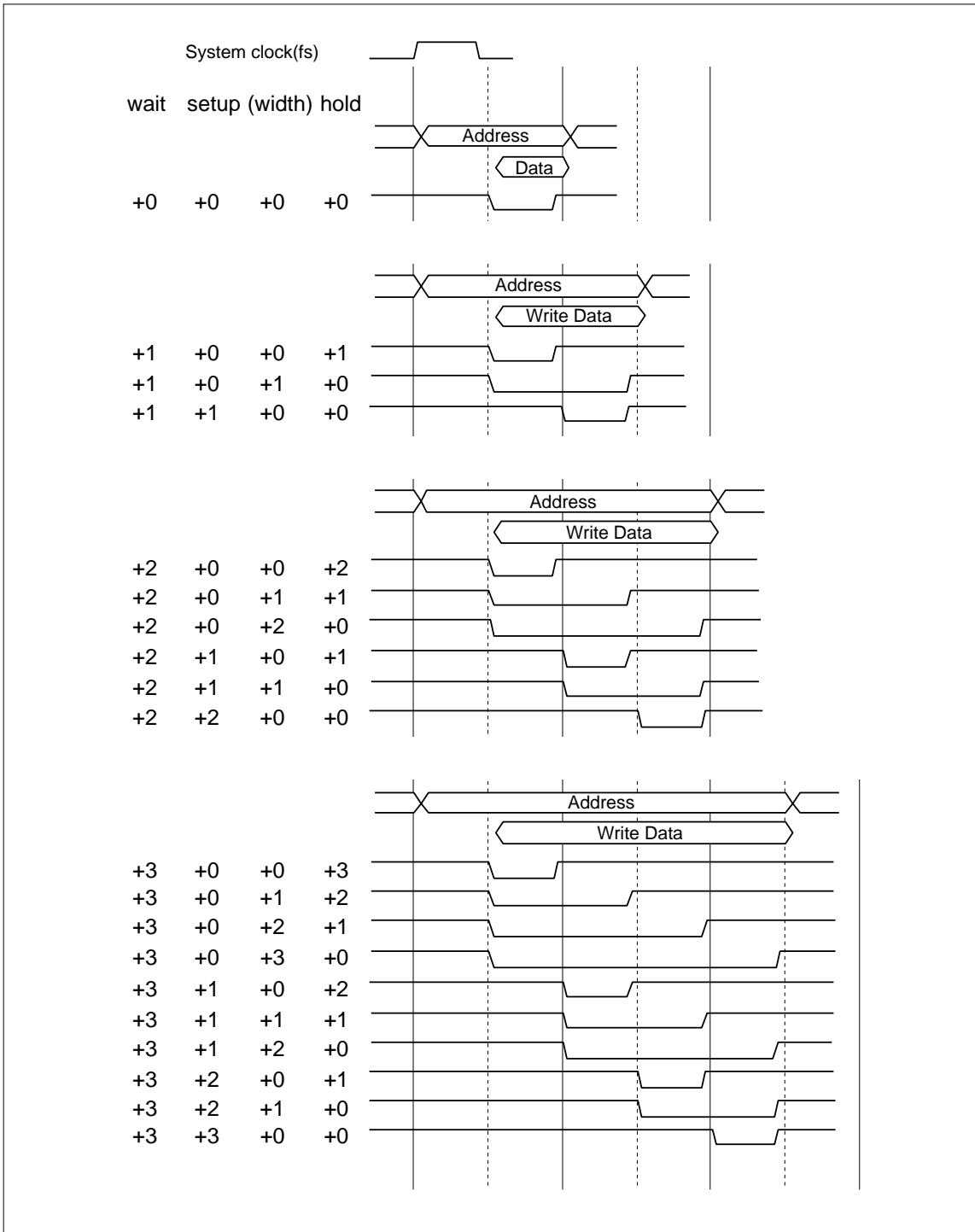
Figure 18-2-1 AC Timing Features of Data Strobe Signal
