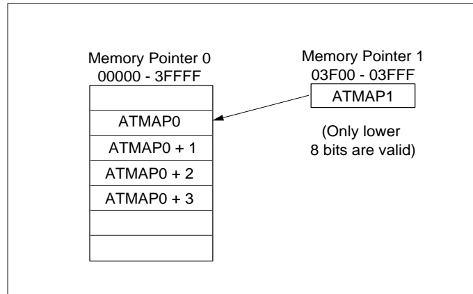
Figure 15-3-3 Transfer Mode 1
