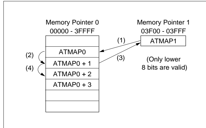
Figure 15-3-8 Transfer Mode 6
