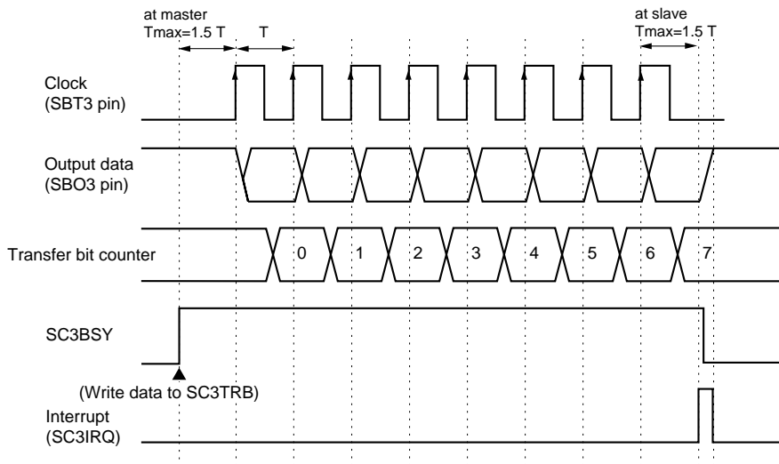
Figure 14-3-5 Transmission Timing (Rising edge, Disable Start Condition)
