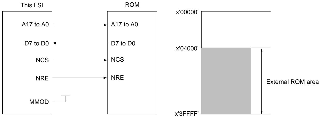
Figure 2-3-6 ROM Connection Example
