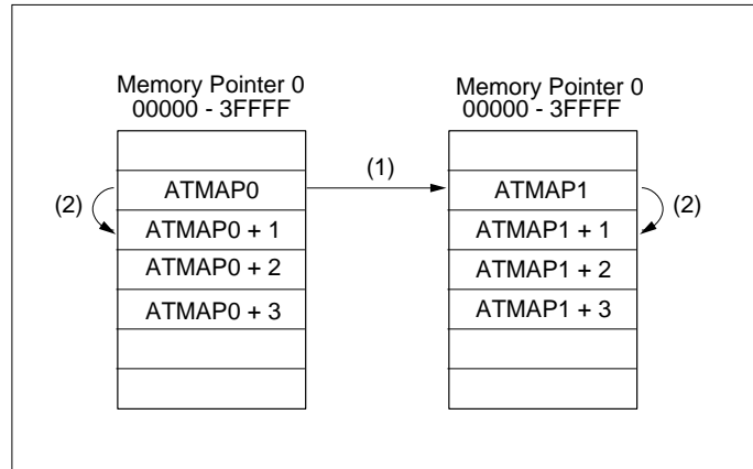
Figure 15-3-14 Transfer Mode C
