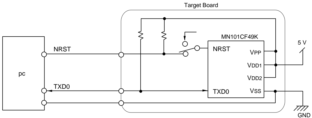
Figure 20-6-1 Target Board for programming with the UART communication using PC
