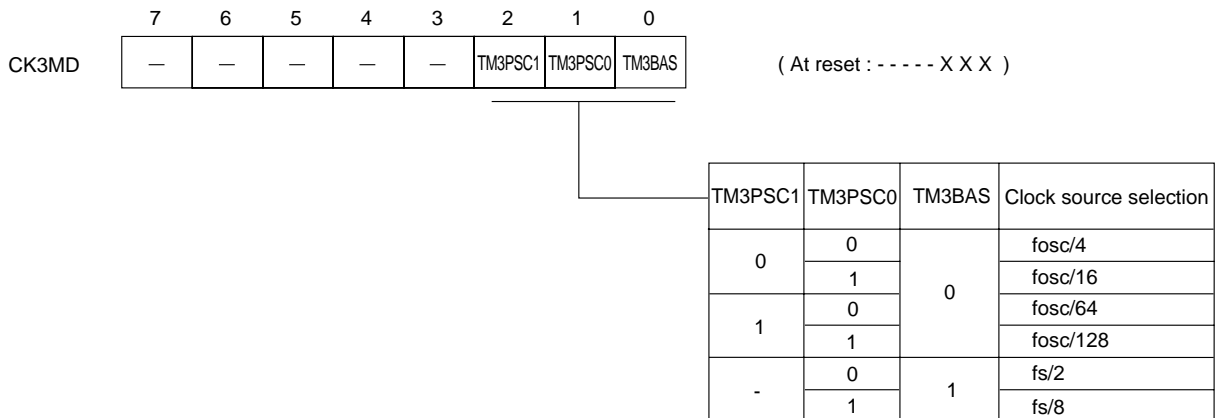
Figure 5-2-5 Timer 3 Prescaler Selection Register (CK3MD : x'03F5F', R/W)
