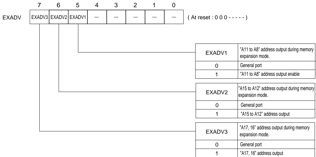
Address output control register (EXADV : x'03F0E', R/W)
