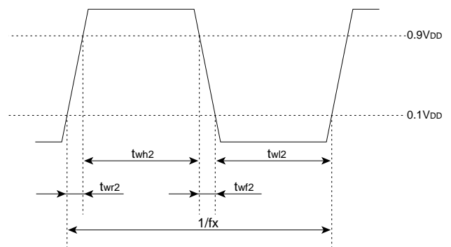
Figure 20-3-4 XI Timing Chart
