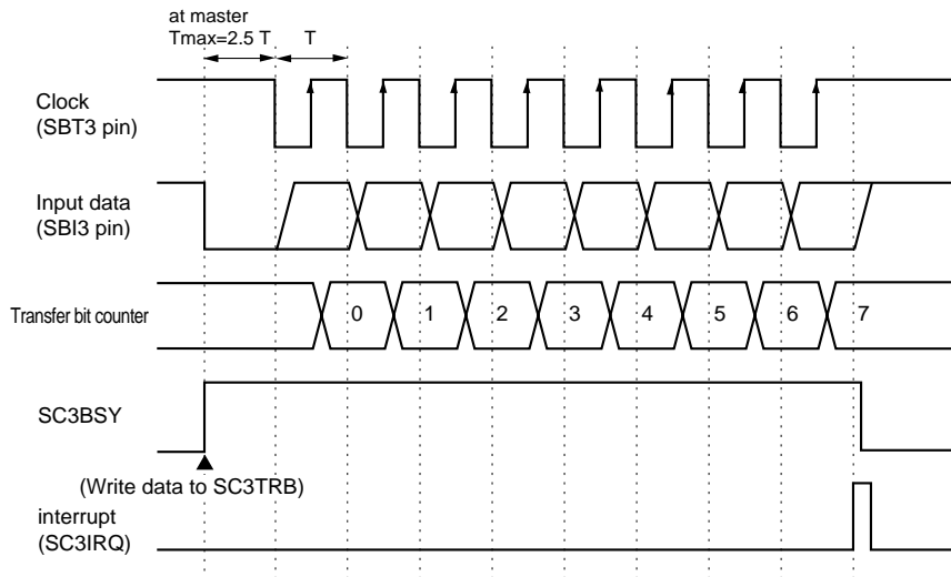
Figure 14-3-6 Reception Timing (Rising edge, Enable Start Condition)
