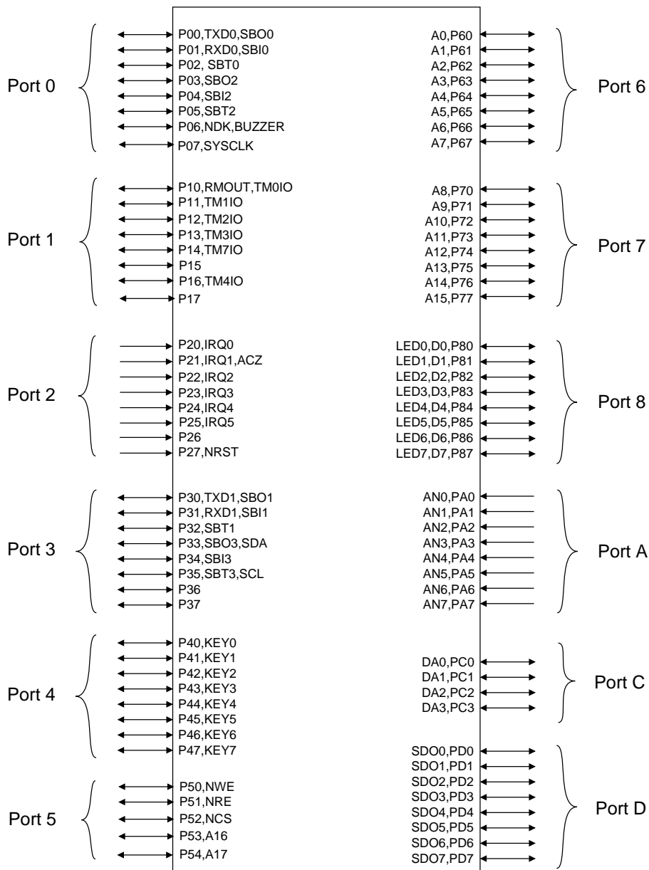
Figure 4-1-1 I/O Port Functions
