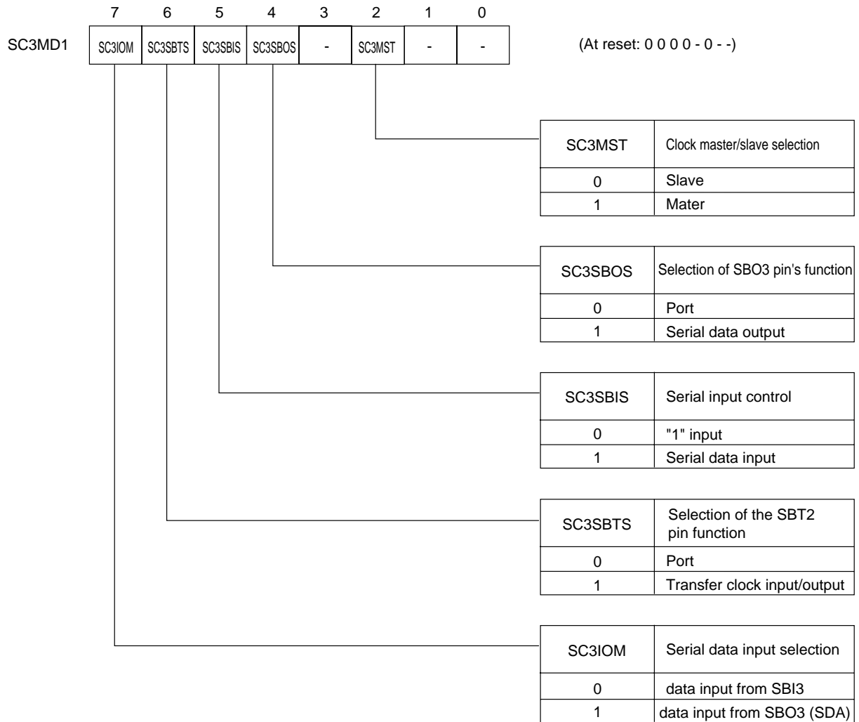
Figure 14-2-3 Serial Interface 3 Mode Register 1 (SC3MD1 : x'03FA9', R/W)
