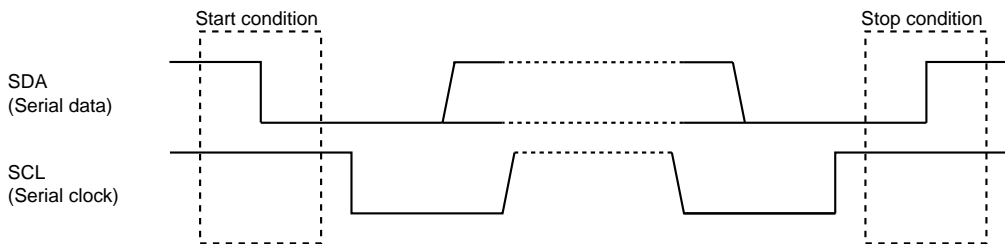
Figure 14-3-12 Start Condition and Stop Condition
