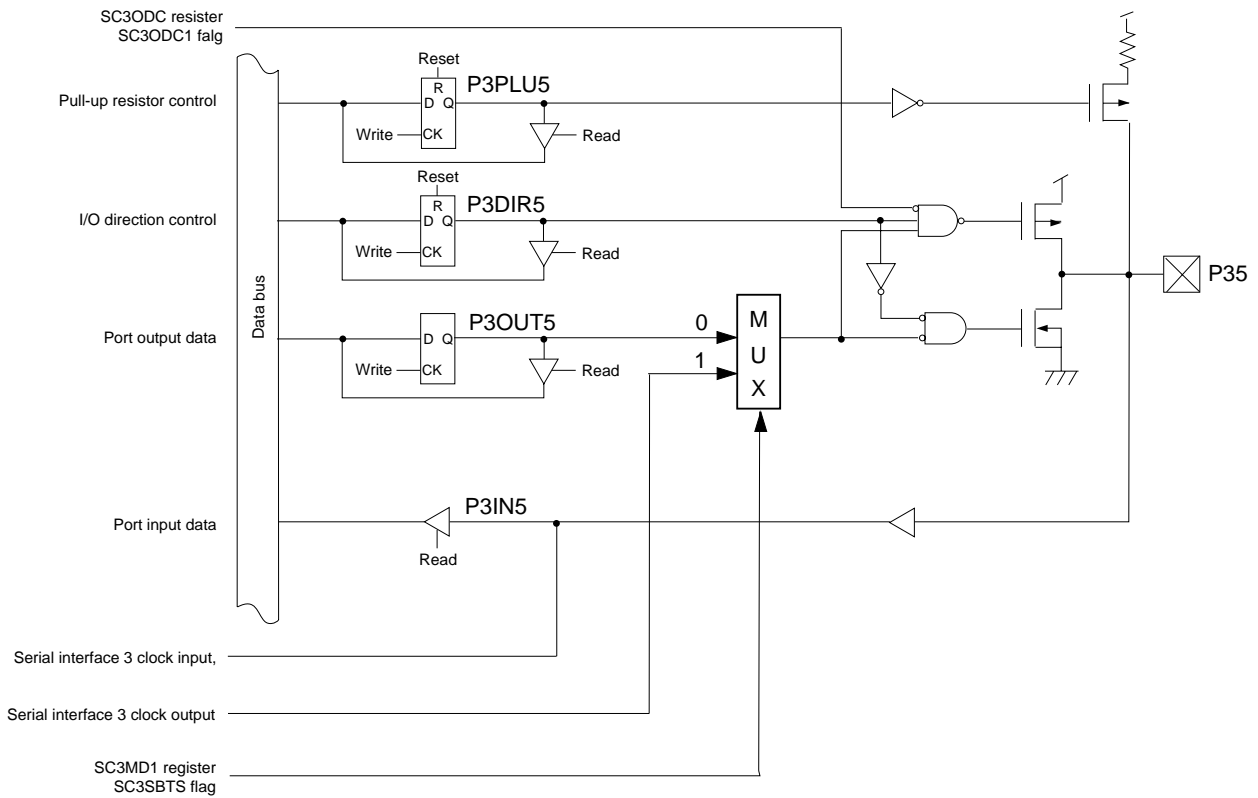
Figure 4-5-7 Block Diagram (P35)
