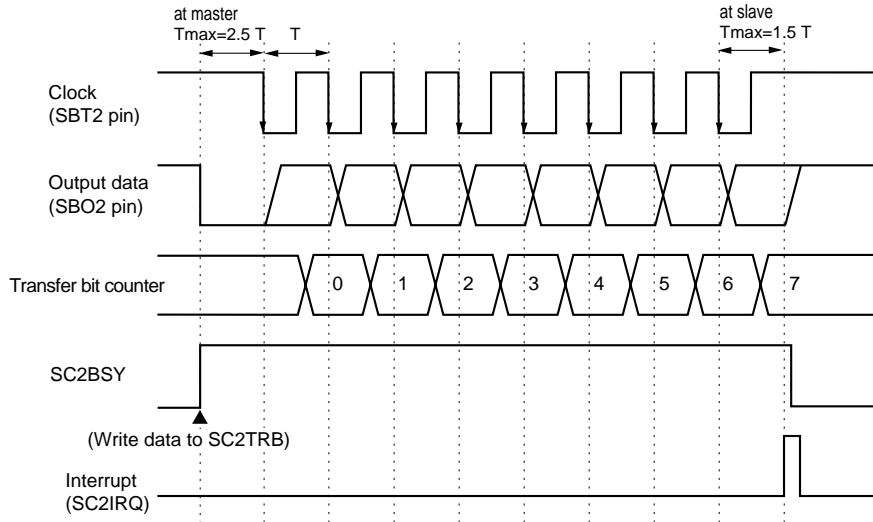
Figure 13-3-2 Transmission Timing (Falling edge, Start condition is enabled)
