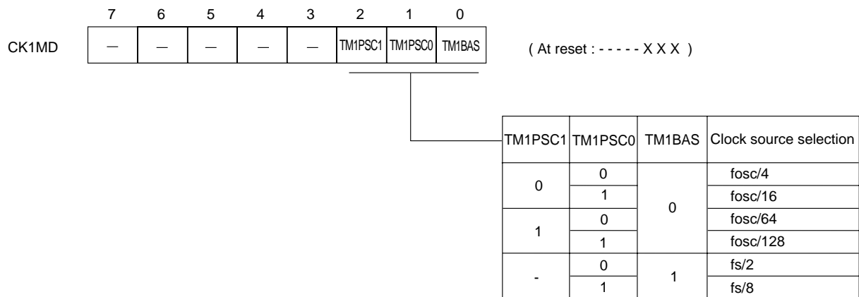
Figure 5-2-3 Timer 1 Prescaler Selection Register (CK1MD : x'03F57', R/W)
