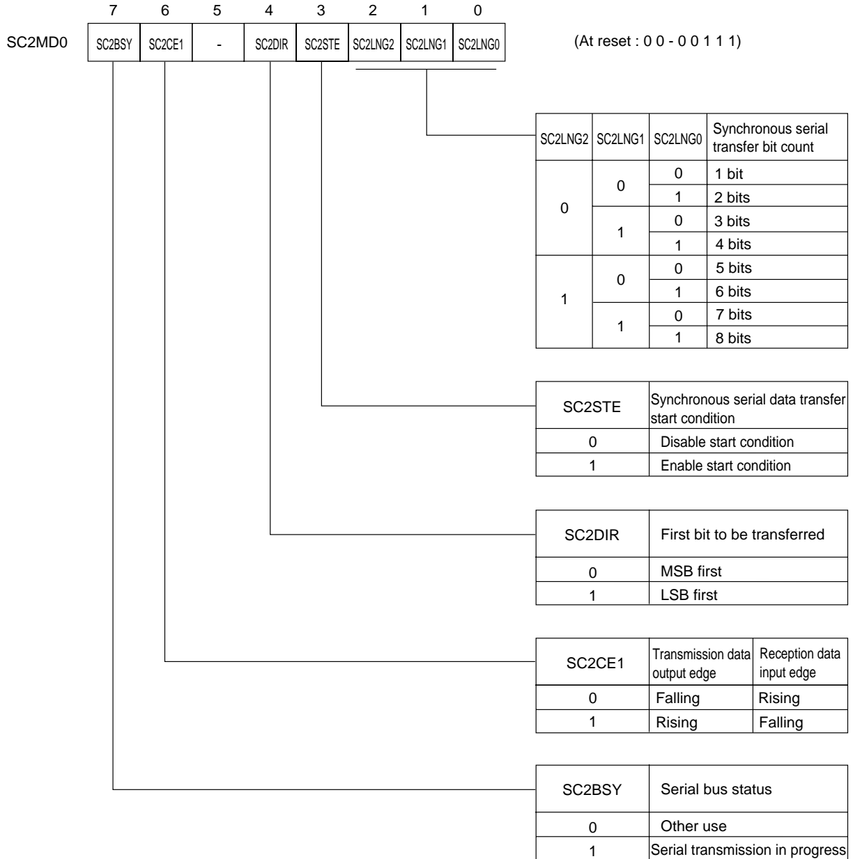
Figure 13-2-2 Serial Interface 2 Mode Register 0 (SC2MD0 : x'03FA0', R/W)
