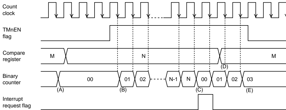
Figure 6-3-1 Count Timing of Timer Operation (Timers 0, 1, 2, 3 and 4)
