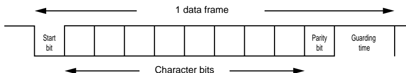
Figure 12-3-21 Communication Data Format (T=0, 1)
