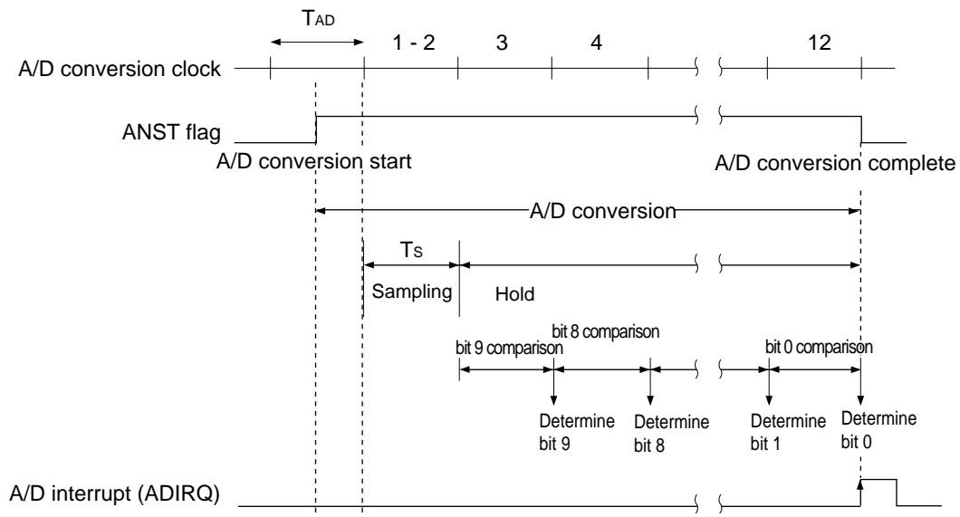
Figure 16-3-1 Operation of A/D Conversion
