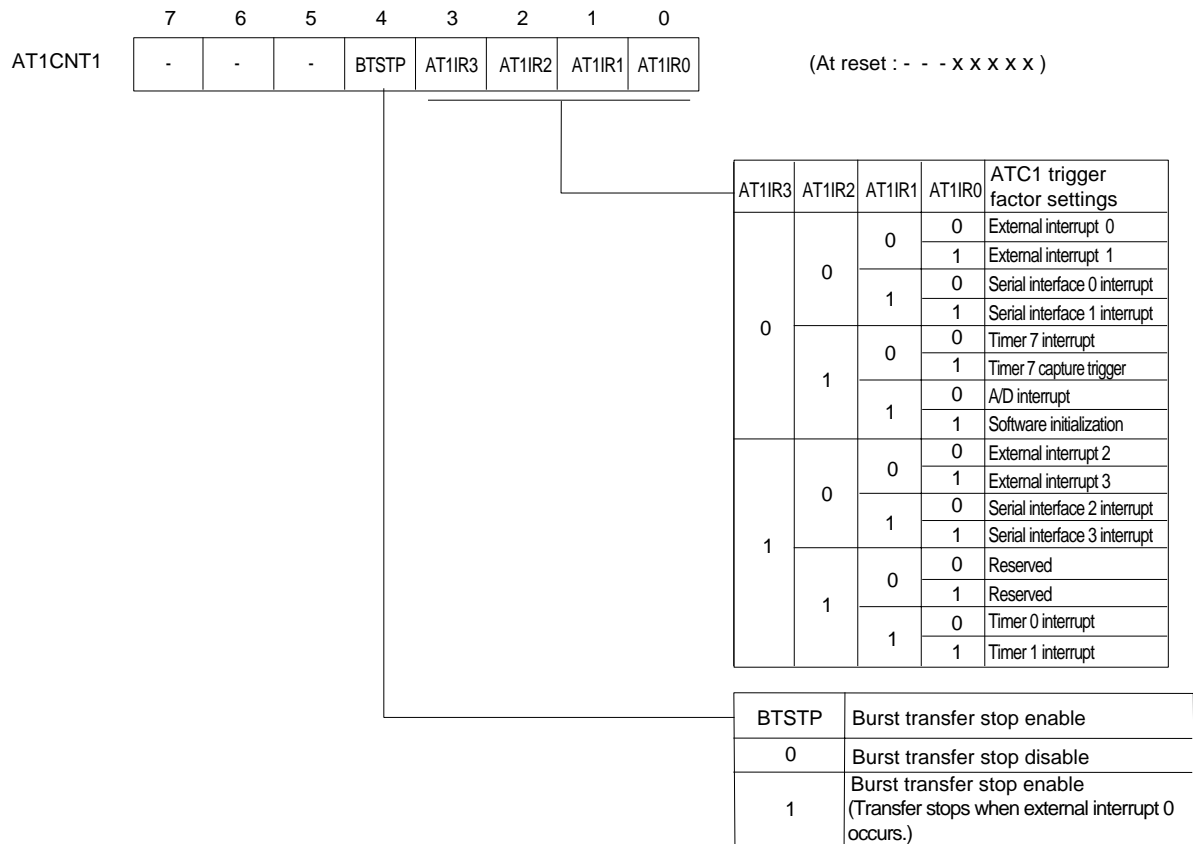
Figure 15-2-2 ATC1 Control Register 1 (AT1CNT1 : x'03FD1', R/W)
