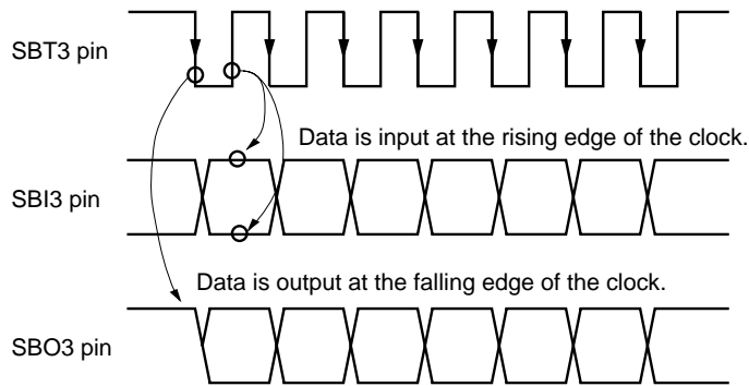
Figure 14-3-10 Transmission/Reception Timing (Reception : Rising edge, Transmission : Falling edge)
