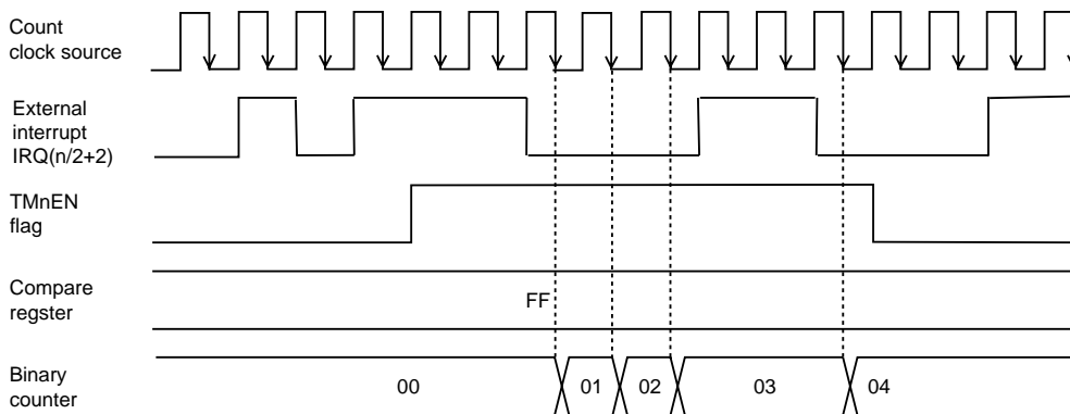
Figure 6-9-1 Count Timing at Measurement of Simple Pulse Width (Timer 0, Timer 2, Timer 4)
