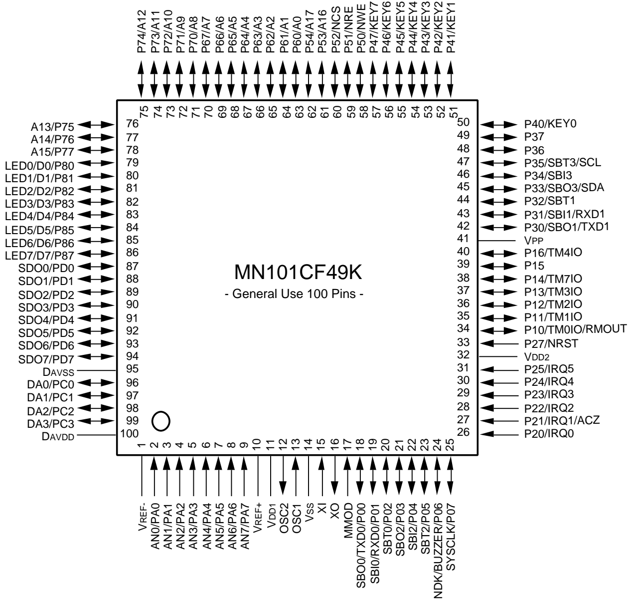
Figure20-2-1 Pin Configuration ( 100QFP : Top view )
