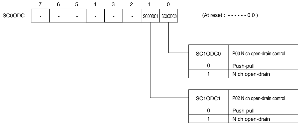
Figure 11-2-7 Serial Interface 0 Port Control Register (SC0ODC : x'03F96', R/W)
