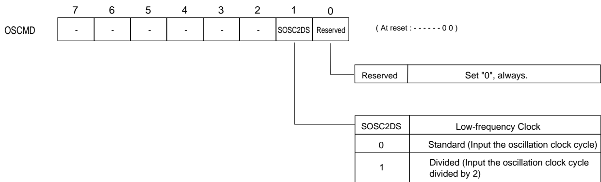
Figure 2-5-1 Oscillator Frequency Control Register (OSCMD : x'03F0D', R/W)
