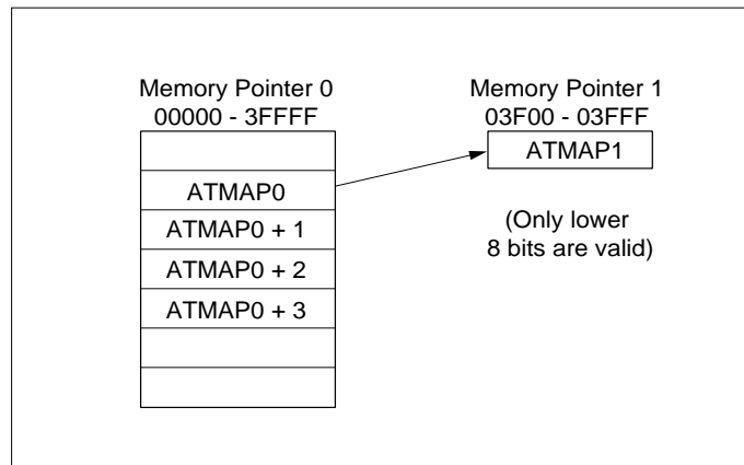
Figure 15-3-2 Transfer Mode 0
