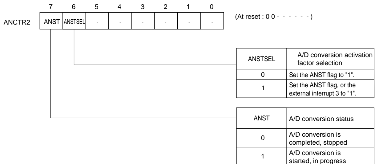
Figure 16-2-3 A/D Converter Control Register 2 (ANCTR2 : x'03FB2', R/W)
