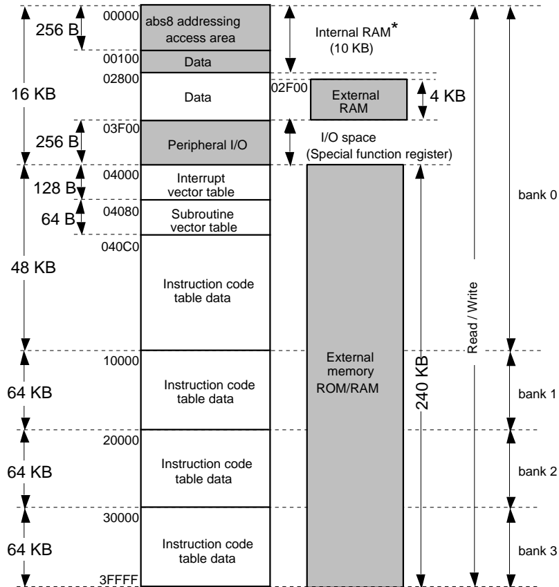
Figure 2-6-5 Processor Mode
