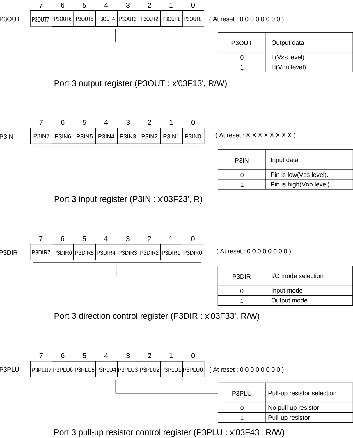
Figure 4-5-1 Port 3 Registers
