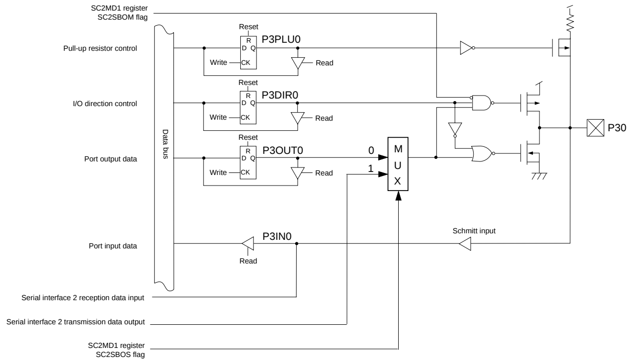
Figure 4-5-2 Block diagram (P30)
