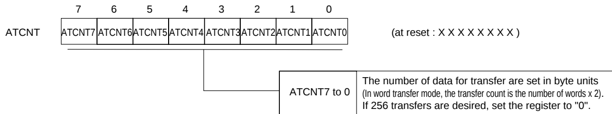
Figure 13-2-2 Transfer Data Counter (ATCNT : x'03FA1', R/W)
