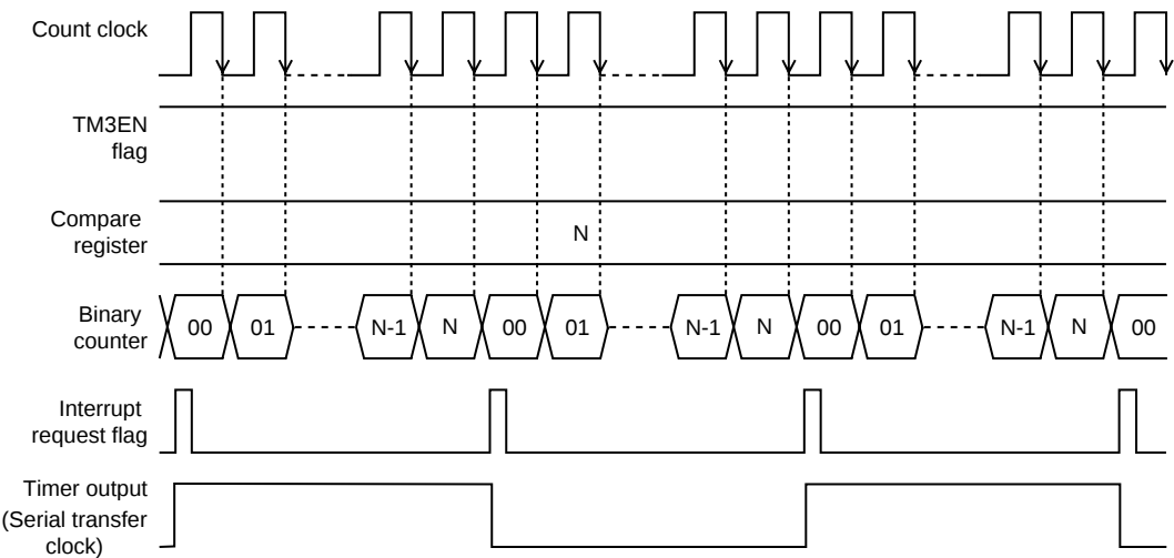
Figure 5-8-1 Timing of Serial Interface Transfer Clock (Timer 0 and Timer 3)
