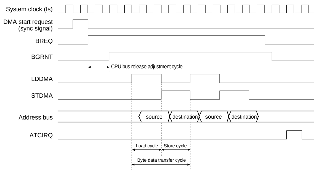
Figure 13-3-1 ATC Timing Chart
