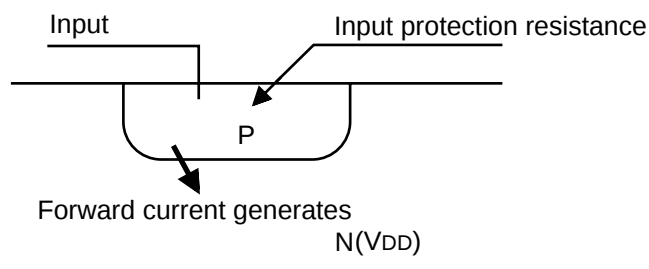
Figure 1-7-5 Power Supply and Input Pin Voltage
