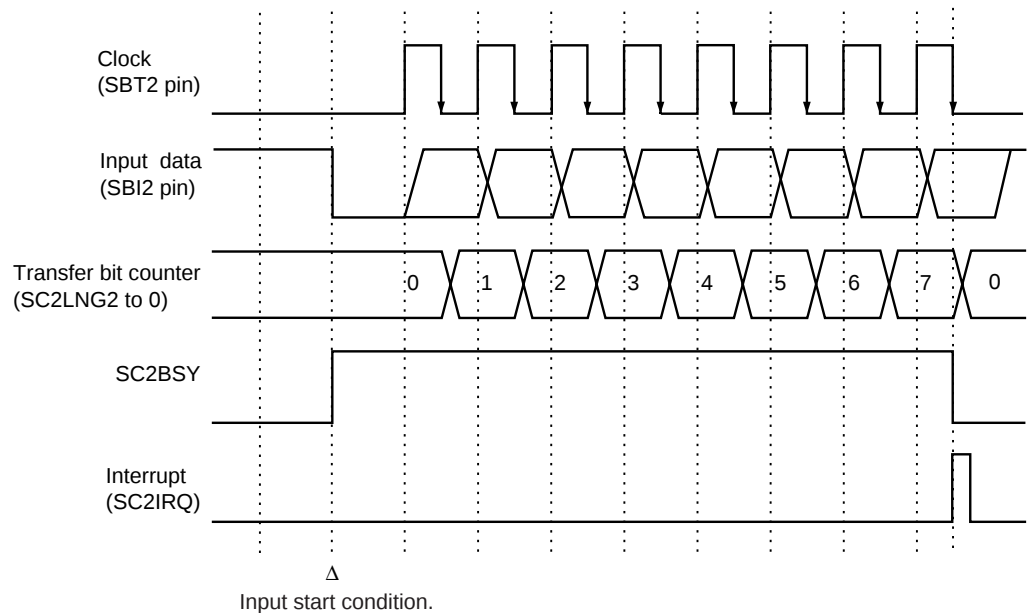
Figure 12-3-6 Reception Timing (falling edge, start condition is enabled)
