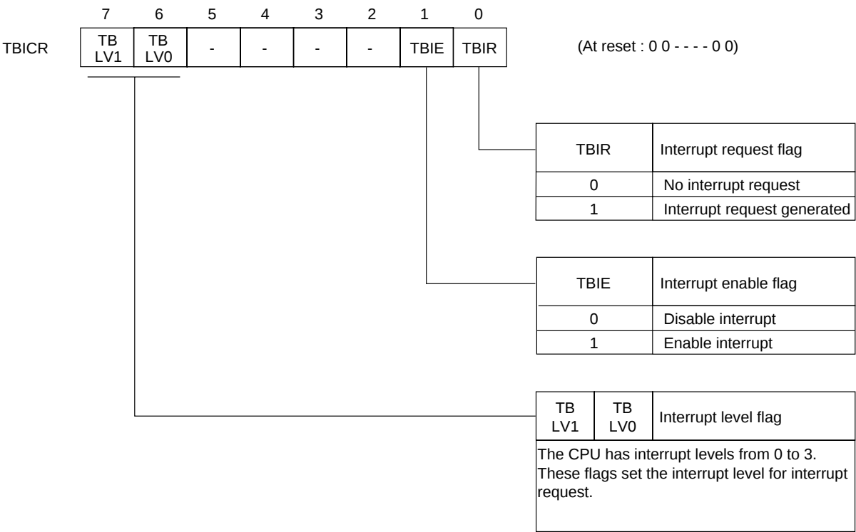
Figure 3-2-13 Time Base Interrupt Control Register (TBICR : x'03FE7', R/W)
