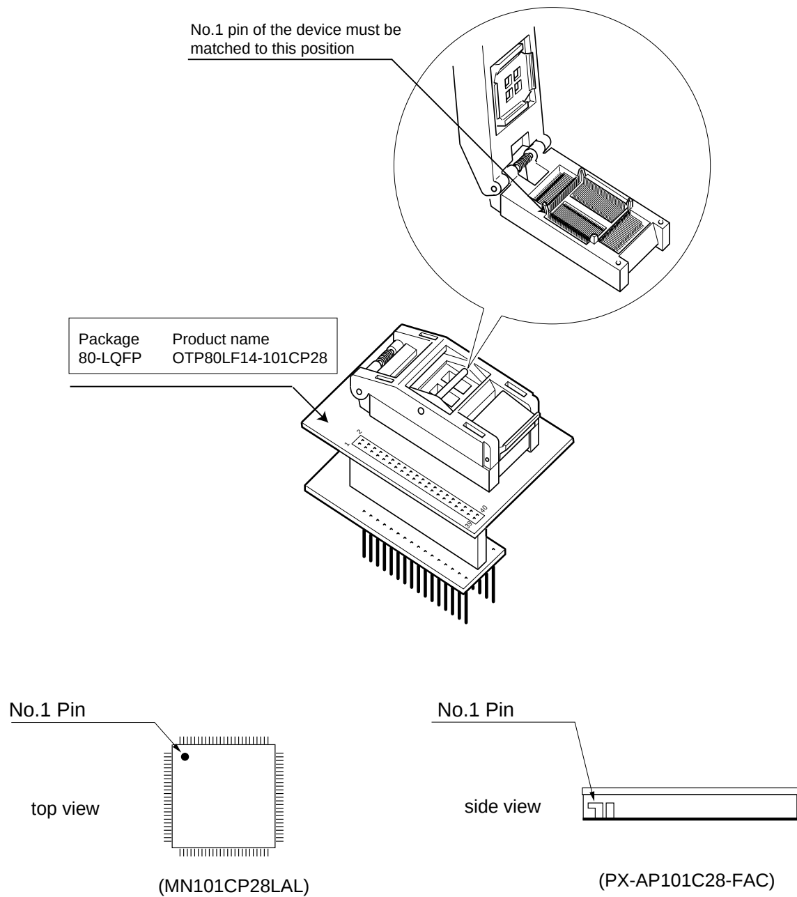
Figure 15-1-1 Mounting a Device in Programming Adapter and the Position of No.1 Pin
