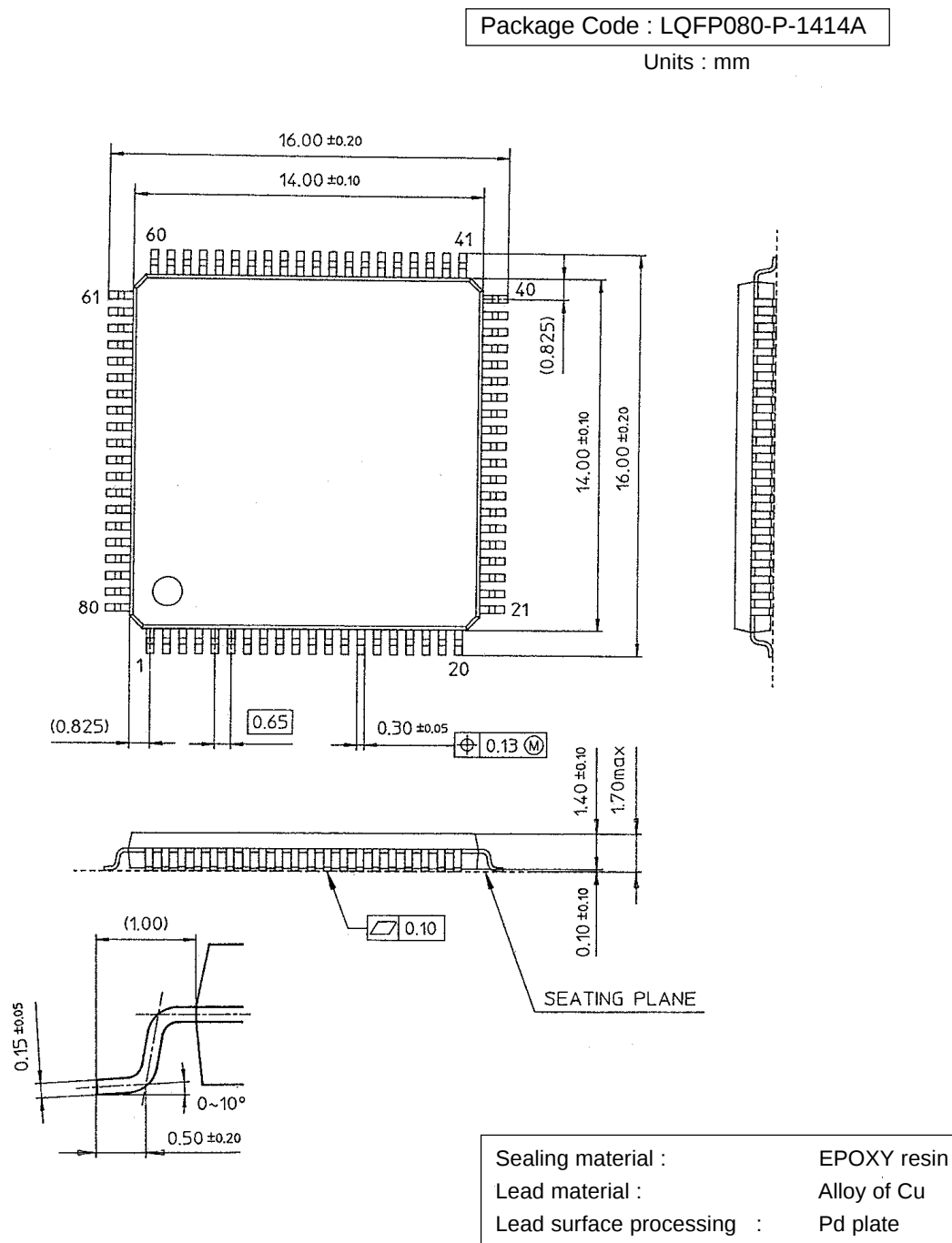
Figure 1-6-1 80-Pin LQFP
