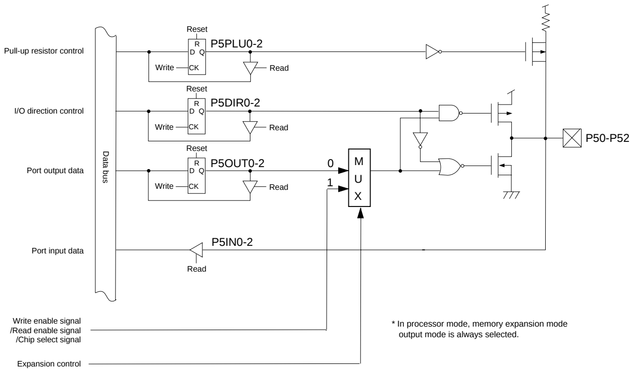
Figure 4-7-3 Block Diagram (P50 to P52)
