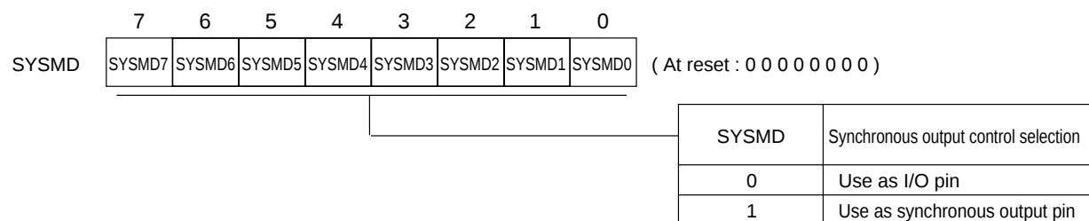
Synchronous output control register (SYSMD : X'03F1F', R/W)
