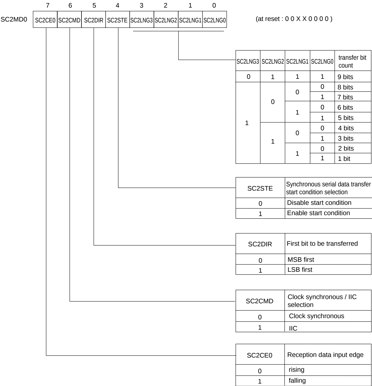
Figure 12-2-2 Serial Interface 2 Mode Register 0 (SC2MD0 : x'03F5A', R/W)
