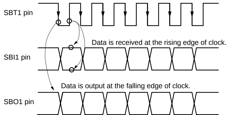
Figure 11-3-9 Transmission / Reception Timing (Reception : at rising edge, Transmission : at falling edge) (SC1CE0=0, SC1CE1=0)
