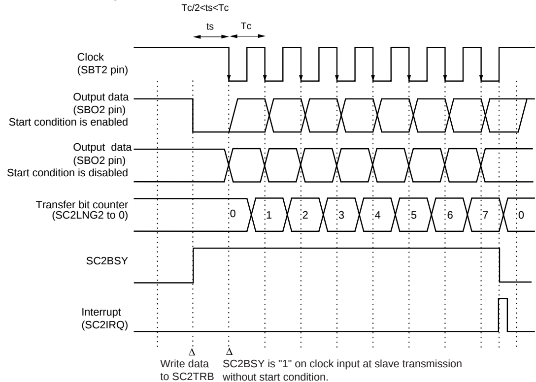
Figure 12-3-3 Transmission Timing (falling edge)
