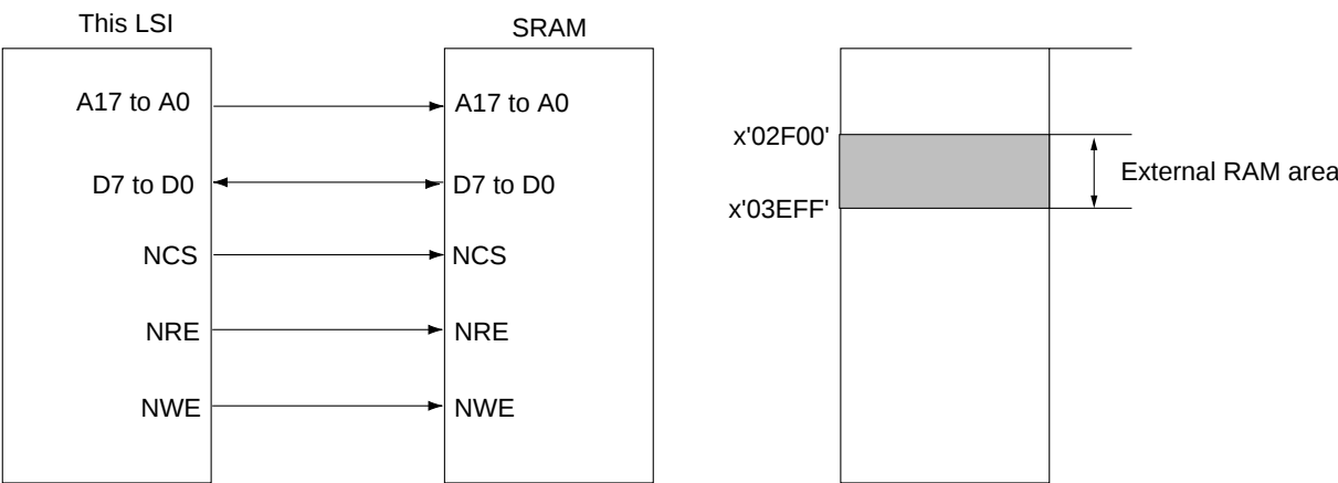
Figure 2-3-7 SRAM Connection Example
