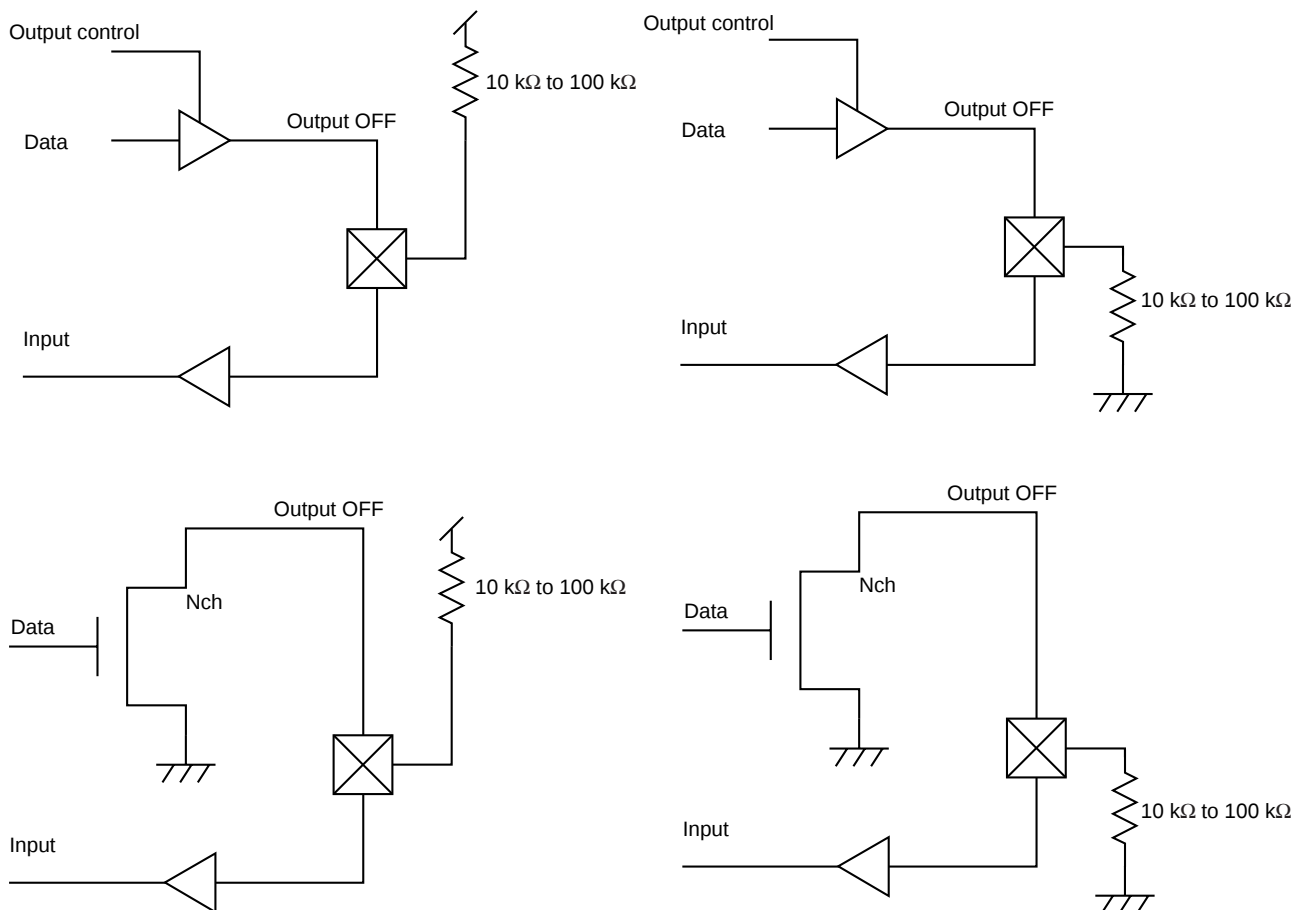
Figure 1-7-4 Unused I/O pins (high impedance output at reset)
