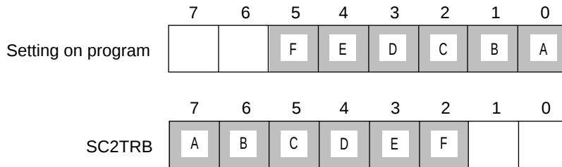
Figure 12-3-1-2 Transfer Bit Count and First Transfer Bit (starting with LSB)
