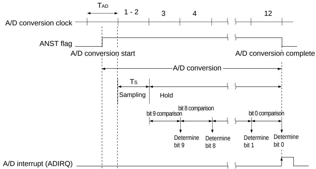
Figure 14-3-1 Operation of A/D Conversion
