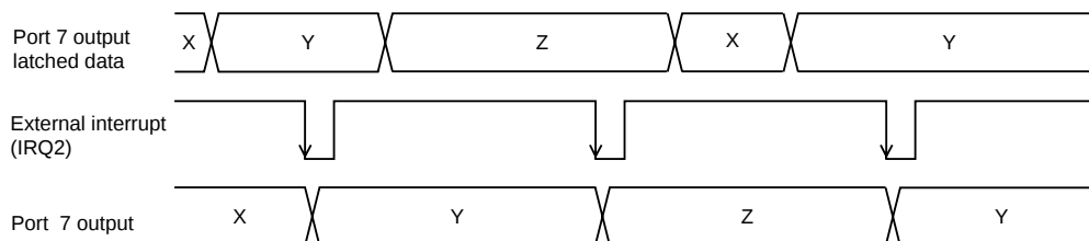
Figure 4-12-2 Synchronous Output Timing by Event Generation (IRQ2)
