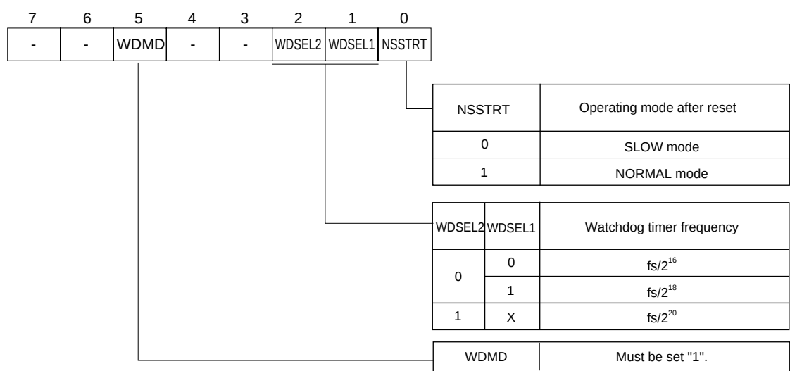
Figure 15-1-3 EPROM Option Bits
