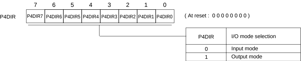
Port 4 direction control register (P4DIR : x'03F34', R/W)
