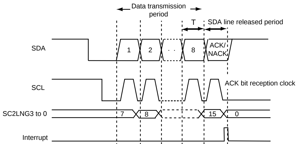
Figure 12-3-10 ACK Bit Reception Timing after Transmission of 8-Bit Data
