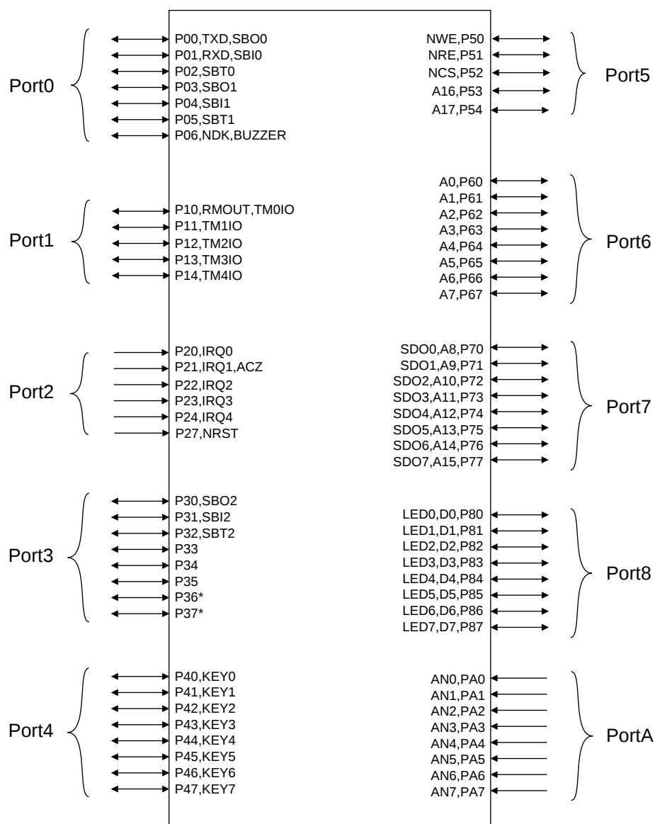
Figure 4-1-1 I/O Port Functions
