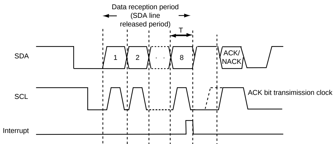
Figure 12-3-11 ACK Bit Transmission Timing after Reception of 8-Bit Data
