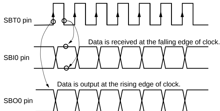
Figure 10-3-10 Transmission / Reception Timing (Reception : falling edge, Transmission : rising edge) (SC0CE0 = 0, SC0CE1 = 1)
