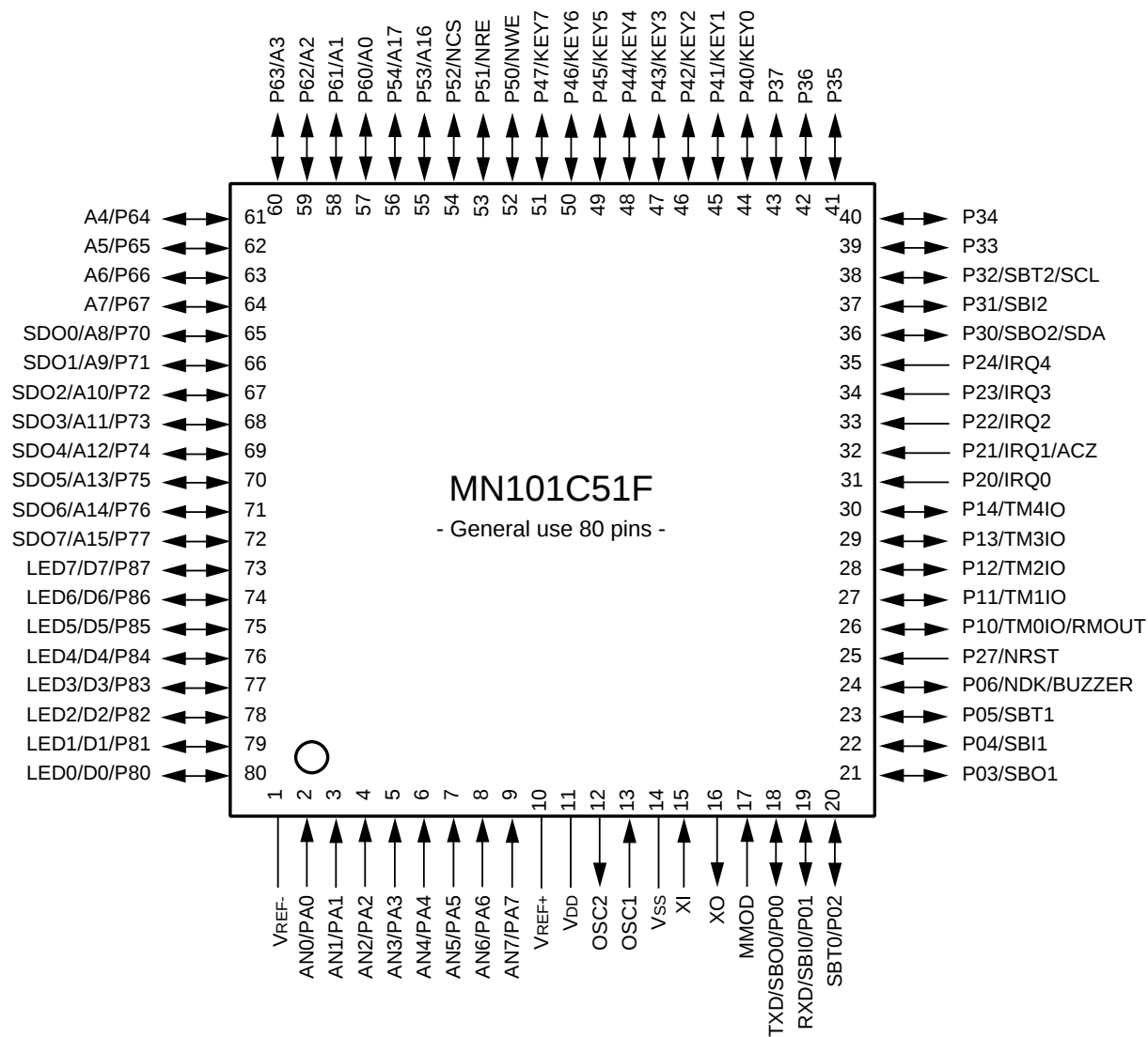
Figure 1-3-1 Pin Configuration ( 80LQFP : Top view )
