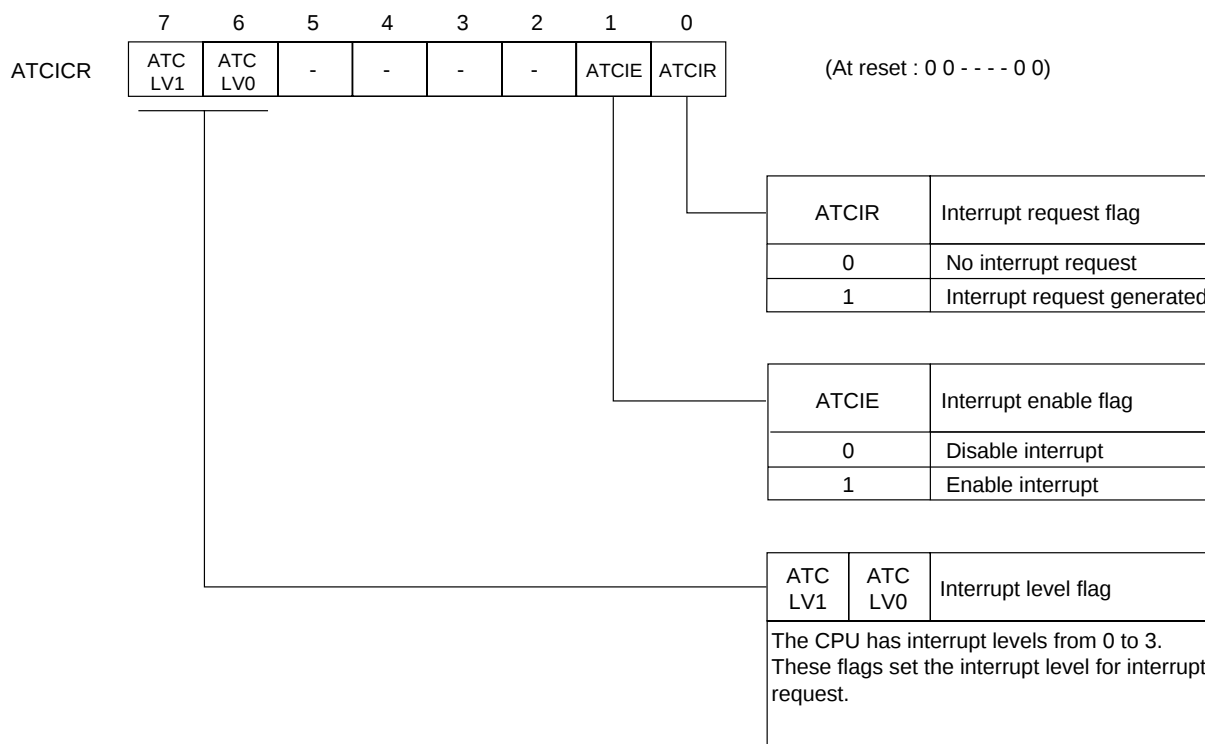
Figure 3-2-18 ATC Interrupt Control Register (ATCICR : x'03FE9', R/W)
