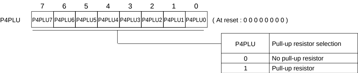
Port 4 pull-up resistor control register (P4PLU : x'03F44', R/W)
