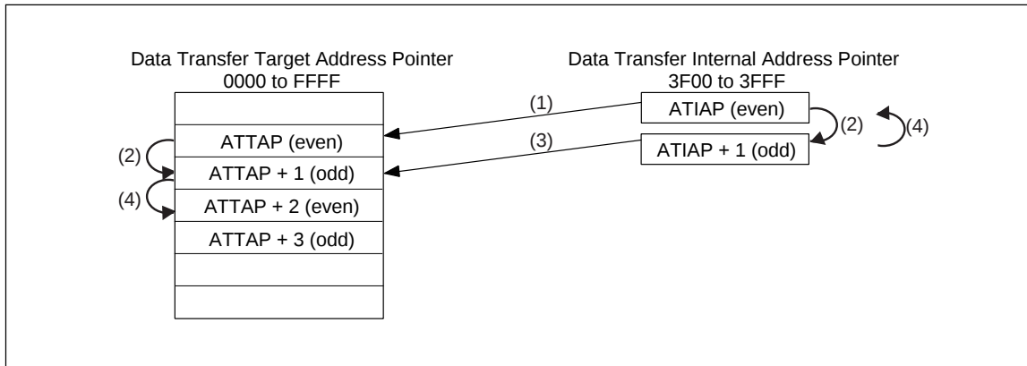
Figure 13-3-9 Transfer Mode 7
