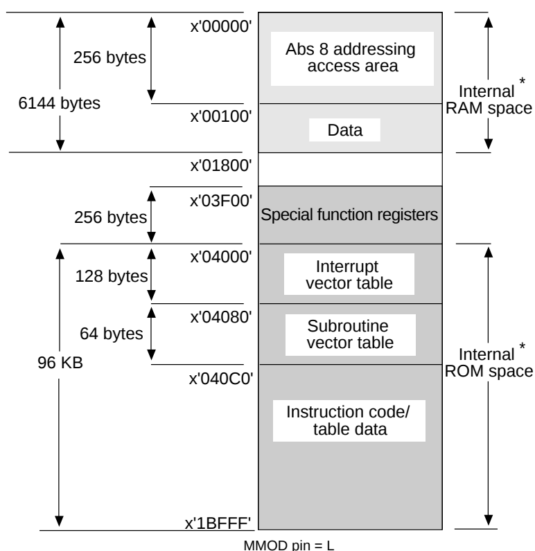
Figure 2-2-1 Single-chip Mode
