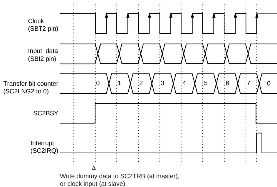
Figure 12-3-5 Reception Timing (rising edge, start condition is disabled)
