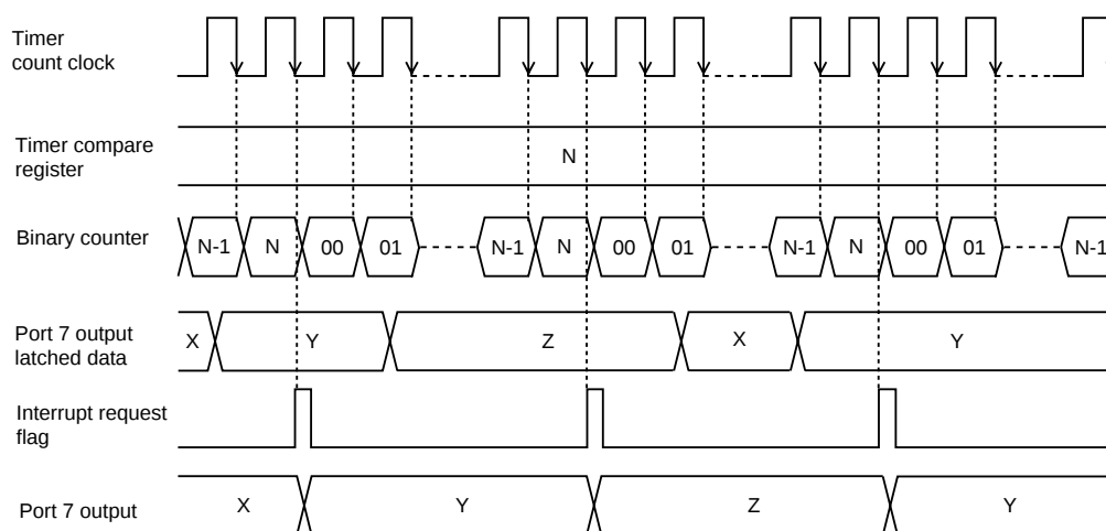
Figure 4-12-3 Synchronous Output Timing by Event Generation (Timers 1, 2 and 4)
