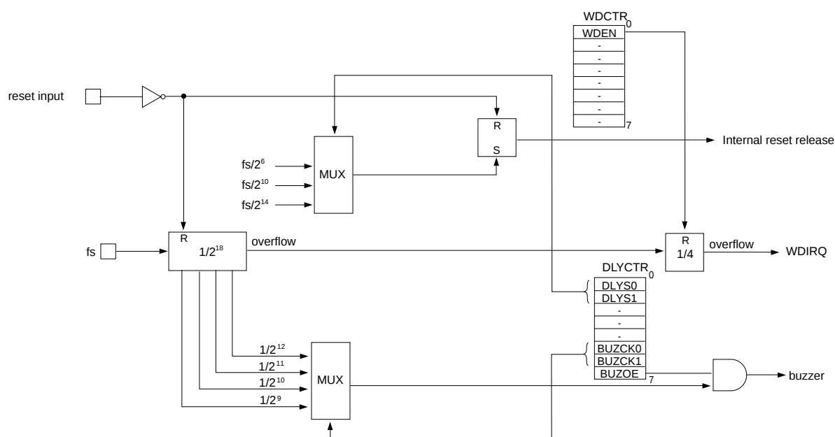
Figure 2-5-3 Block Diagram of Oscillation Stabilization Wait Time (watchdog timer)
