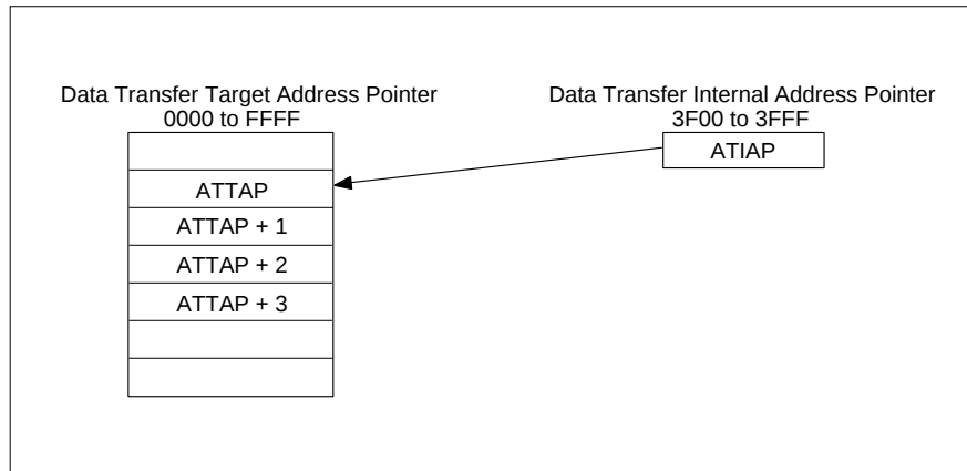
Figure 13-3-3 Transfer Mode 1
