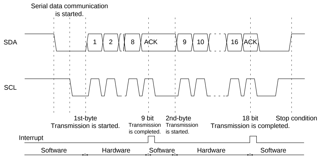
Figure 12-3-13 Master Transmission Timing
