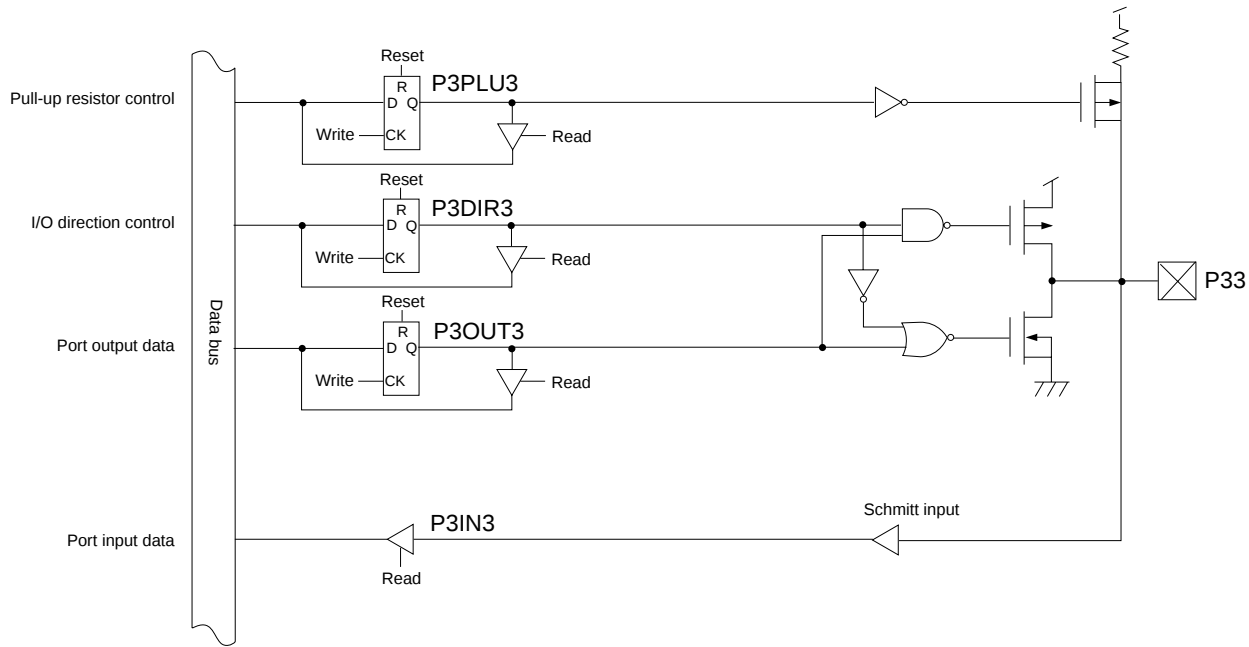
Figure 4-5-5 Block diagram (P33)
