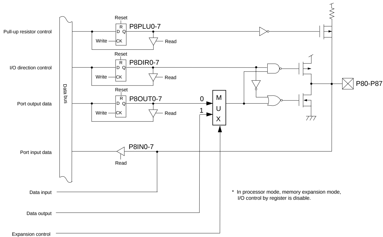
Figure 4-10-2 Block Diagram (P80 to P87)
