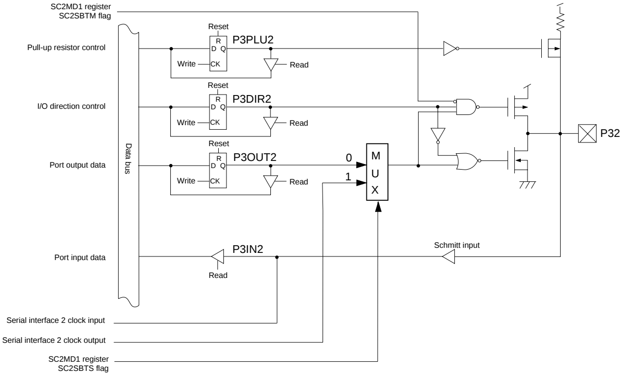
Figure 4-5-4 Block diagram (P32)
