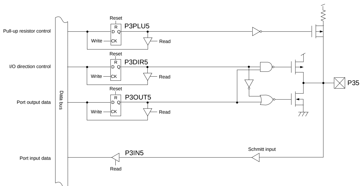
Figure 4-5-7 Block Diagram (P35)
