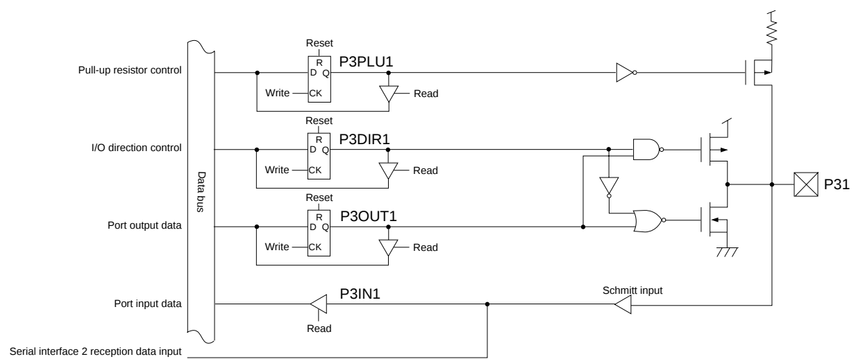
Figure 4-5-3 Block diagram (P31)
