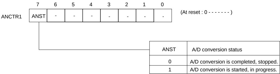
Figure 14-2-2 A/D Converter Control Register 1 (ANCTR1 : x'03F91', R/W)
