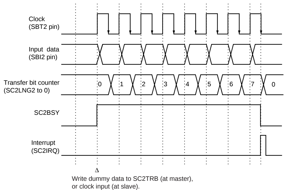
Figure 12-3-7 Reception Timing (falling edge, start condition is disabled)
