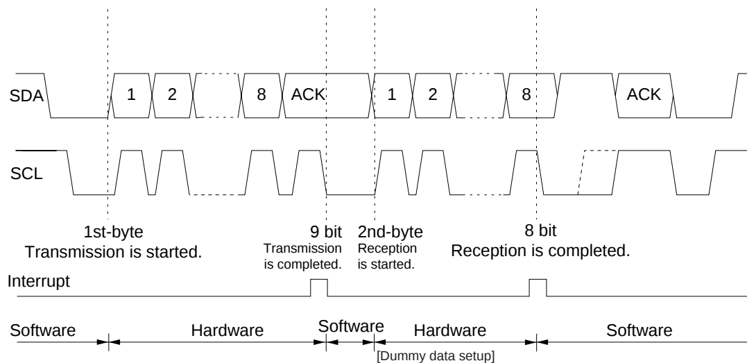
Figure 12-3-14 Master Reception Timing
