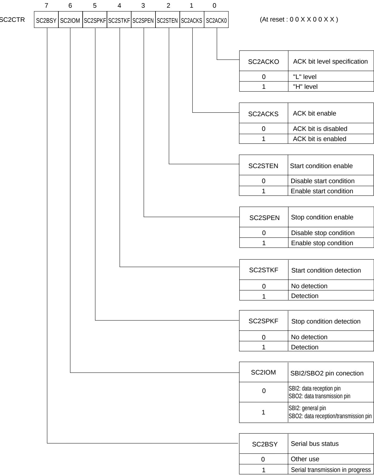
Figure 12-2-4 Serial Interface 2 Control Register (SC2CTR : x'03F5C', R/W)
