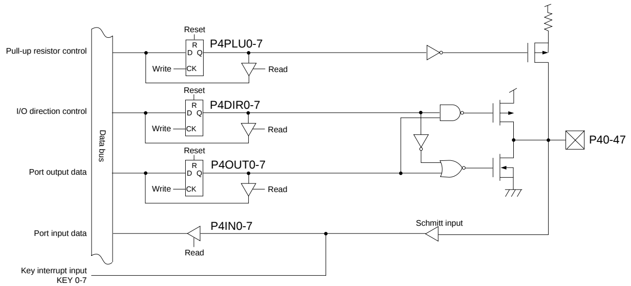
Figure 4-6-3 Block diagram (P40 to P47)
