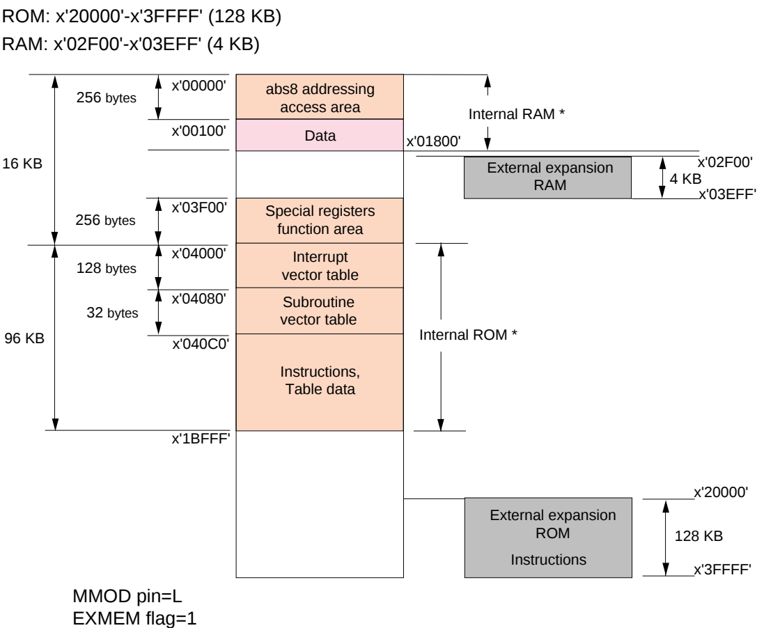
Figure 2-2-2 Memory Expansion Mode
