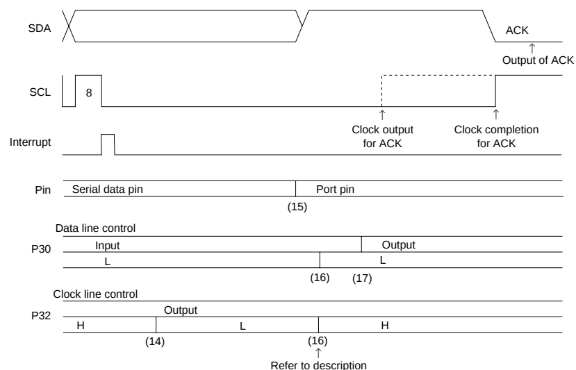
Figure 12-3-15 ACK Processing at Reception
