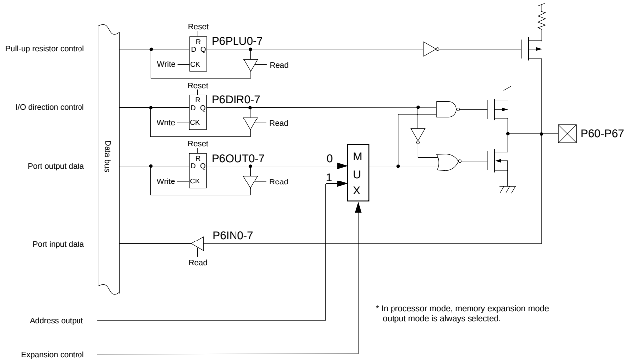
Figure 4-8-2 Block Diagram (P60 to P67)
