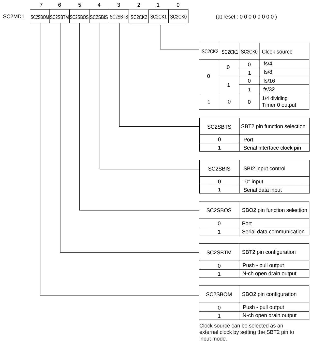
Figure 12-2-3 Serial Interface 2 Mode Register 1 (SC2MD1 : x'03F5B', R/W)
