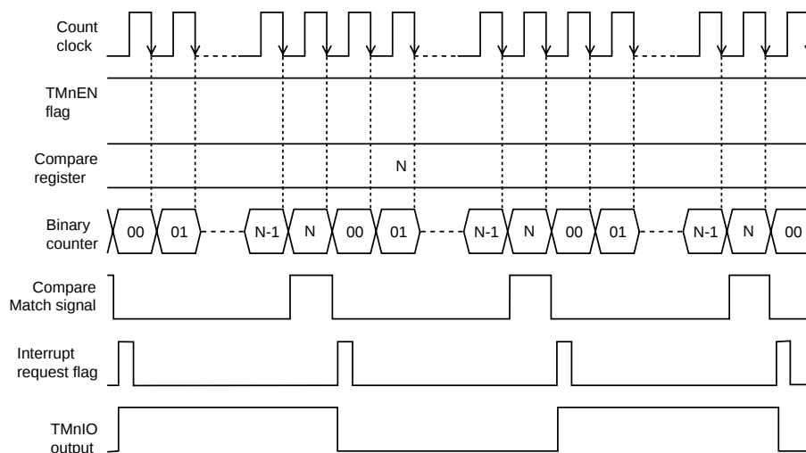
Figure 5-5-1 Count Timing of Timer Pulse Output (Timers 0 to 3)
