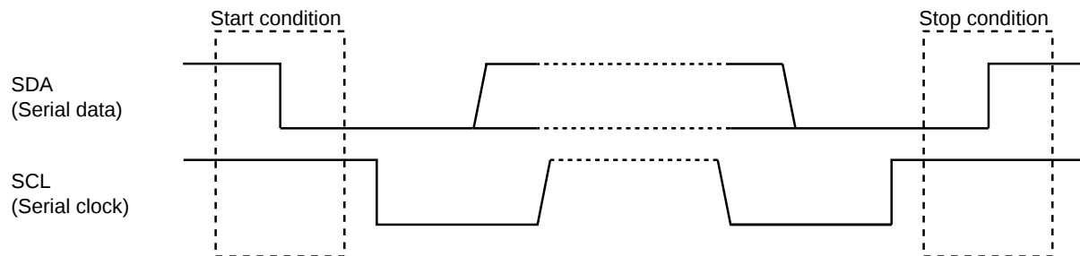
Figure 12-3-9 Start Condition and Stop Condition
