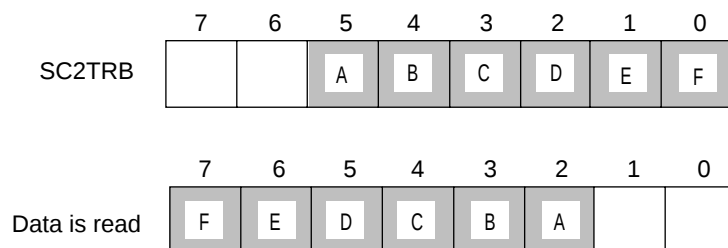
Figure 12-3-2-2 Receive Bit Count and Transfer First Bit (starting with LSB bit)
