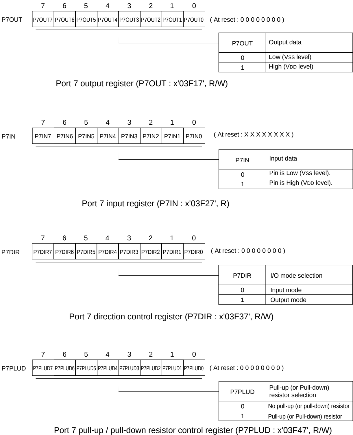
Figure 4-9-1 Port 7 Registers (1/3)
