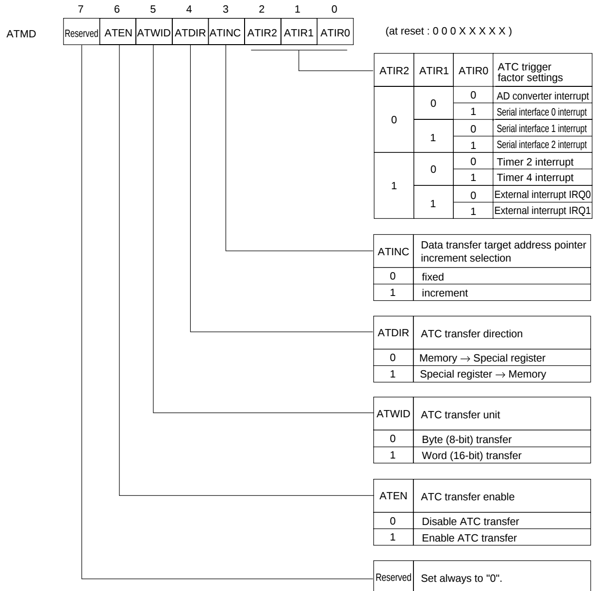
Figure 13-2-1 ATC Register (ATMD : x'03FA0', R/W)
