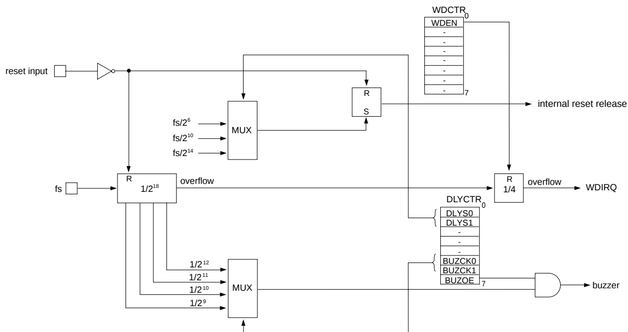
Figure 8-1-1 Block Diagram (Watchdog Timer)
