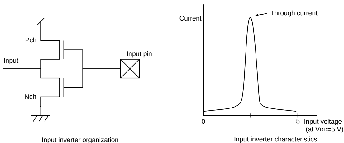
Figure 1-7-3 Input Inverter Organization and Characteristics
