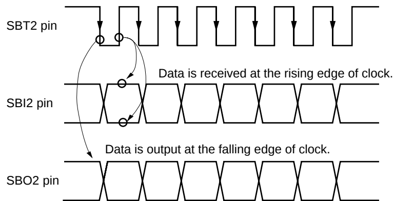
Figure 12-3-8 Transmission / Reception Timing (Reception : rising edge, Transmission : falling edge) (SC2CE0= 0)
