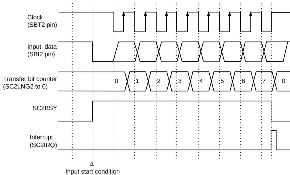
Figure 12-3-4 Reception Timing (rising edge, start condition is enabled)
