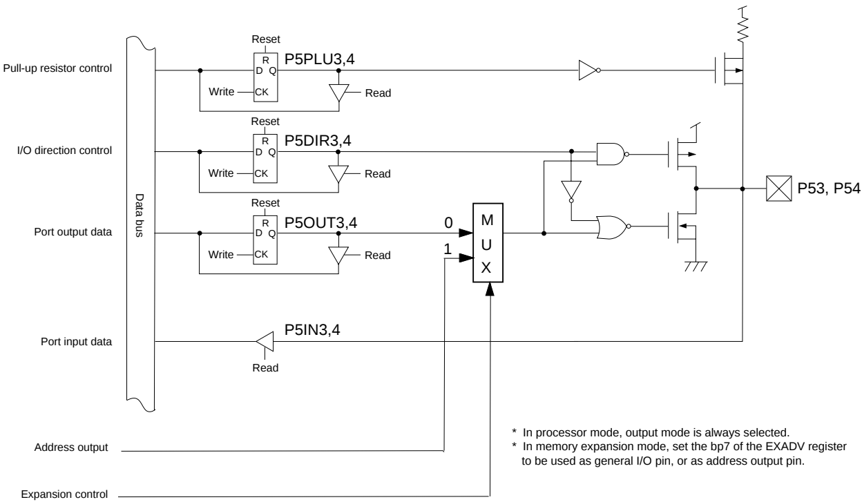
Figure 4-7-4 Block Diagram (P53, P54)
