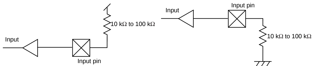
Figure 1-7-2 Unused Pins (only for input)
