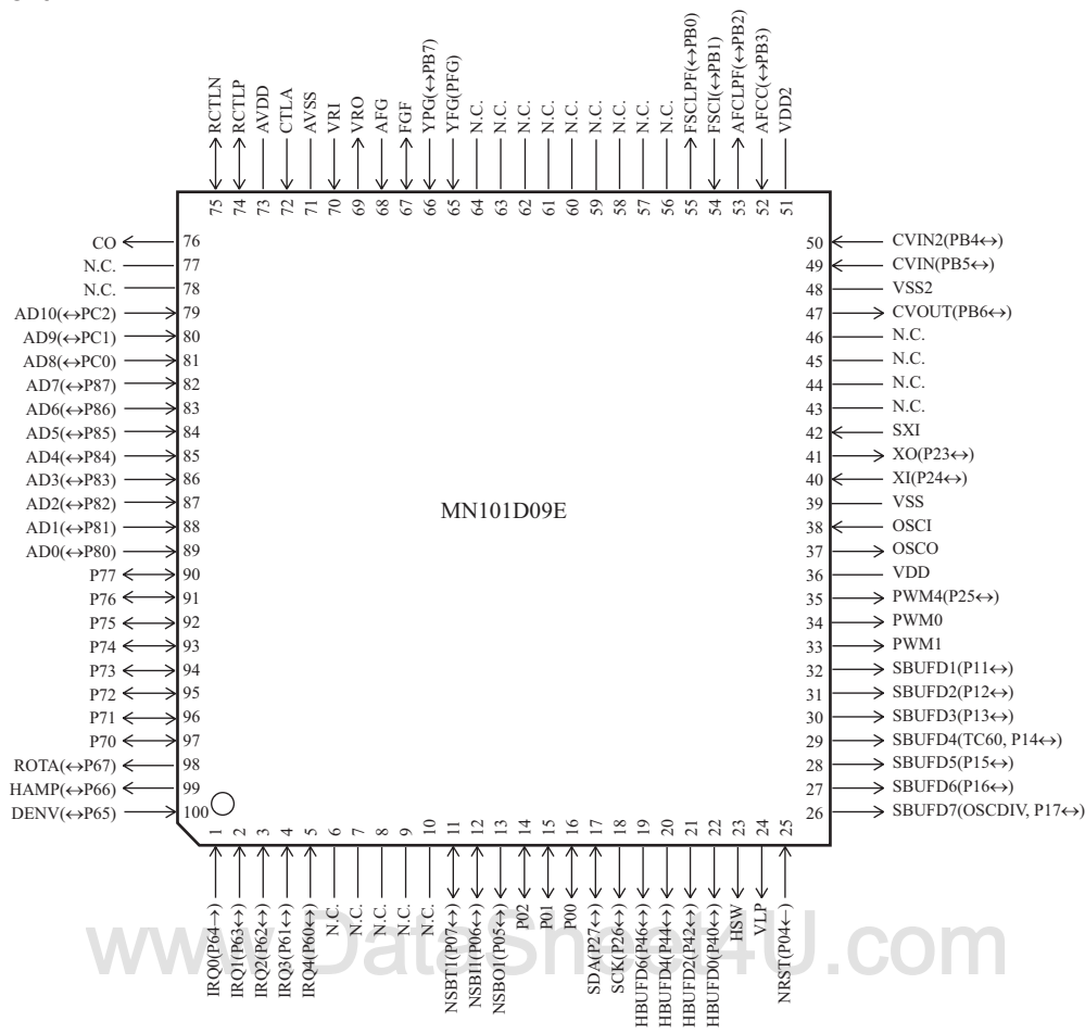
QFP100-P-1818B
