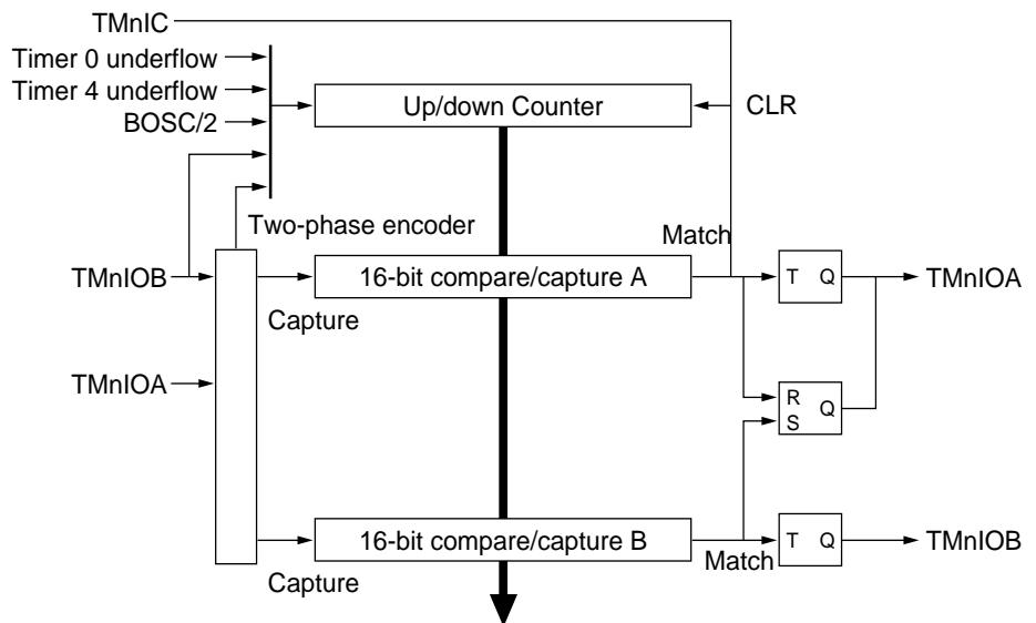
Figure 4-3-1 16-bit Timer Block Diagram
