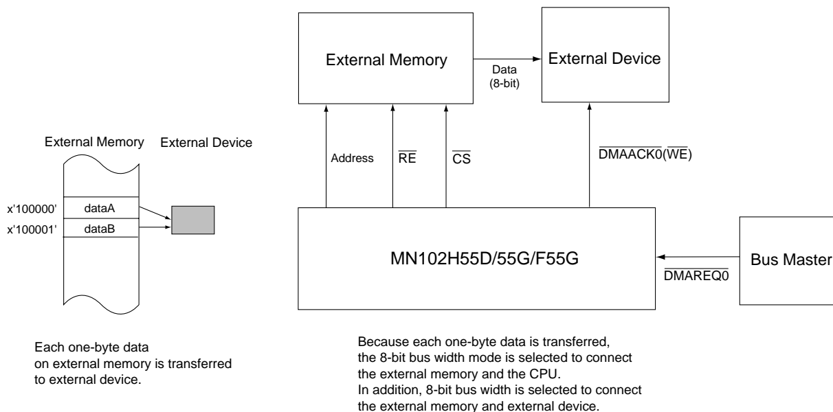
Figure 7-4-2 ETC External Memory → External Device Transfer Connection
