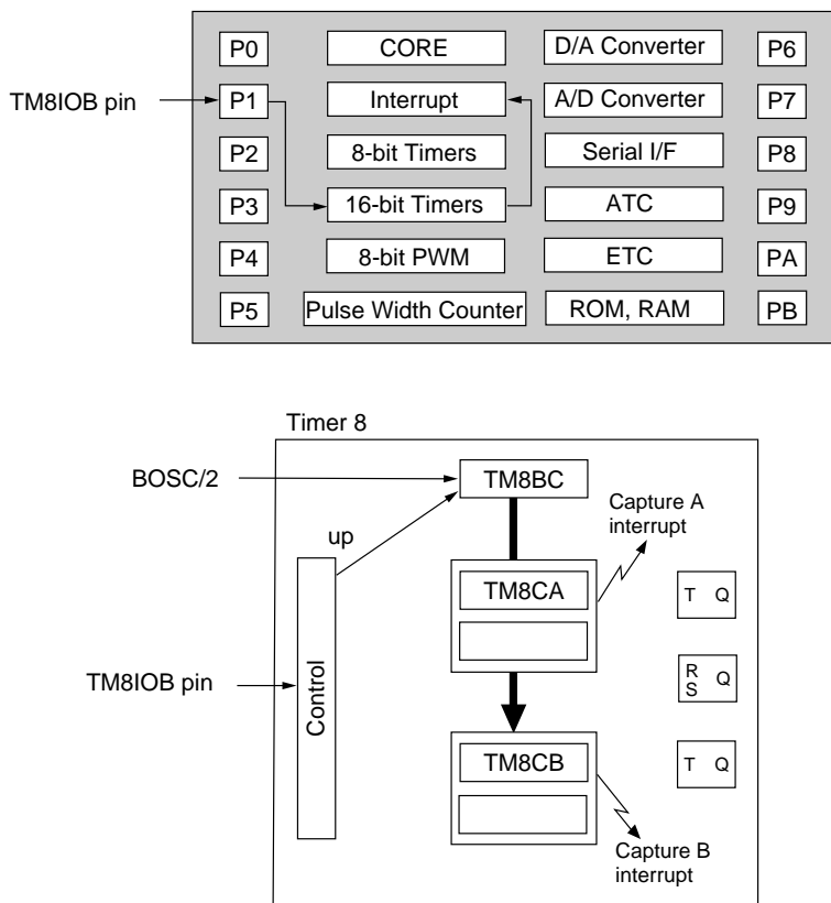
Figure 4-4-1 Event Counter Block Diagram
