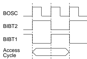
Figure 2-1-7 External Access (No Wait Cycle)
