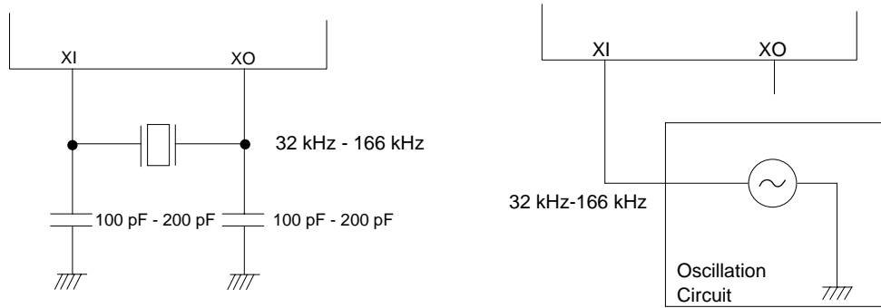
Figure 1-4-11 XI, XO Connection Example
