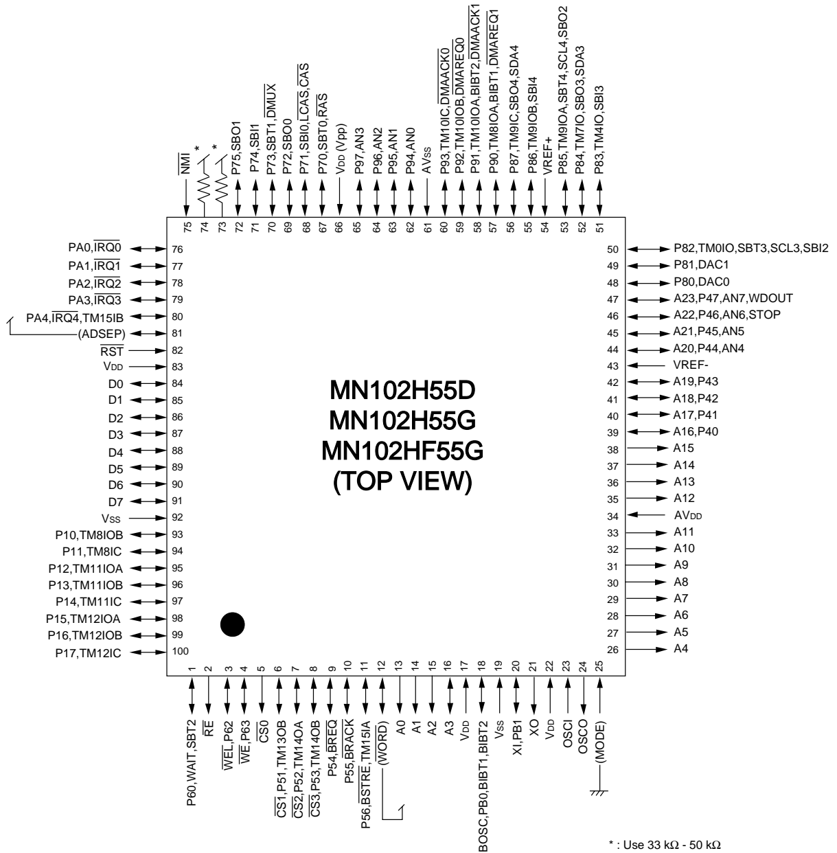
Figure 1-4-6 Pin Configuration in Processor Mode with 8-bit Bus Address/Data Separate Mode
