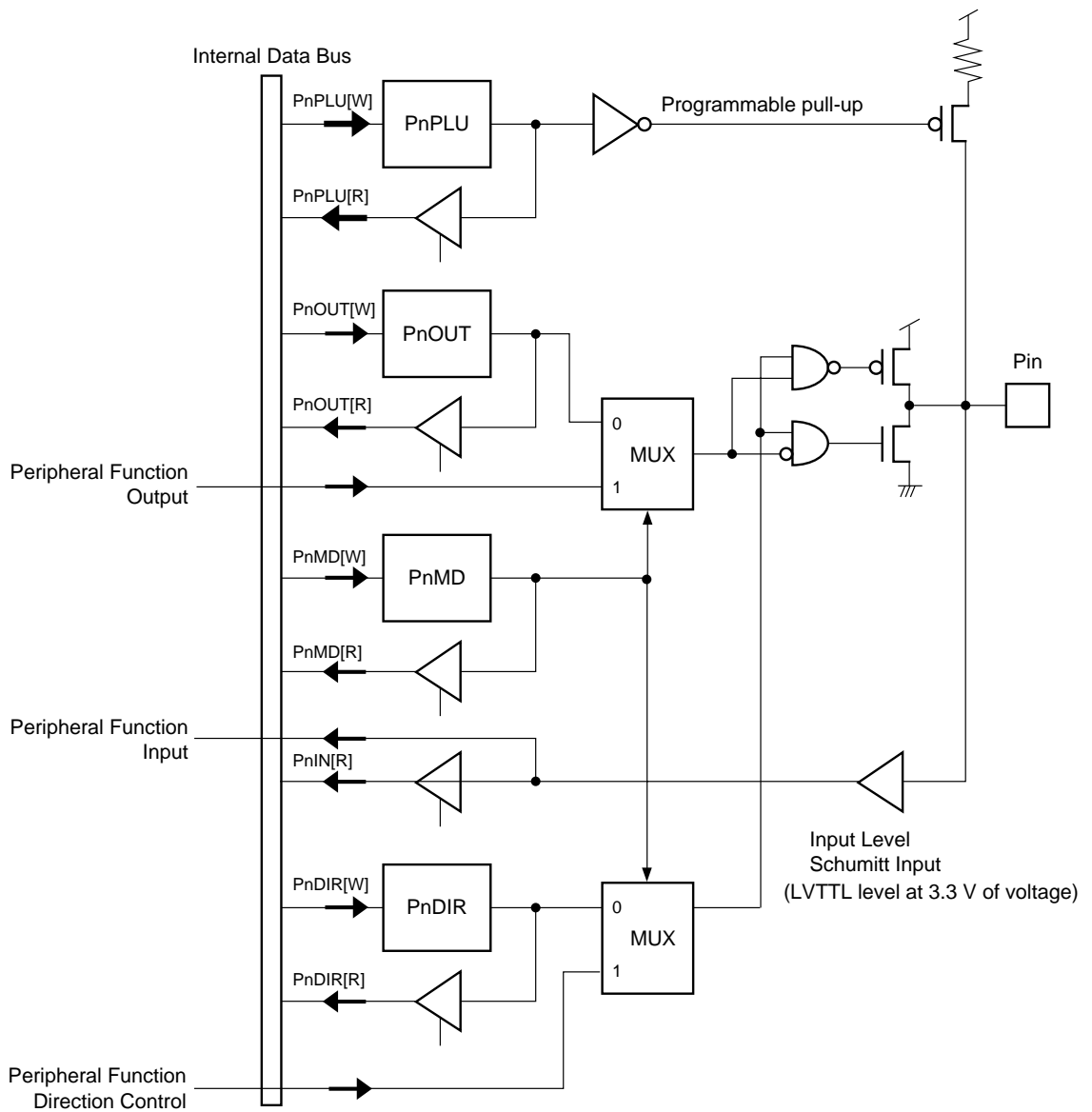
Figure 8-1-1 I/O Port Configuration
