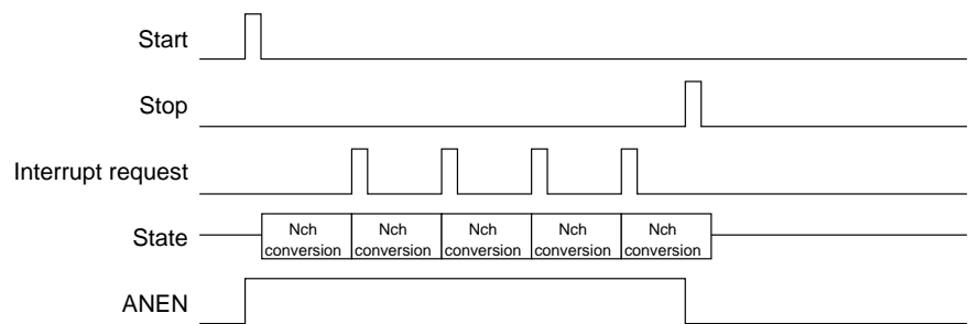
Figure 6-1-5 Single Channel/Continuous Conversion Timing
