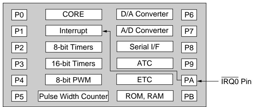
Figure 3-2-1 External Pin Interrupt Block Diagram
