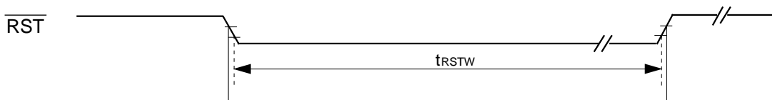
Figure 11-1-2 Reset Timing
