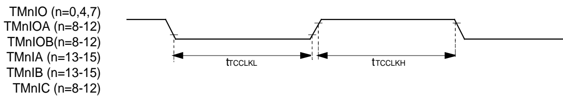
Figure 11-1-18 Timer/Counter Signal Timing
