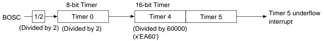
Figure 4-2-6 Interval Timer Configuration Example (8-bit Timer)
