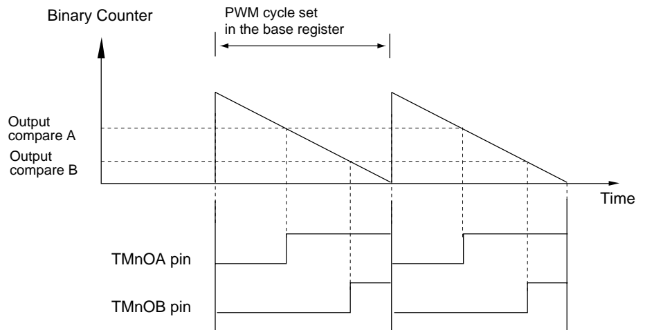
Figure 4-5-2 PWM Output Waveform
