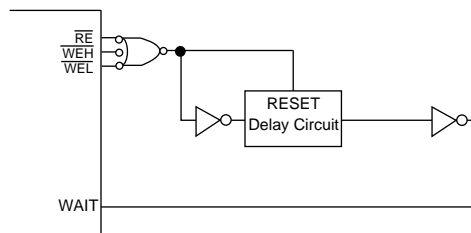
Figure 1-4-13 WAIT Signal Control Circuit Connection Example
