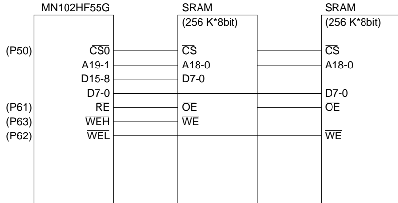
Figure 2-1-2 SRAM (Mask ROM) Connection Example (16-bit Bus Width)
