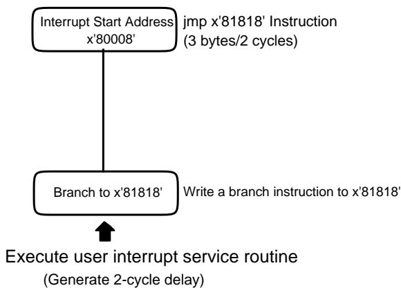
Figure 11-4-11 Interrupt Service Routine Flow
