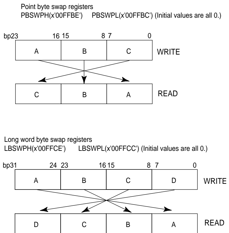
Figure 8-3-1 Byte-swapped Register
