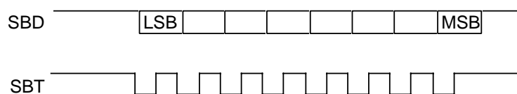
Figure 11-4-12 Data Transfer Timing
