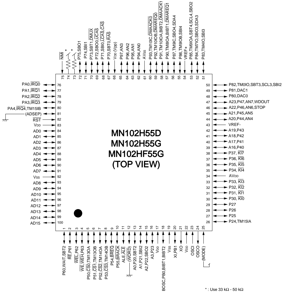
Figure 1-4-5 Pin Configuration in Memory Expansion Mode with 16-bit Bus Address/Data Shared Mode
