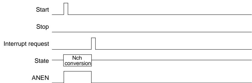
Figure 6-1-3 Single Channel/Single Conversion Timing
