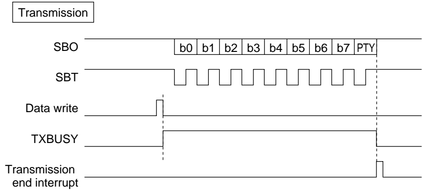
Figure 5-1-7 Synchronous Serial Timing (Transmission)
