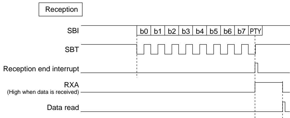
Figure 5-1-8 Synchronous Serial Timing (Reception)
