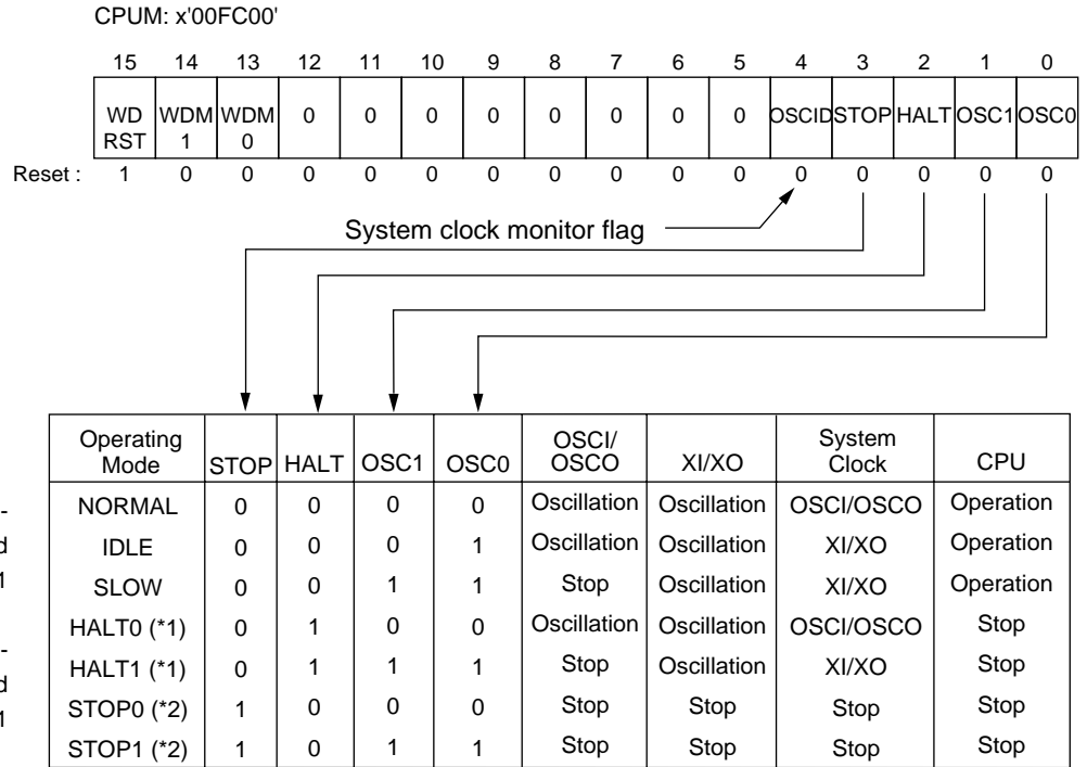
Figure 10-1-2 Operating Mode Control and Clock Oscillation On/Off
