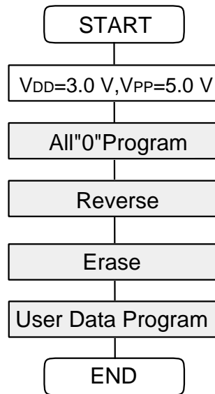
Figure 11-4-13 Programming Flow
