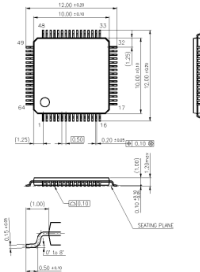
Figure:1.7.6 Package Dimension of TQFP064-P-1010D
