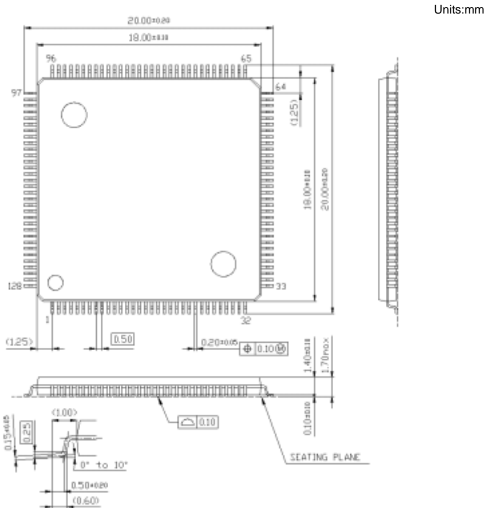
Figure:1.7.2 Package Dimension of LQFP128-P-1818F
