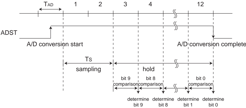
Figure 6-3-1 Timing of A/D Conversion ( T_s = T_{AD} \times 2 )
