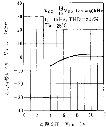
V_{i(max)} - V_{DD}
