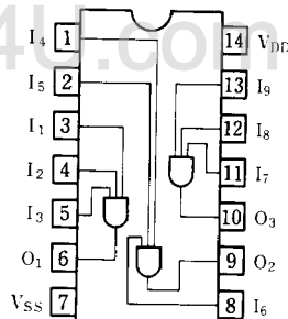
Pin Configuration
