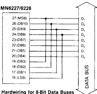
Hardwiring for 8-Bit Data Buses
