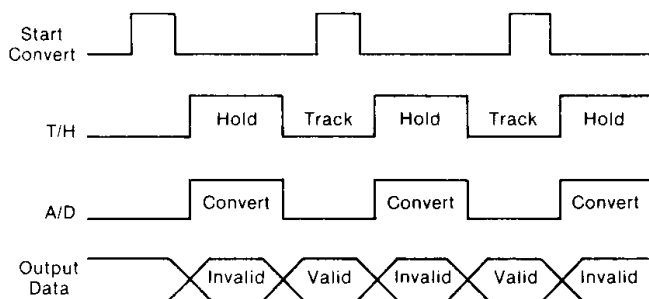
MN6227/6228 TIMING
