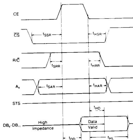
Read Cycle Timing
