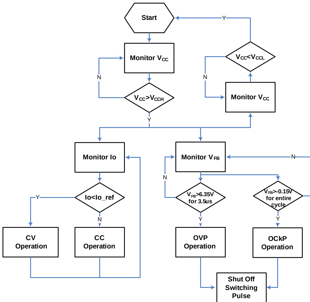
Figure 17: Flow Chart
